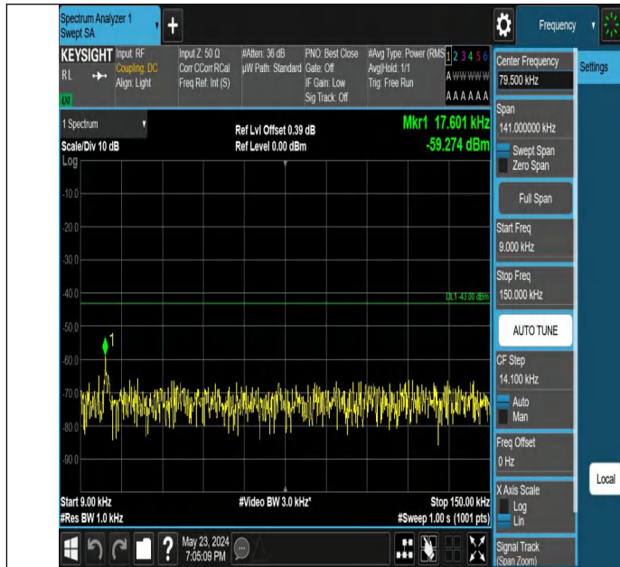
Band66_3MHz_QPSK_132322_1RB#0_0.009~0.15_0.009~0.15
