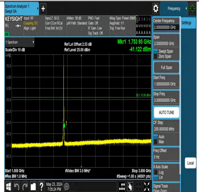
Band66_3MHz_QPSK_132322_1RB#0_1000~3000_1000~3000
