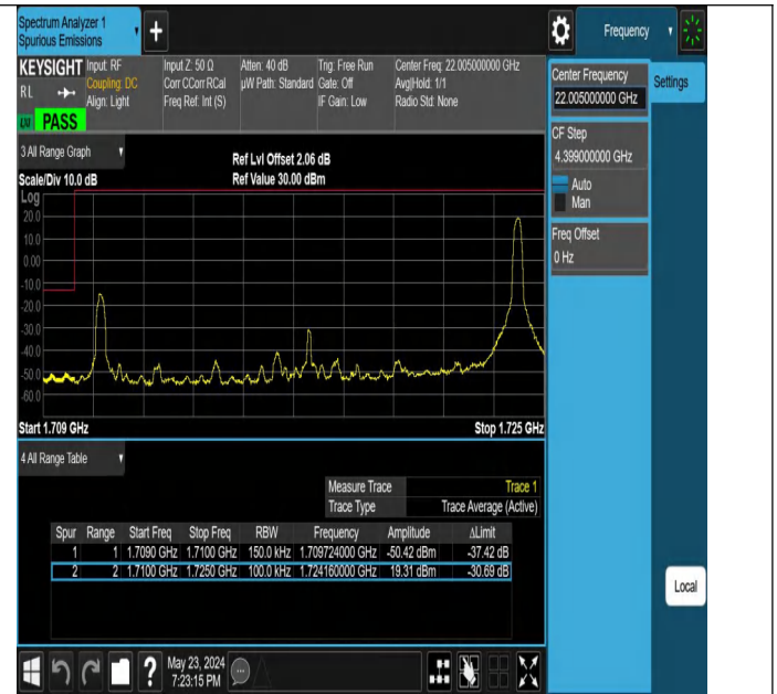
Band66_15MHz_QPSK_132047_1RB#74
