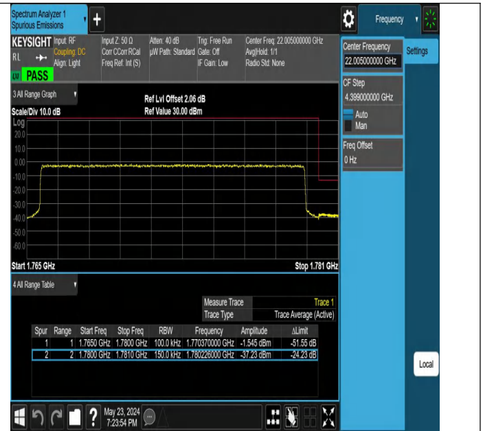
Band66_15MHz_QPSK_132597_75RB#0
