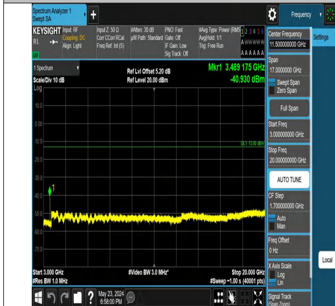
Band66_1.4MHz_QPSK_132322_1RB#0_3000~20000_3000~2000
