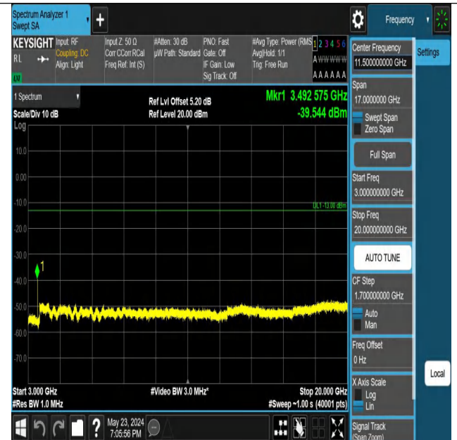
Band66_3MHz_QPSK_132322_1RB#14_3000~20000_3000~2000
