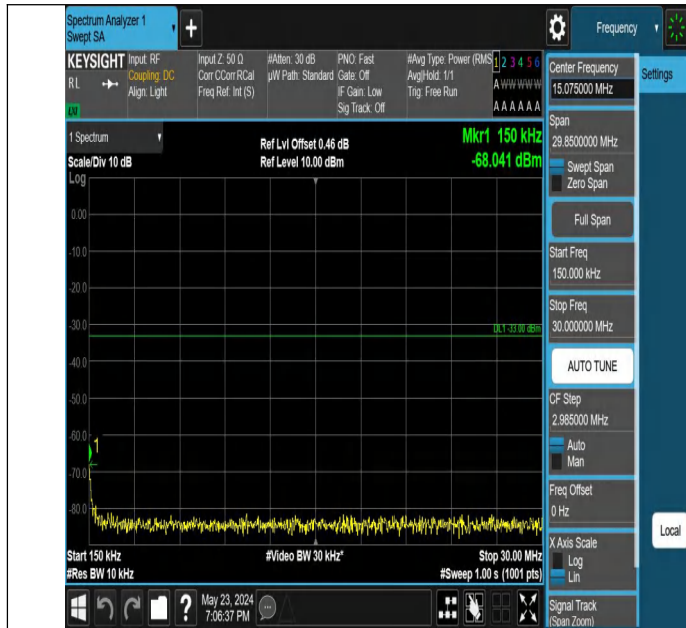
Band66_3MHz_QPSK_132657_1RB#14_0.15~30_0.15~30
