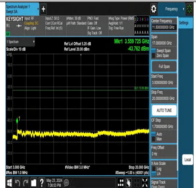
Band66_3MHz_QPSK_132657_1RB#14_3000~20000_3000~2000
