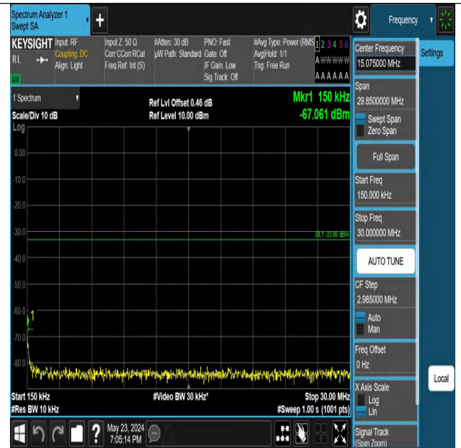
Band66_3MHz_QPSK_132322_1RB#0_0.15~30_0.15~30
