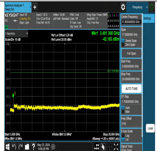
Band66_1.4MHz_QPSK_132322_1RB#5_3000~20000_3000~200
