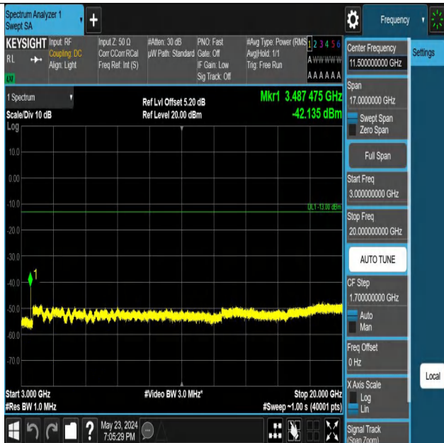
Band66_3MHz_QPSK_132322_1RB#0_3000~20000_3000~2000
