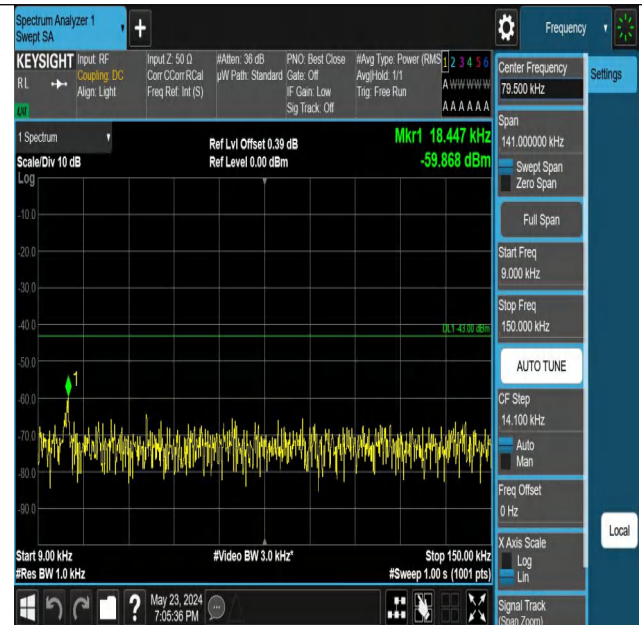
Band66_3MHz_QPSK_132322_1RB#14_0.009~0.15_0.009~0.15
