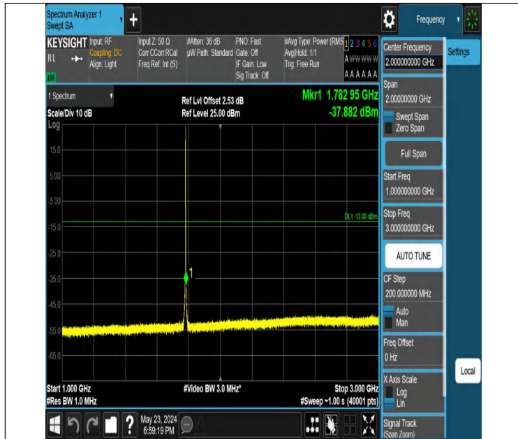
Band66_1.4MHz_QPSK_132665_1RB#5_1000~3000_1000~3000
