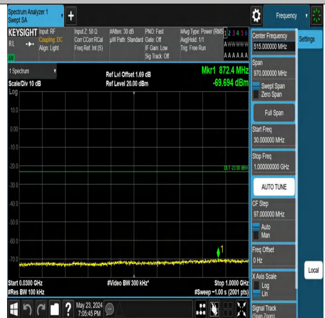
Band66 3MHz QPSK 132322 1RB#14 30~1000 30~1000
