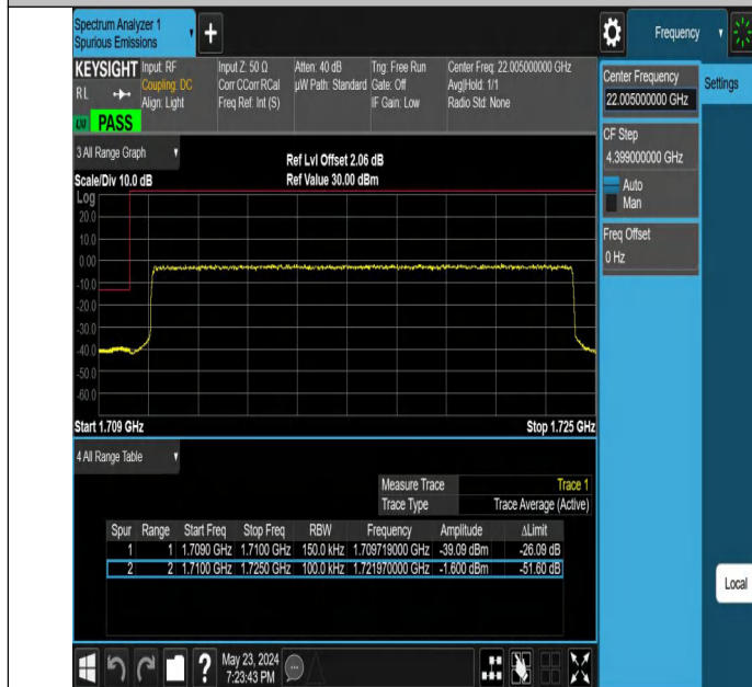
Band66_15MHz_QPSK_132047_75RB#0
