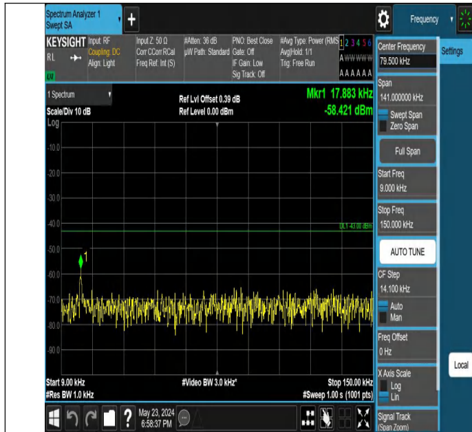
Band66_1.4MHz_QPSK_132665_1RB#0_0.009~0.15_0.009~0.15
