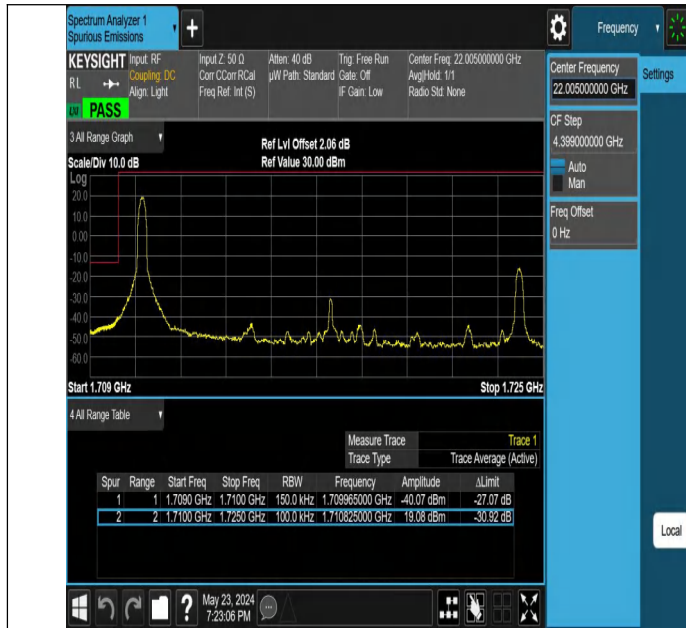
Band66_15MHz_QPSK_132047_1RB#0
