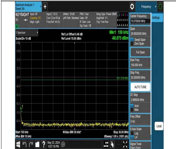
Band66_1.4MHz_QPSK_131979_1RB#5_0.15~30_0.15~30
