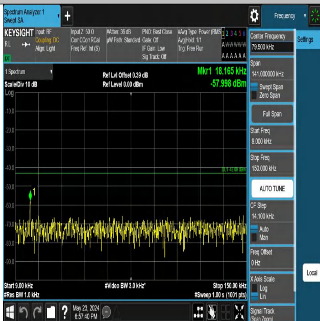
Band66 1.4MHz QPSK 132322 1RB#0 0.009~0.15 0.009~0.15
