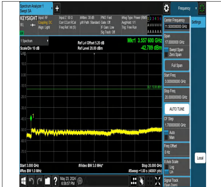
Band66_1.4MHz_QPSK_132665_1RB#0_3000~20000_3000~20000
