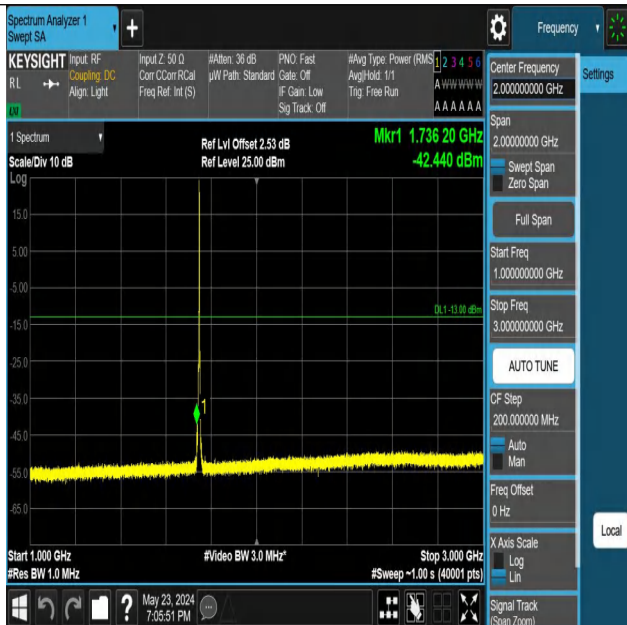
Band66_3MHz_QPSK_132322_1RB#14_1000~3000_1000~3000
