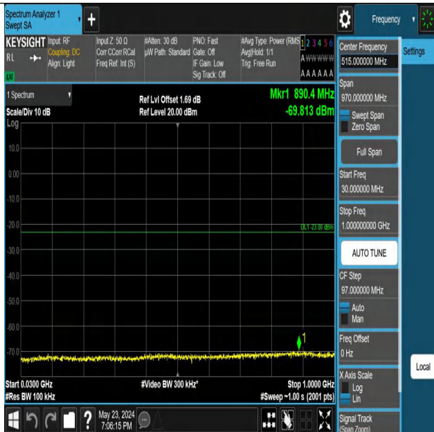
Band66_3MHz_QPSK_132657_1RB#0_30~1000_30~1000
