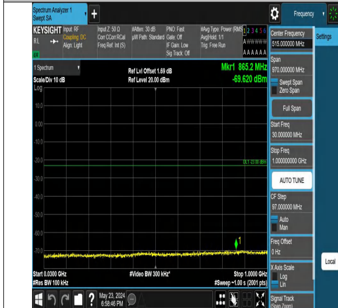
Band66_1.4MHz_QPSK_132665_1RB#0_30~1000_30~1000
