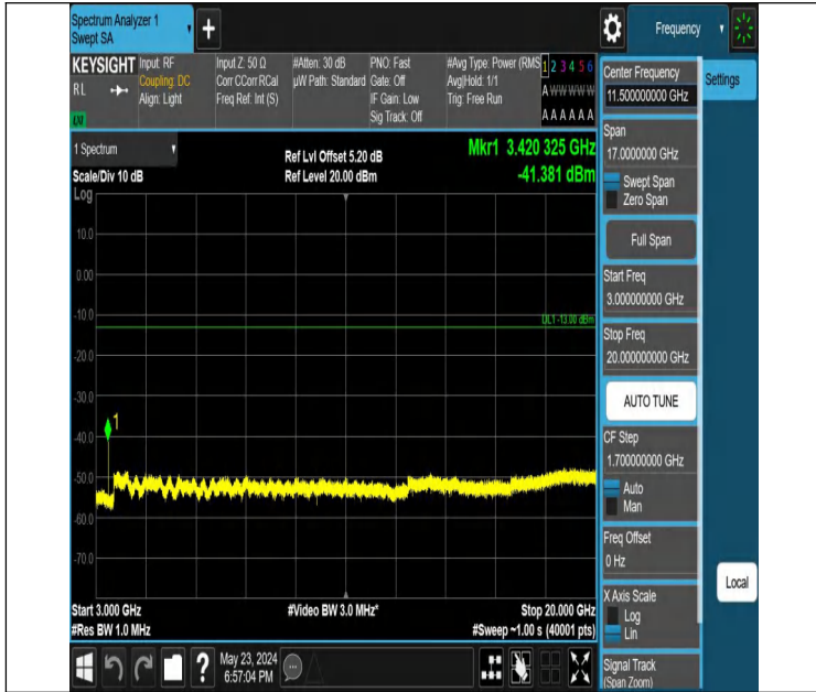
Band66_1.4MHz_QPSK_131979_1RB#0_3000~20000_3000~20000
