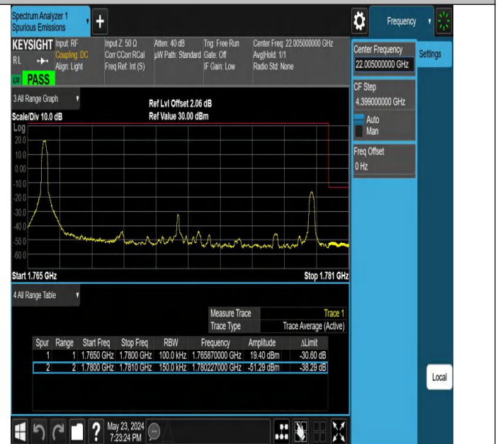
Band66_15MHz_QPSK_132597_1RB#0
