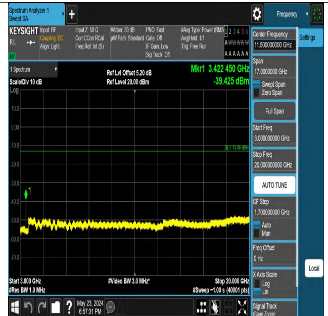
Band66_1.4MHz_QPSK_131979_1RB#5_3000~20000_3000~20000
