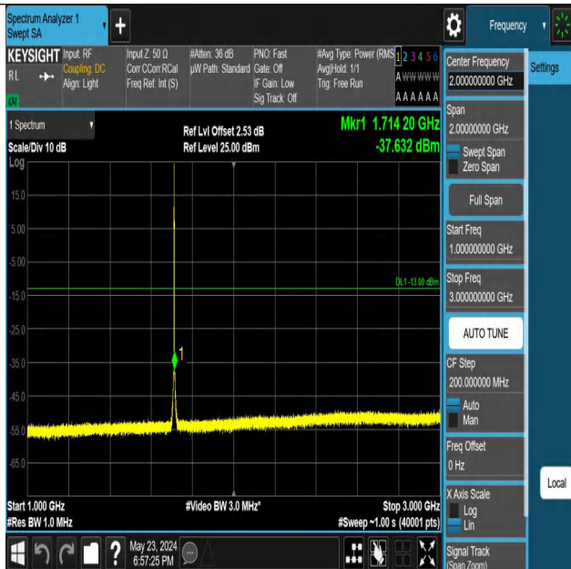
Band66_1.4MHz_QPSK_131979_1RB#5_1000~3000_1000~3000
