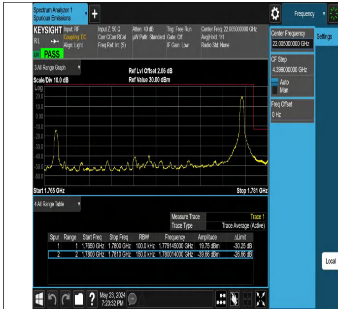
Band66_15MHz_QPSK_132597_1RB#74
