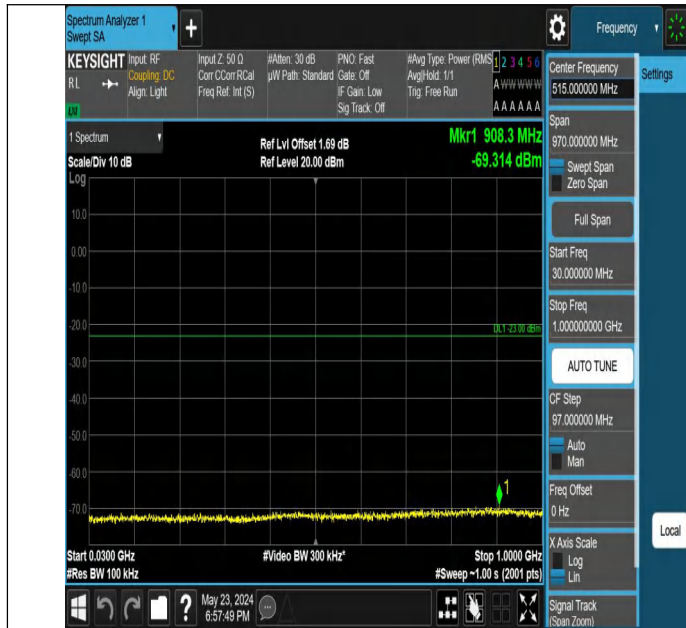
Band66_1.4MHz_QPSK_132322_1RB#0_30~1000_30~1000
