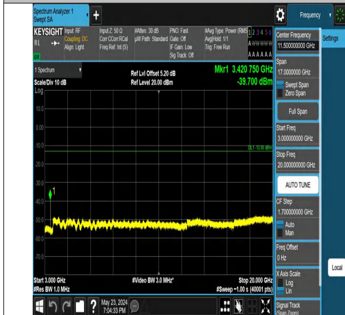
Band66_3MHz_QPSK_131987_1RB#0_3000~20000_3000~2000
