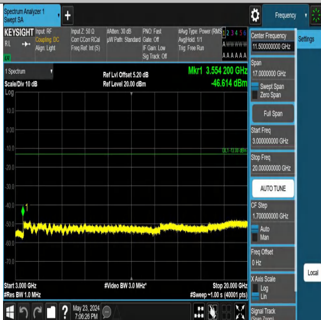
Band66_3MHz_QPSK_132657_1RB#0_3000~20000_3000~2000
