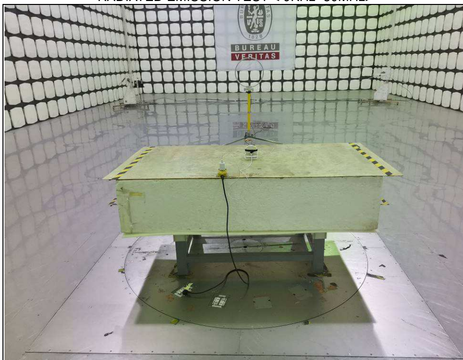
RADIATED EMISSION TEST < 9KHz~30MHz>
