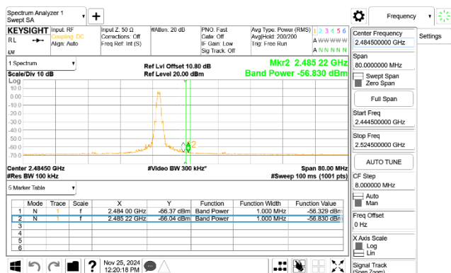
CBE_BLE_125k_2480MHz
