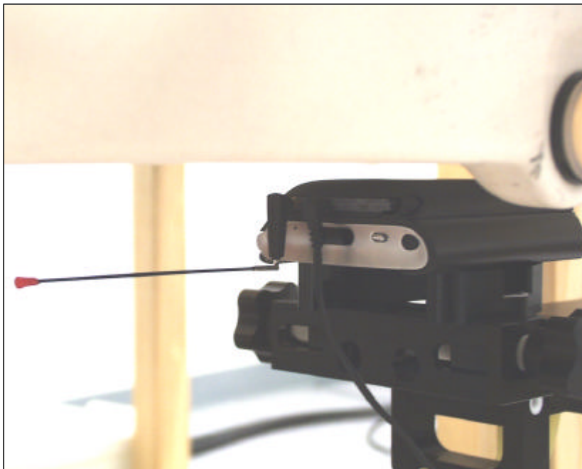
EUT Set-up configuration 2
