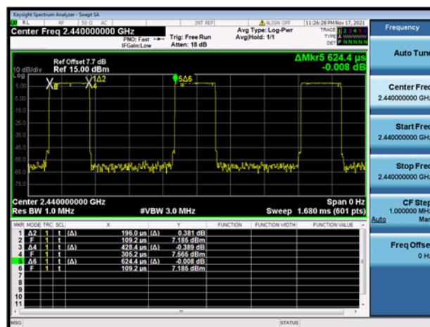
GFSK(BLE 2Mbps)
