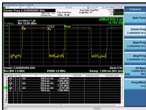
GFSK(BLE 1Mbps)
