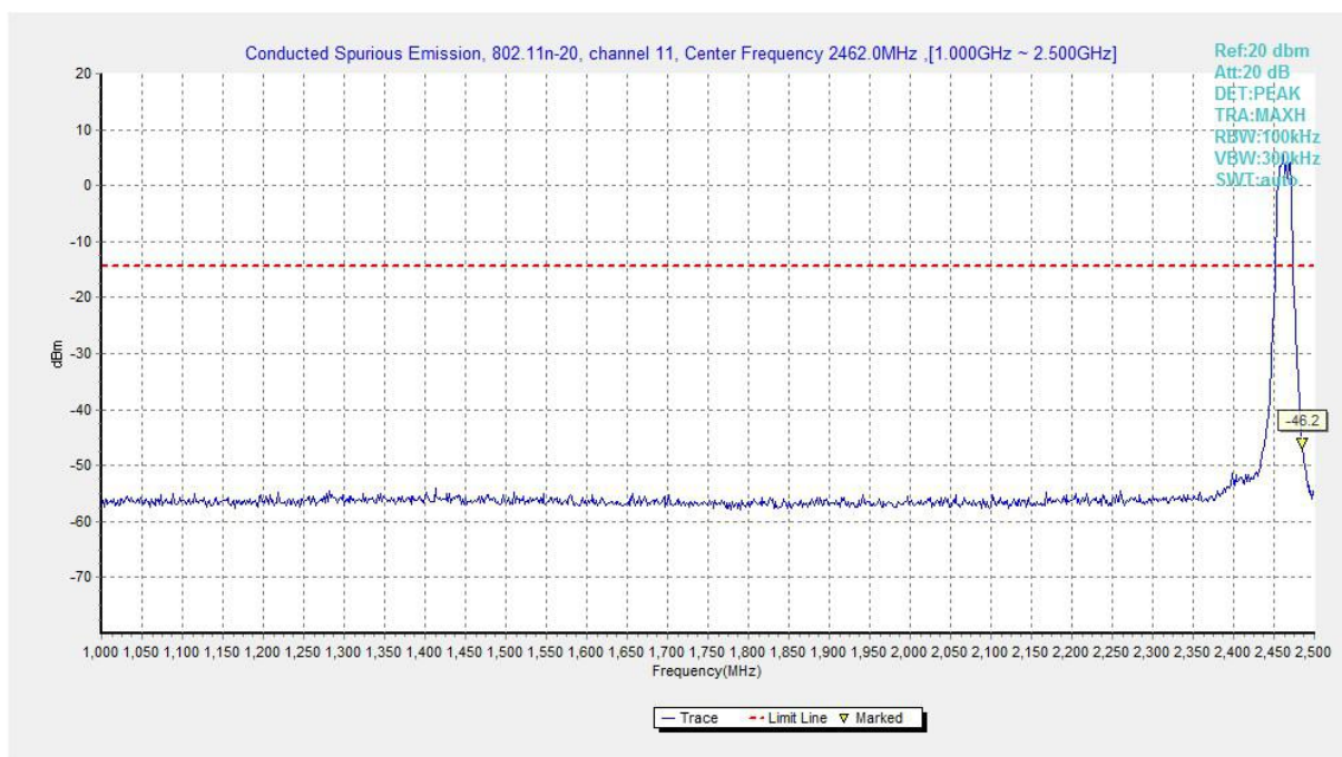
Fig.A.6.1.19 Transmitter Spurious Emission - Conducted (802.11n-HT20, Ch11, 1 GHz-2.5 GHz)
