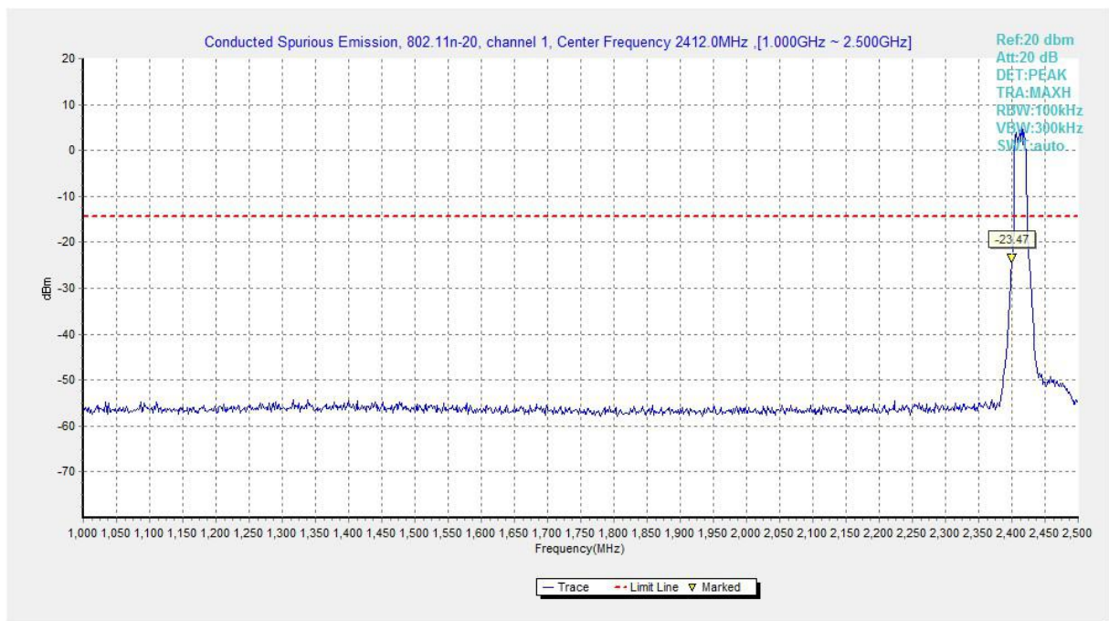
Fig.A.6.1.3 Transmitter Spurious Emission - Conducted (802.11n-HT20, Ch1, 1 GHz-2.5 GHz)
