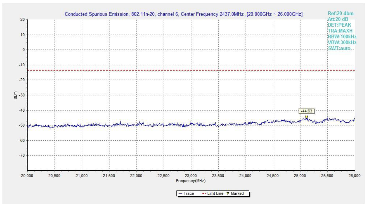
Fig.A.6.1.16 Transmitter Spurious Emission - Conducted (802.11n-HT20, Ch6, 20 GHz-26 GHz)
