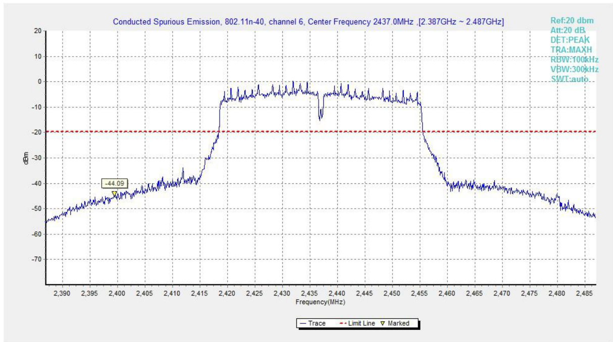
Fig.A.6.1.33 Transmitter Spurious Emission - Conducted (802.11n-HT40, Ch6, Center Frequency)
