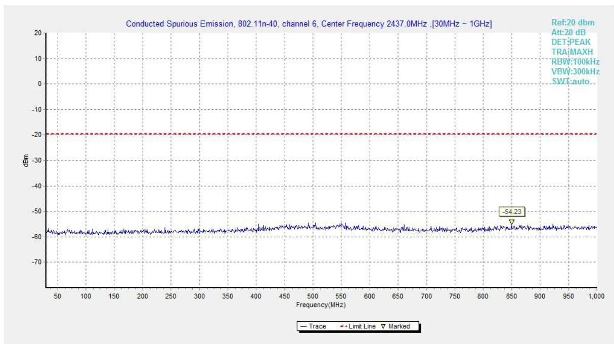
Fig.A.6.1.34 Transmitter Spurious Emission - Conducted (802.11n-HT40, Ch6, 30 MHz-1 GHz)
