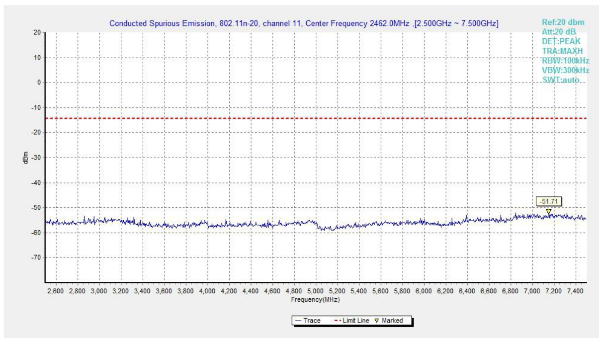
Fig.A.6.1.20 Transmitter Spurious Emission - Conducted (802.11n-HT20, Ch11, 2.5 GHz-7.5 GHz)
