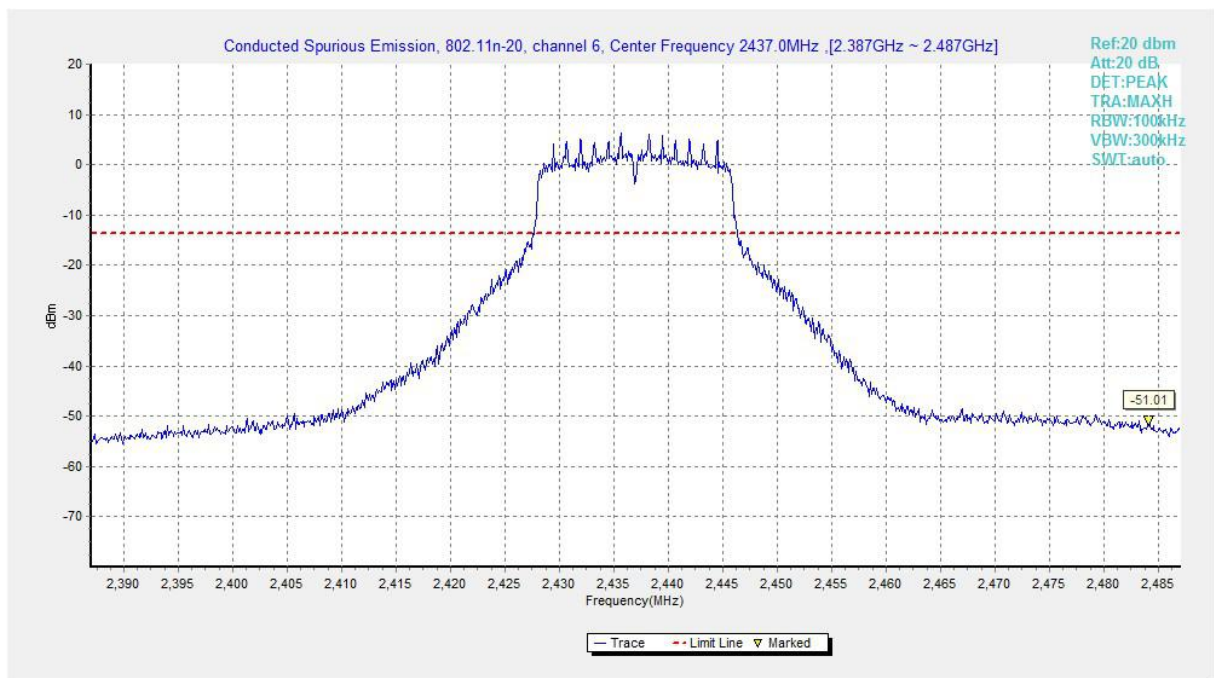
Fig.A.6.1.9 Transmitter Spurious Emission - Conducted (802.11n-HT20, Ch6, Center Frequency)
