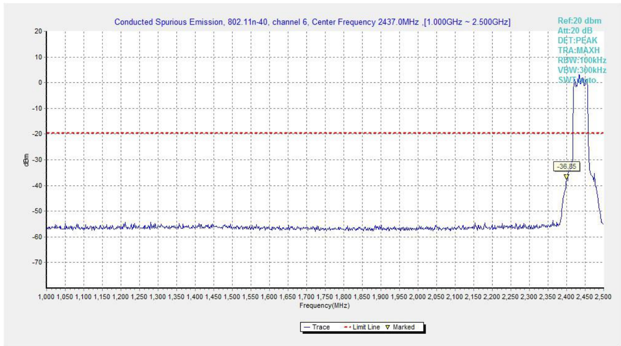
Fig.A.6.1.35 Transmitter Spurious Emission - Conducted (802.11n-HT40, Ch6, 1 GHz-2.5 GHz)
