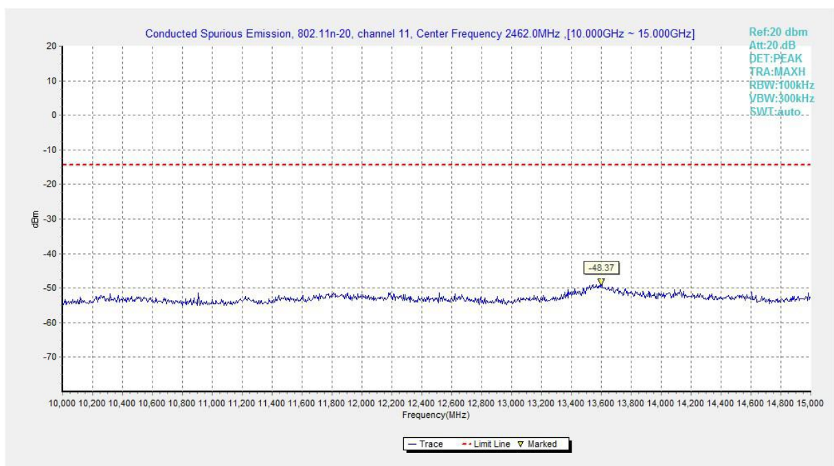
Fig.A.6.1.22 Transmitter Spurious Emission - Conducted (802.11n-HT20, Ch11, 10 GHz-15 GHz)
