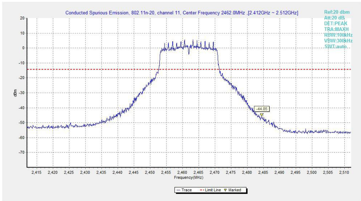
Fig.A.6.1.17 Transmitter Spurious Emission - Conducted (802.11n-HT20, Ch11, Center Frequency)
