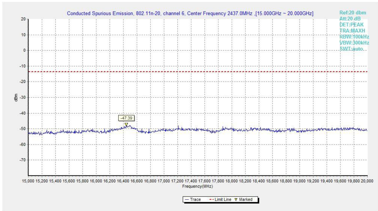
Fig.A.6.1.15 Transmitter Spurious Emission - Conducted (802.11n-HT20, Ch6, 15 GHz-20 GHz)
