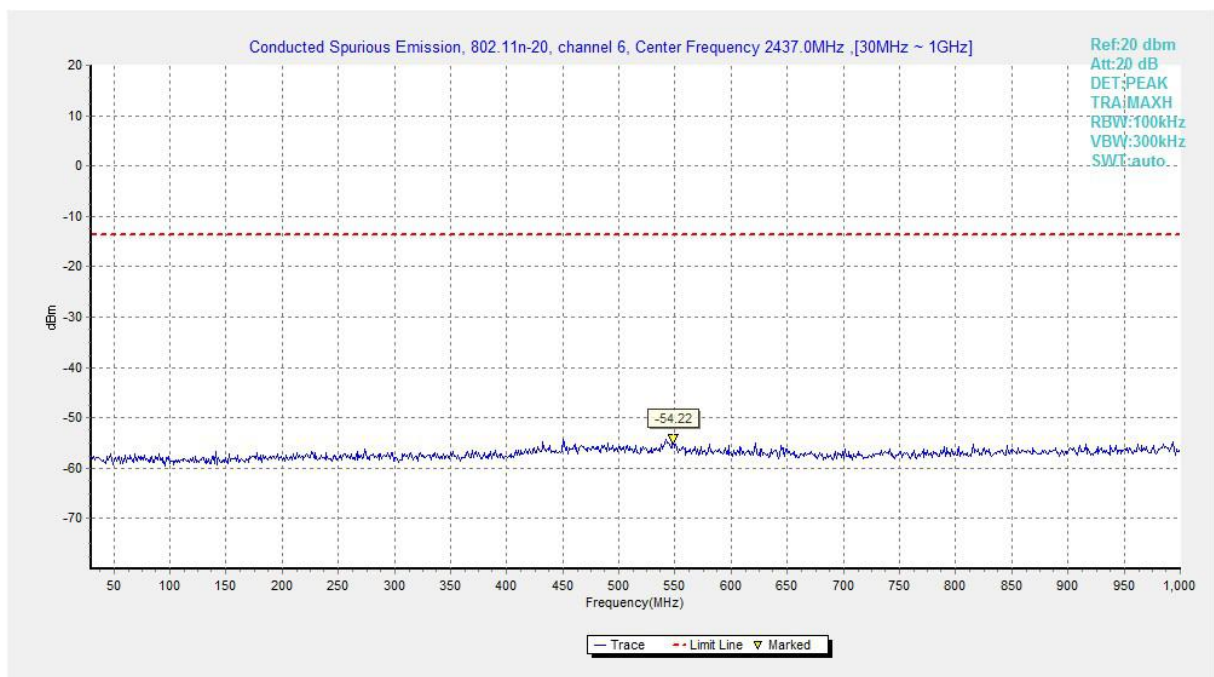
Fig.A.6.1.10 Transmitter Spurious Emission - Conducted (802.11n-HT20, Ch6, 30 MHz-1 GHz)
