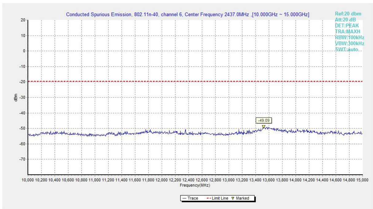
Fig.A.6.1.38 Transmitter Spurious Emission - Conducted (802.11n-HT40, Ch6, 10 GHz-15 GHz)
