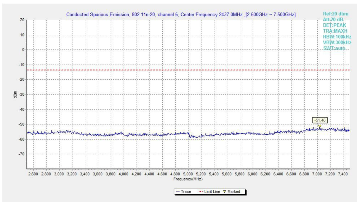
Fig.A.6.1.12 Transmitter Spurious Emission - Conducted (802.11n-HT20, Ch6, 2.5 GHz-7.5 GHz)
