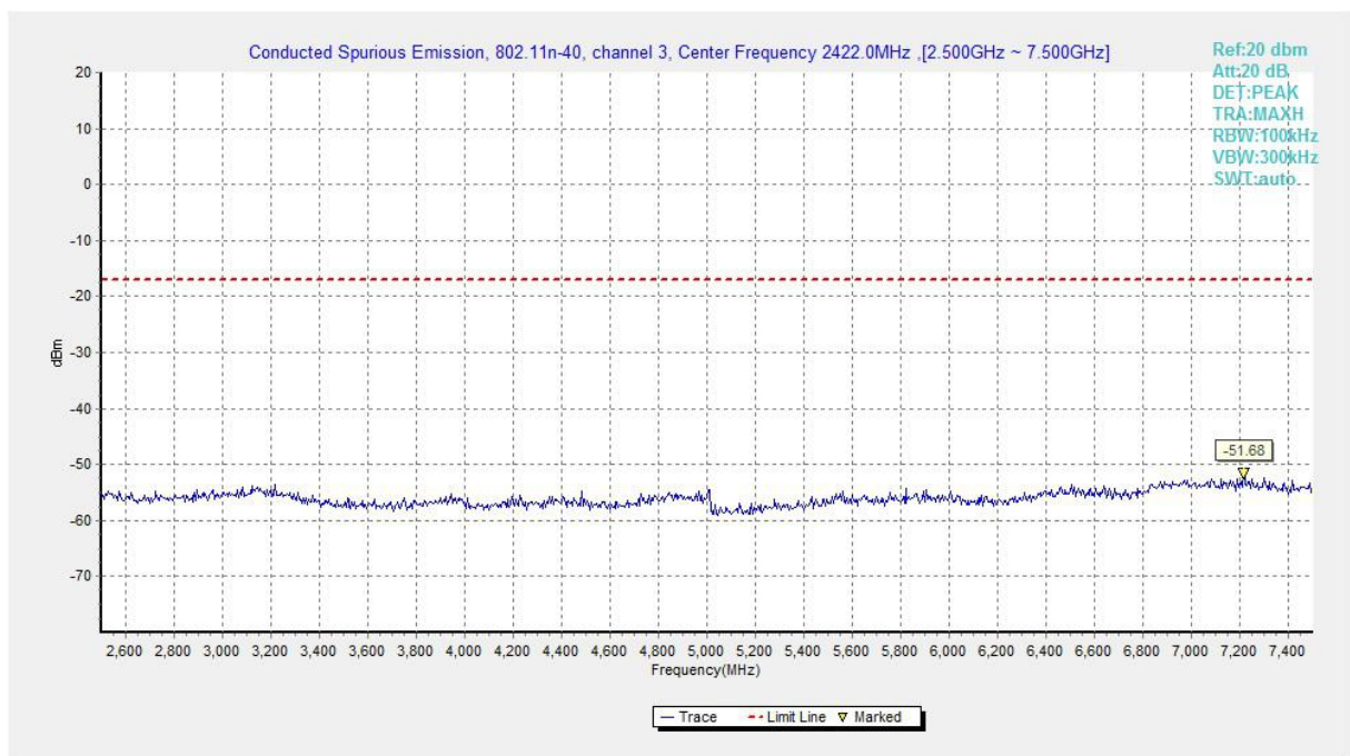
Fig.A.6.1.28 Transmitter Spurious Emission - Conducted (802.11n-HT40, Ch3, 2.5 GHz-7.5 GHz)
