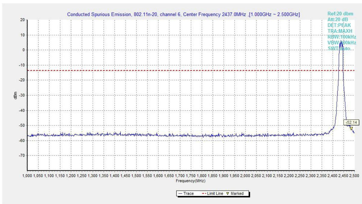
Fig.A.6.1.11 Transmitter Spurious Emission - Conducted (802.11n-HT20, Ch6, 1 GHz-2.5 GHz)
