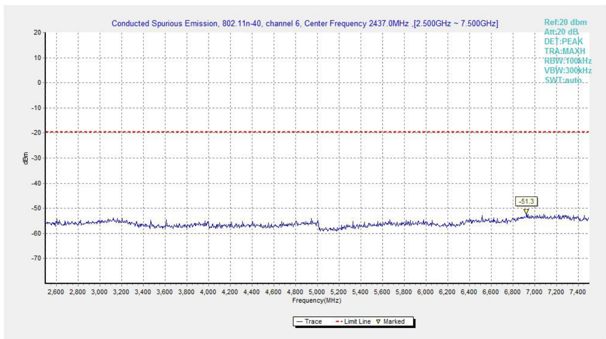
Fig.A.6.1.36 Transmitter Spurious Emission - Conducted (802.11n-HT40, Ch6, 2.5 GHz-7.5 GHz)
