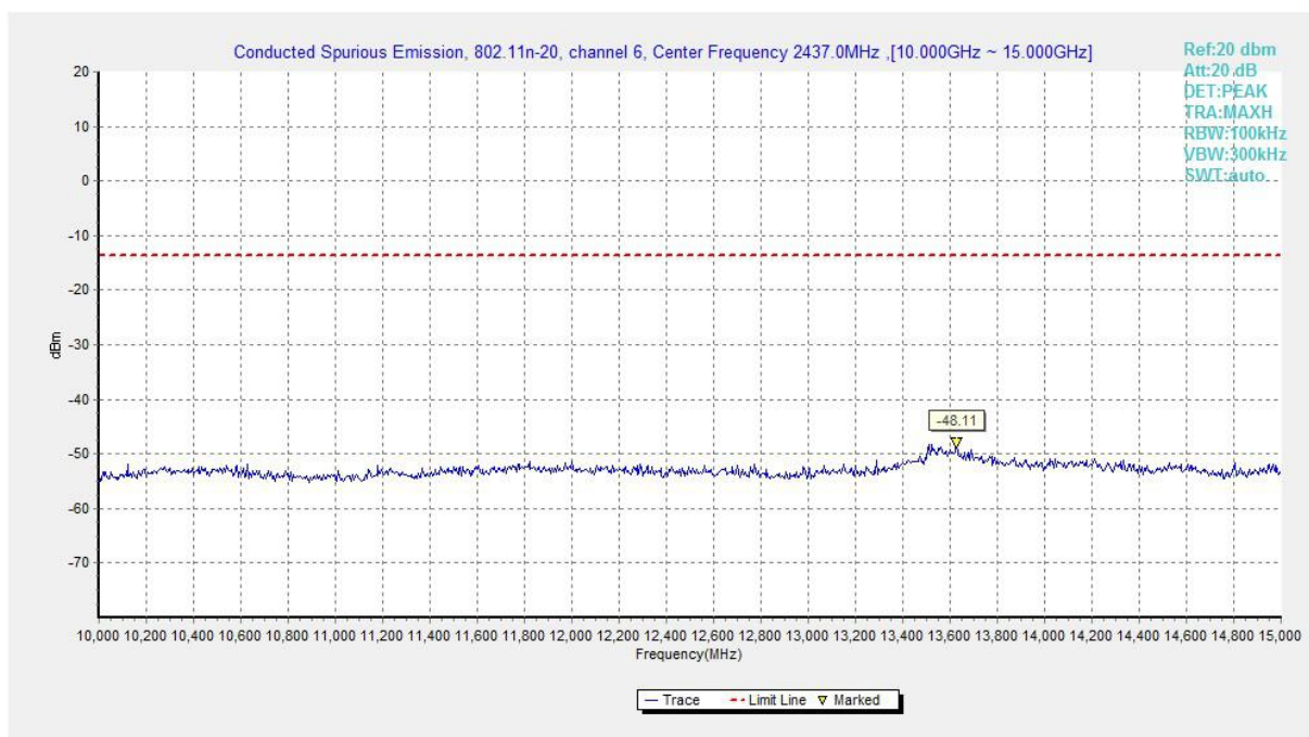
Fig.A.6.1.14 Transmitter Spurious Emission - Conducted (802.11n-HT20, Ch6, 10 GHz-15 GHz)
