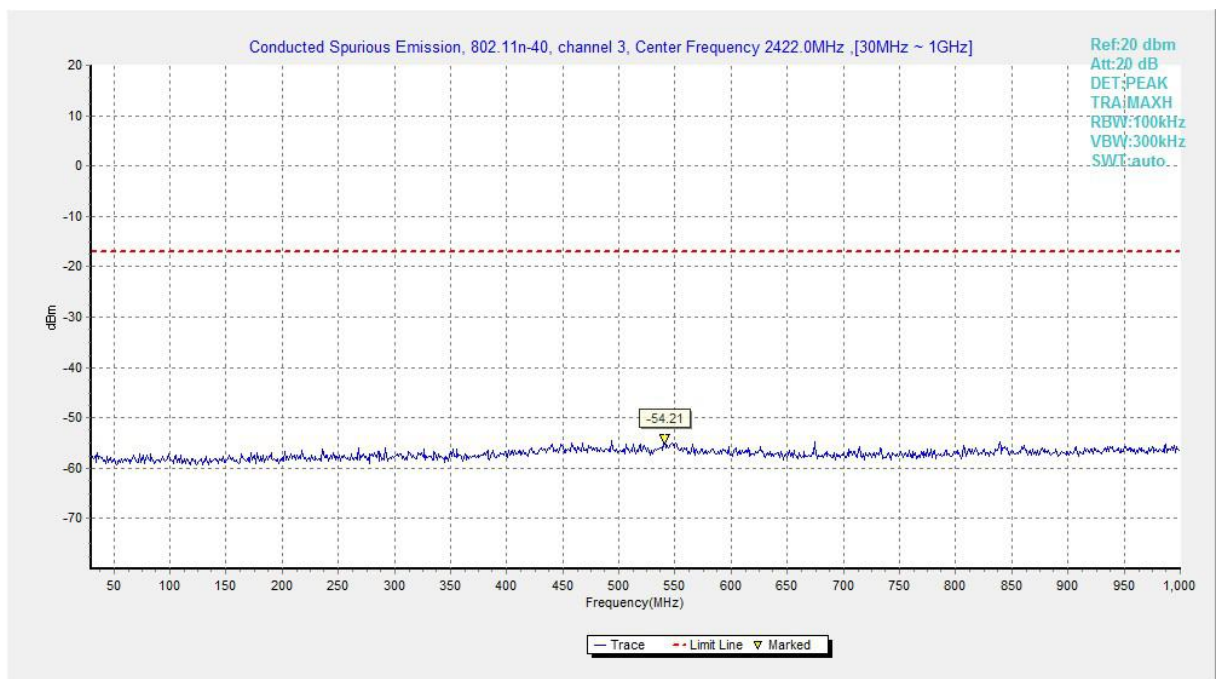
Fig.A.6.1.26 Transmitter Spurious Emission - Conducted (802.11n-HT40, Ch3, 30 MHz-1 GHz)
