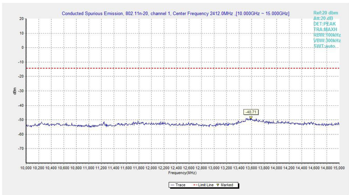
Fig.A.6.1.6 Transmitter Spurious Emission - Conducted (802.11n-HT20, Ch1, 10 GHz-15 GHz)
