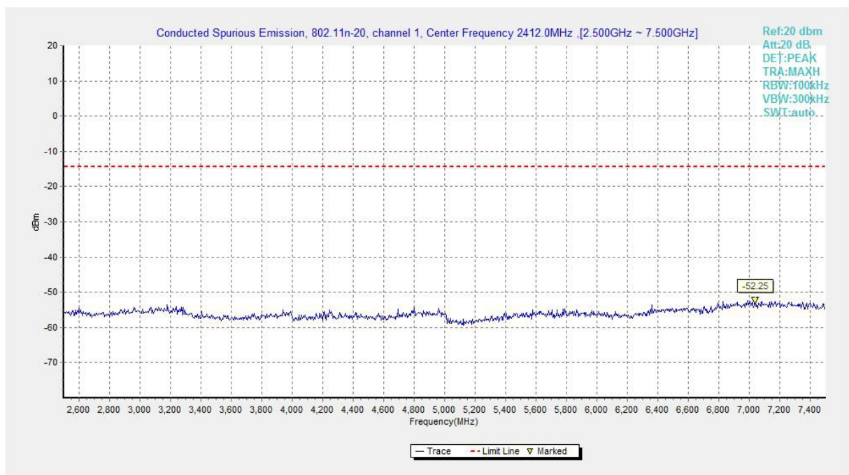
Fig.A.6.1.4 Transmitter Spurious Emission - Conducted (802.11n-HT20, Ch1, 2.5 GHz-7.5 GHz)
