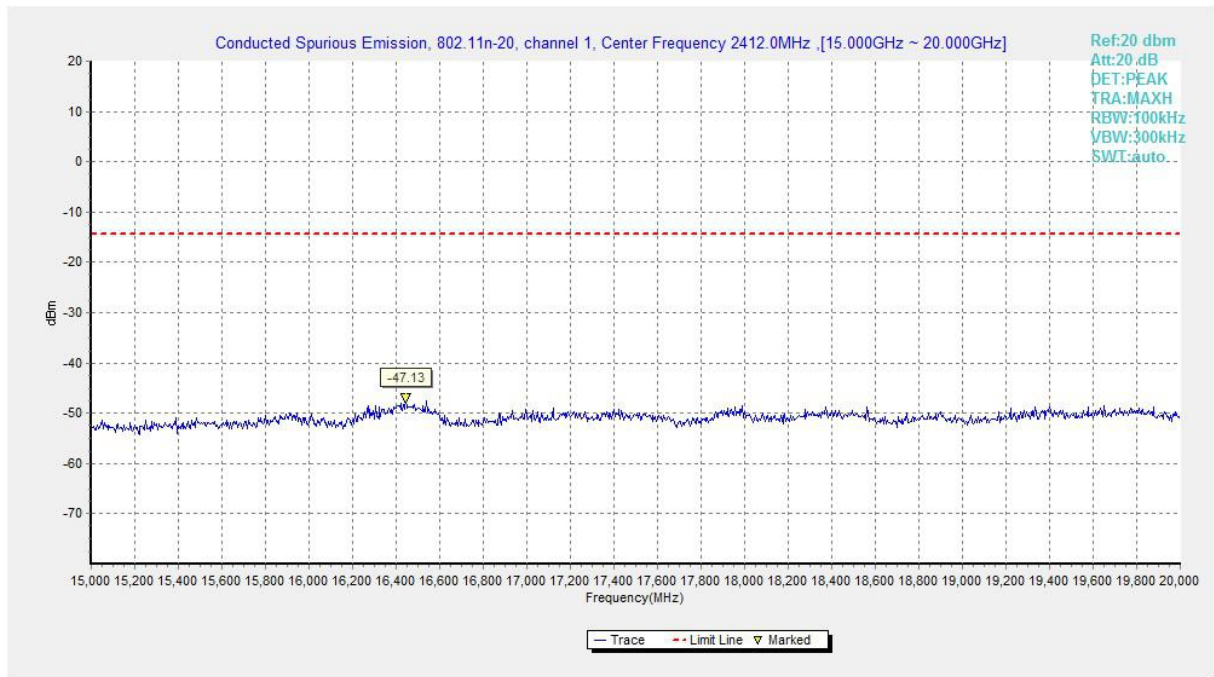
Fig.A.6.1.7 Transmitter Spurious Emission - Conducted (802.11n-HT20, Ch1, 15 GHz-20 GHz)
