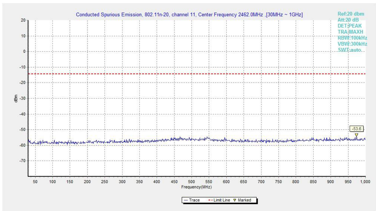
Fig.A.6.1.18 Transmitter Spurious Emission - Conducted (802.11n-HT20, Ch11, 30 MHz-1 GHz)
