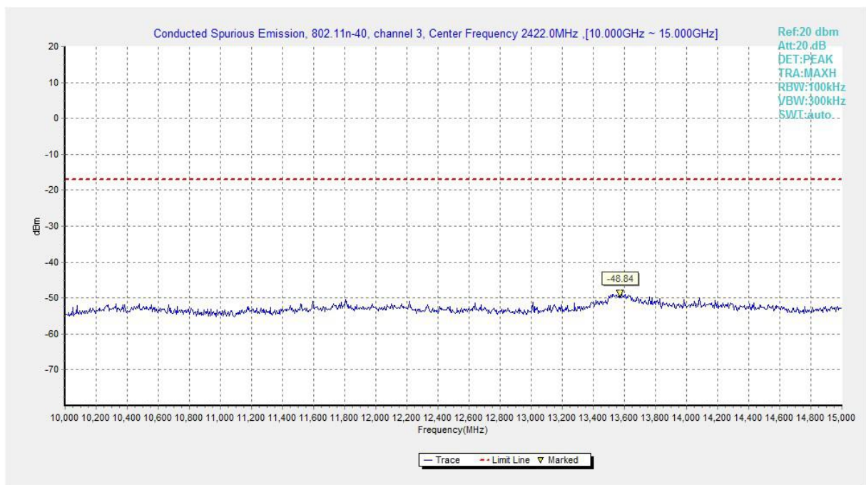
Fig.A.6.1.30 Transmitter Spurious Emission - Conducted (802.11n-HT40, Ch3, 10 GHz-15 GHz)
