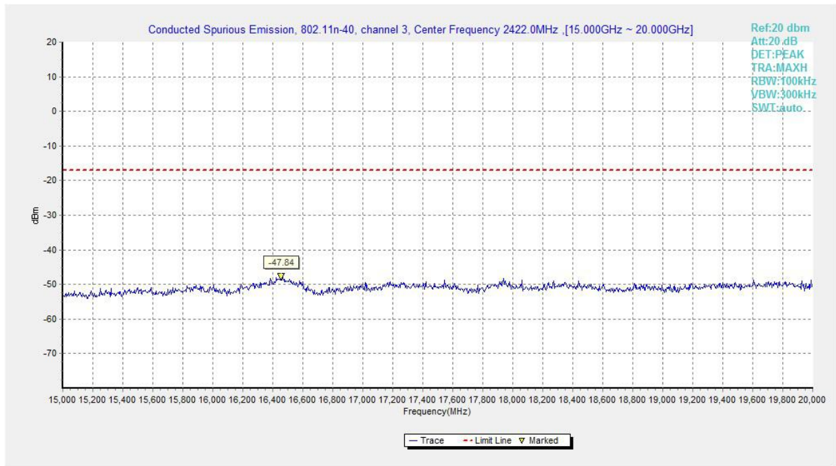
Fig.A.6.1.31 Transmitter Spurious Emission - Conducted (802.11n-HT40, Ch3, 15 GHz-20 GHz)
