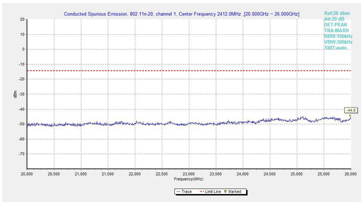
Fig.A.6.1.8 Transmitter Spurious Emission - Conducted (802.11n-HT20, Ch1, 20 GHz-26 GHz)
