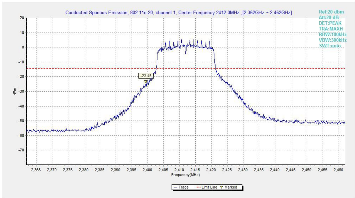
Fig.A.6.1.1 Transmitter Spurious Emission - Conducted (802.11n-HT20, Ch1, Center Frequency)
