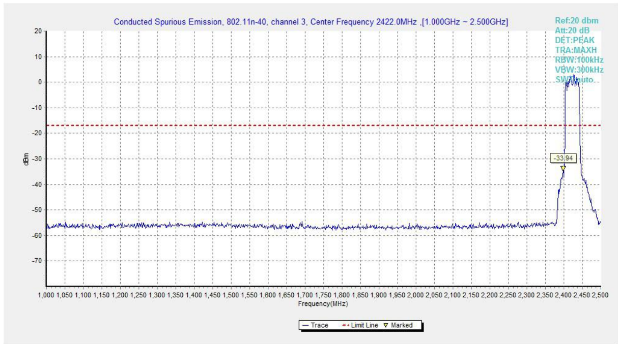
Fig.A.6.1.27 Transmitter Spurious Emission - Conducted (802.11n-HT40, Ch3, 1 GHz-2.5 GHz)
