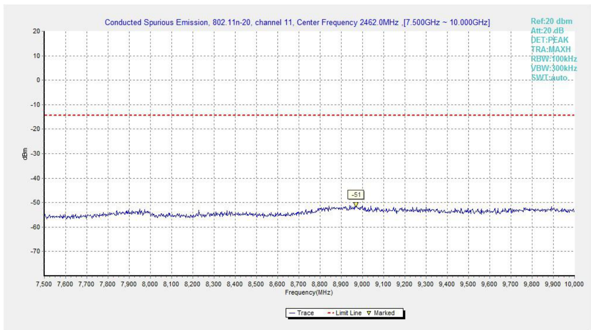
Fig.A.6.1.21 Transmitter Spurious Emission - Conducted (802.11n-HT20, Ch11, 7.5 GHz-10 GHz)
