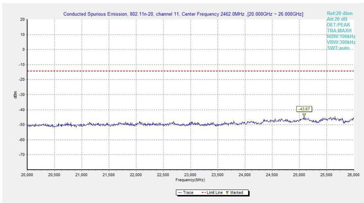
Fig.A.6.1.24 Transmitter Spurious Emission - Conducted (802.11n-HT20, Ch11, 20 GHz-26 GHz)
