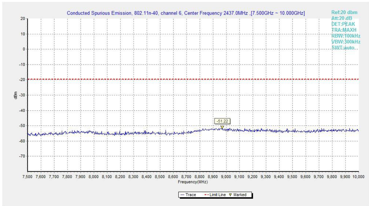
Fig.A.6.1.37 Transmitter Spurious Emission - Conducted (802.11n-HT40, Ch6, 7.5 GHz-10 GHz)
