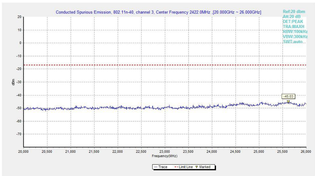
Fig.A.6.1.32 Transmitter Spurious Emission - Conducted (802.11n-HT40, Ch3, 20 GHz-26 GHz)
