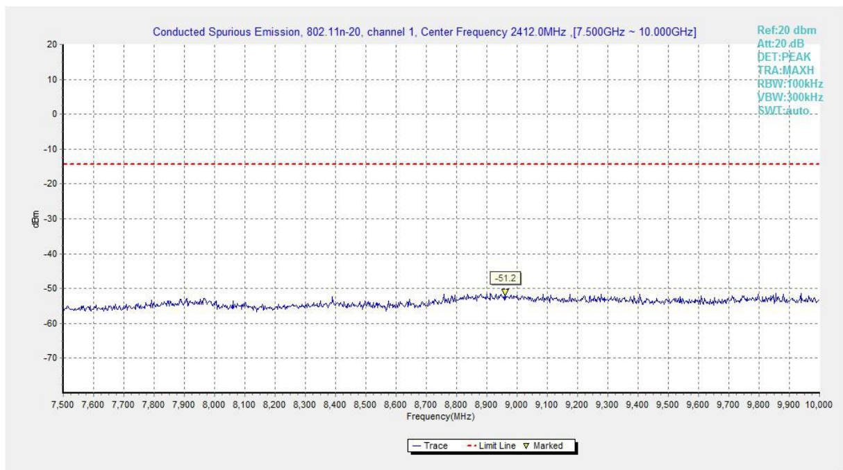
Fig.A.6.1.5 Transmitter Spurious Emission - Conducted (802.11n-HT20, Ch1, 7.5 GHz-10 GHz)
