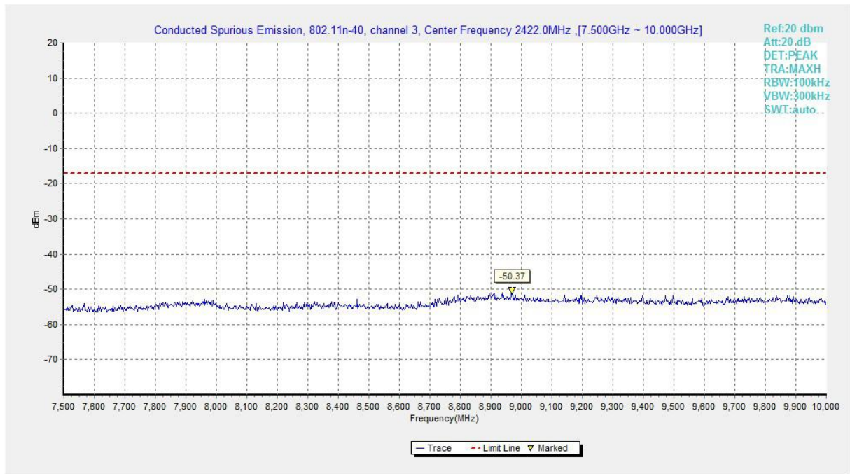
Fig.A.6.1.29 Transmitter Spurious Emission - Conducted (802.11n-HT40, Ch3, 7.5 GHz-10 GHz)
