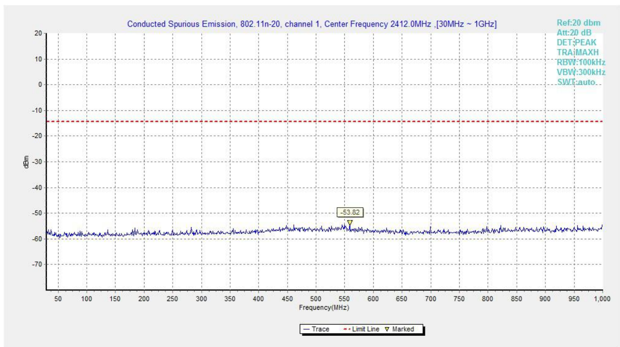
Fig.A.6.1.2 Transmitter Spurious Emission - Conducted (802.11n-HT20, Ch1, 30 MHz-1 GHz)
