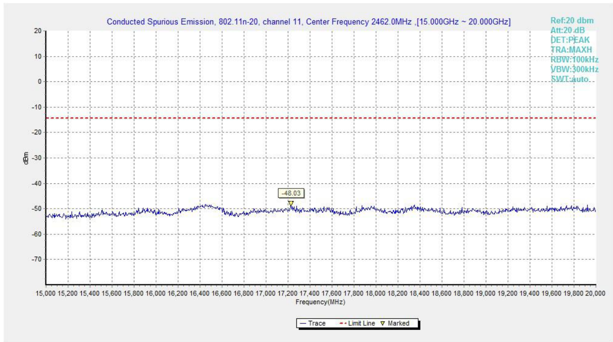
Fig.A.6.1.23 Transmitter Spurious Emission - Conducted (802.11n-HT20, Ch11, 15 GHz-20 GHz)
