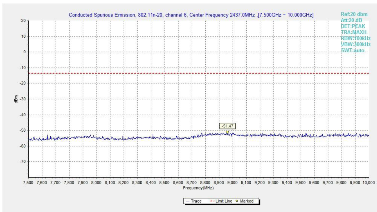
Fig.A.6.1.13 Transmitter Spurious Emission - Conducted (802.11n-HT20, Ch6, 7.5 GHz-10 GHz)
