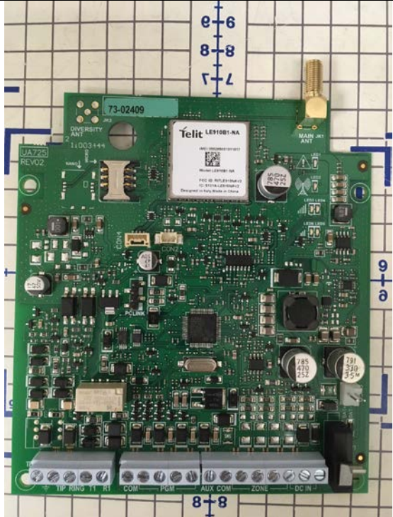
Host - Board Front View
