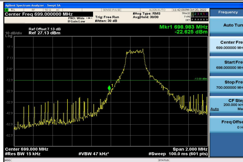
Band12-1.4MHz-16QAM-23017-1RB#0
