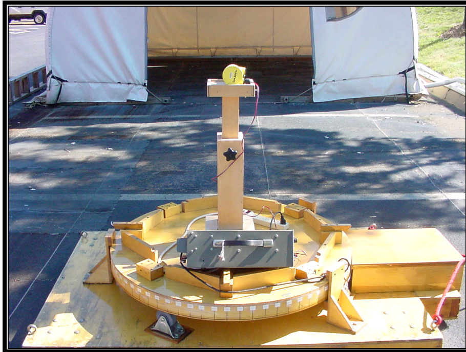
Photograph 12: Radiated Emissions Rear View 19.5 dBi Rod Antenna
