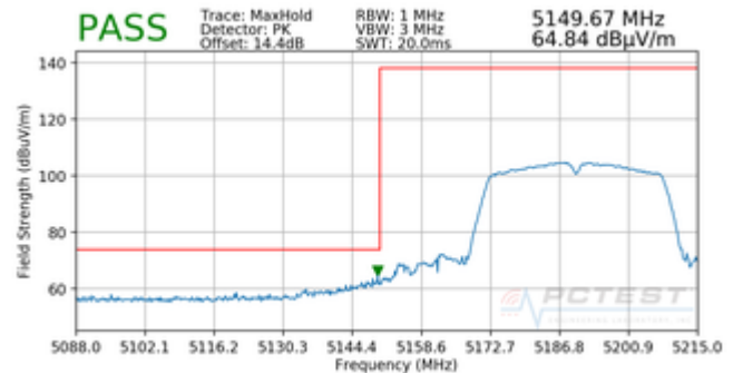
Plot 7-15. Radiated Lower Band Edge Plot (Peak – UNII Band 1)
