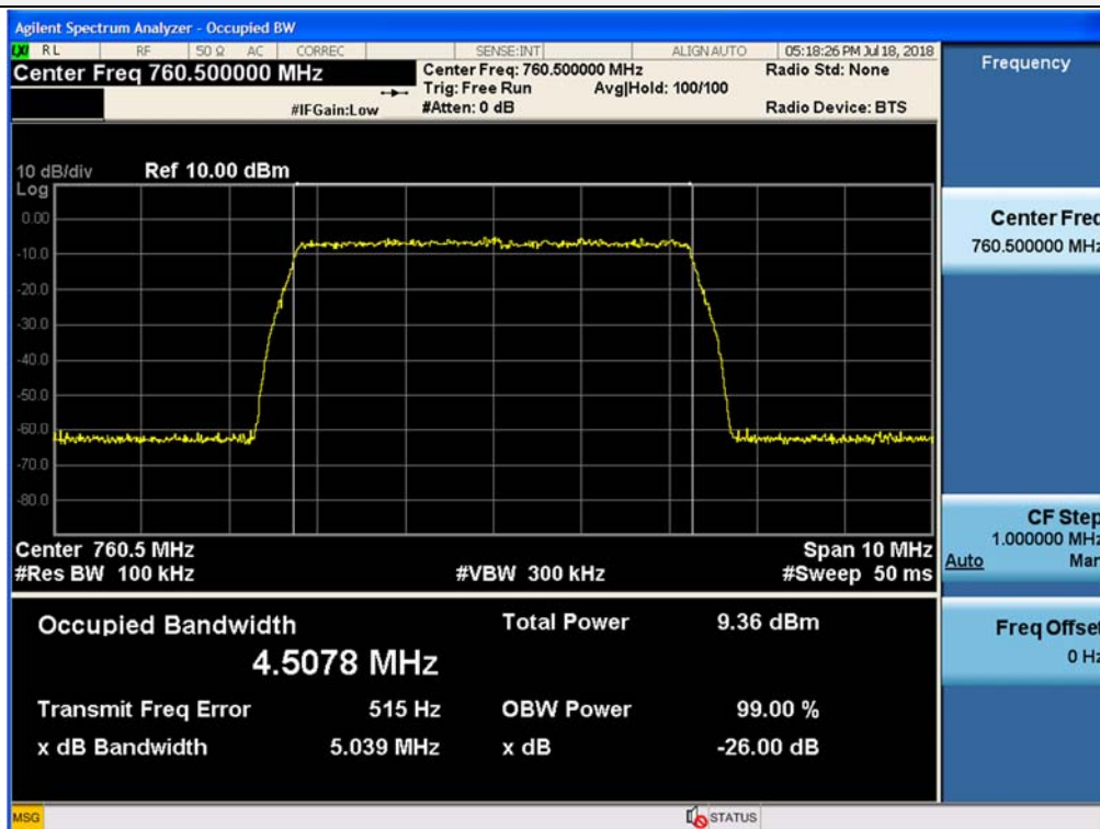
Input / FirstNet / Downlink / LTE 5 MHz / Low Channel
