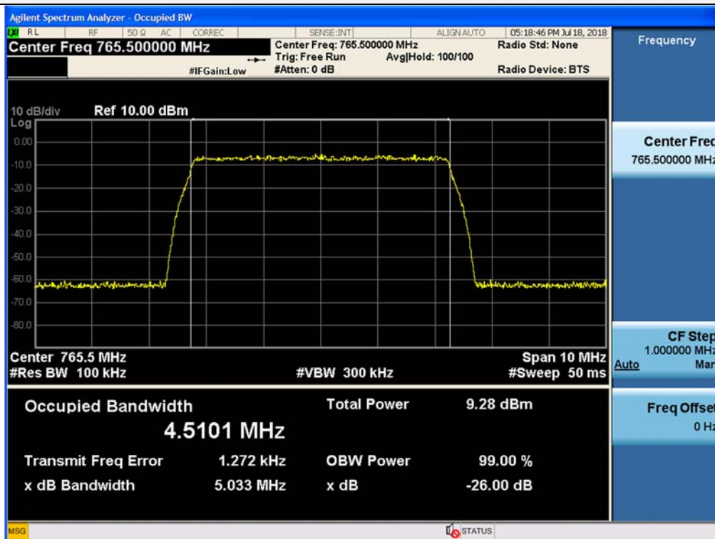
Input / FirstNet / Downlink / LTE 5 MHz / High Channel
