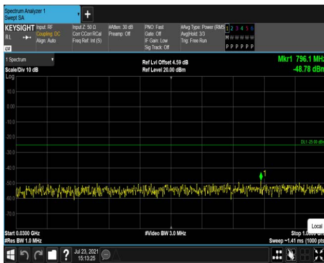
Band41-20MHz-16QAM-40640:30~1000MHz
