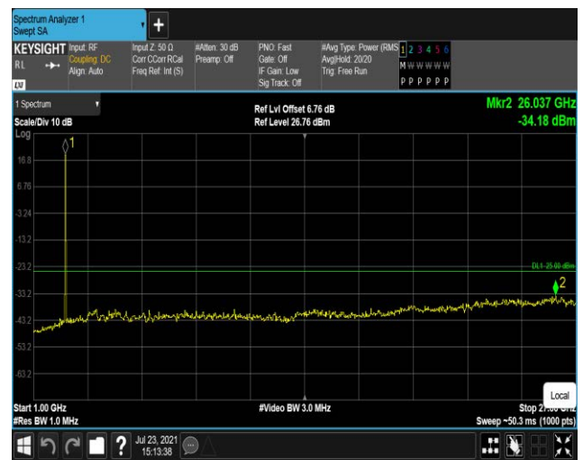
Band41-20MHz-16QAM-40640:1000~27000MHz
