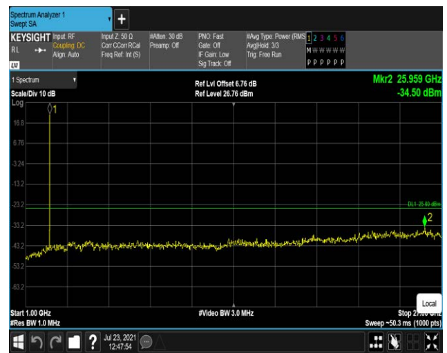
Band7-5MHz-QPSK-21100:1000~27000MHz
