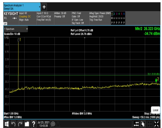
Band38-5MHz-QPSK-38000:1000~27000MHz
