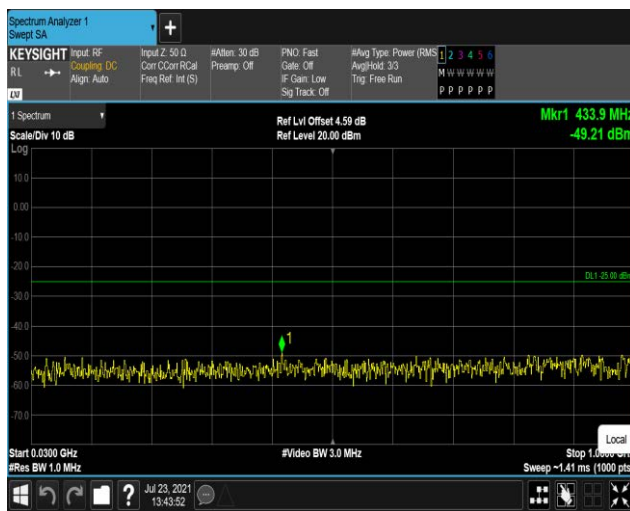
Band38-5MHz-16QAM-38000:30~1000MHz
