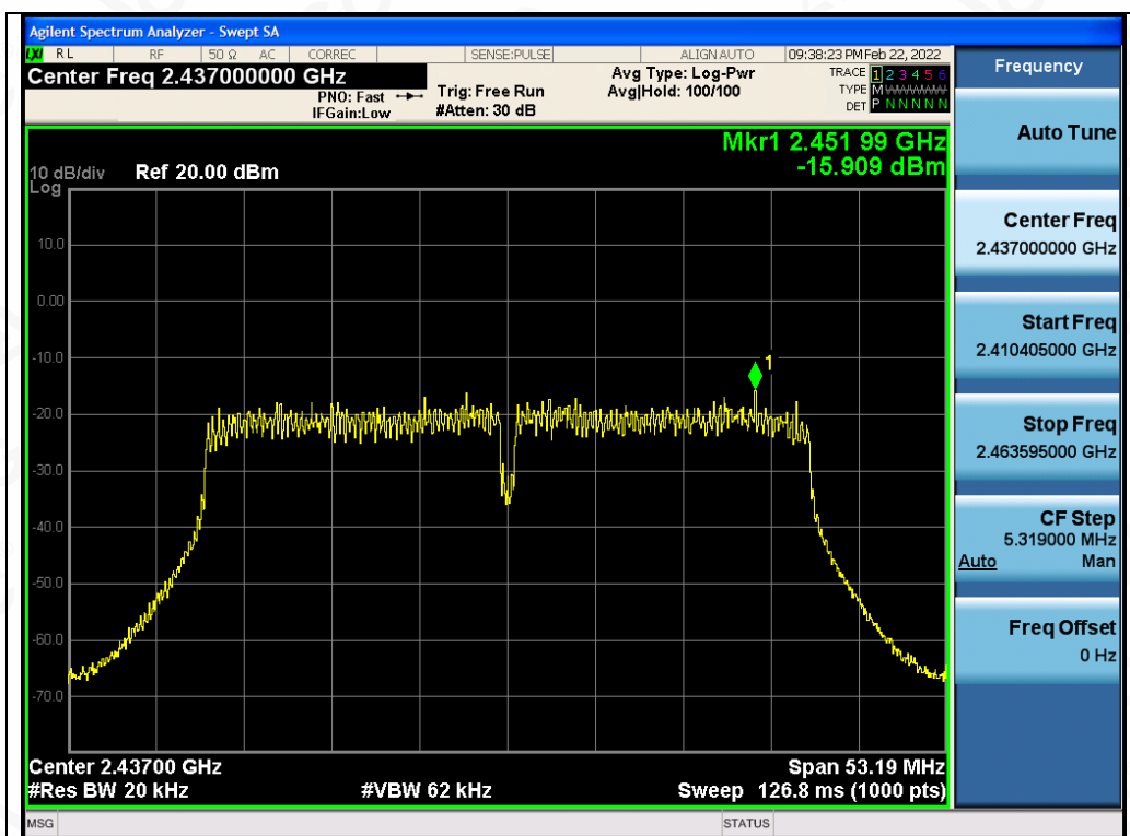
Test_Graph_802.11n40_ANT2_2437_MCS0_PSD
