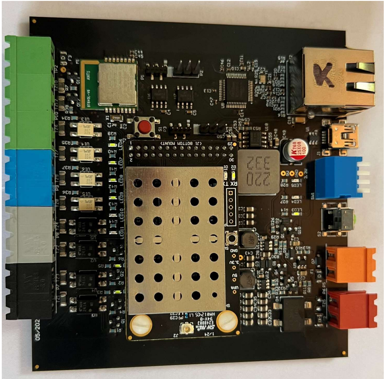
Top with Shield
