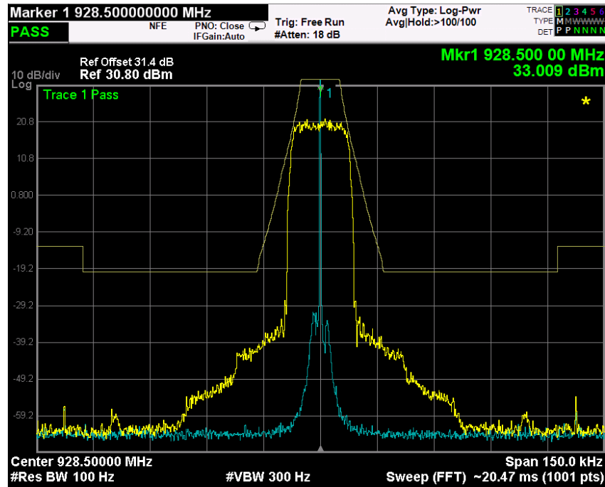
Mask with BW &gt;12,5KHz signal
