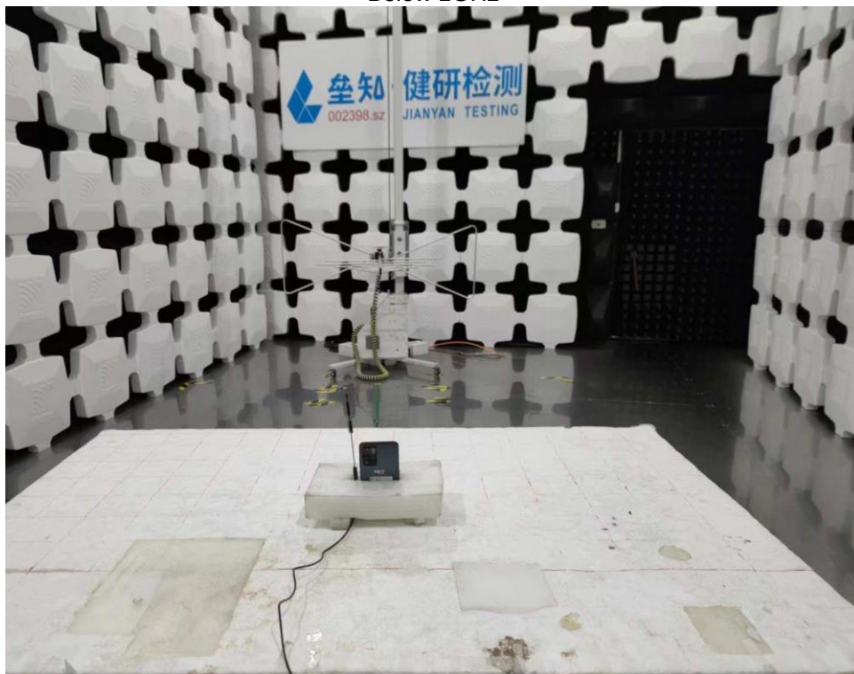
Radiated Spurious Emission Below 1GHz
