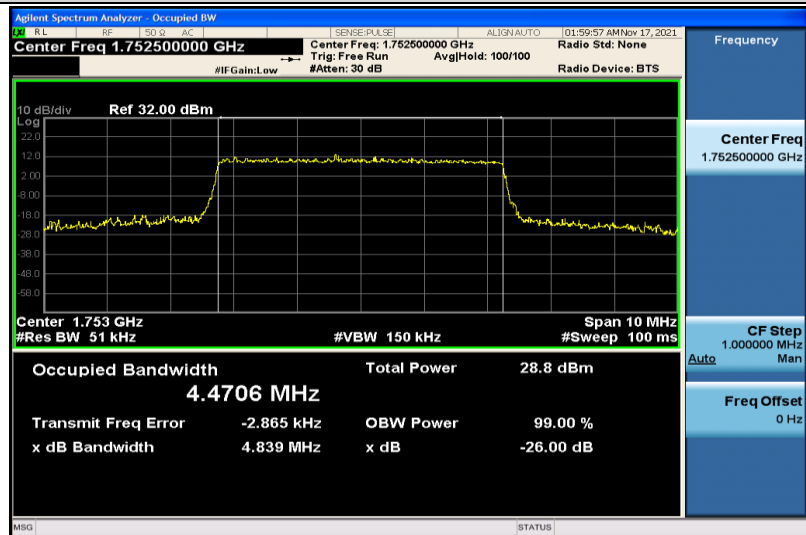
Band4-5MHz-16QAM-20375-25RB#0-4.4706
