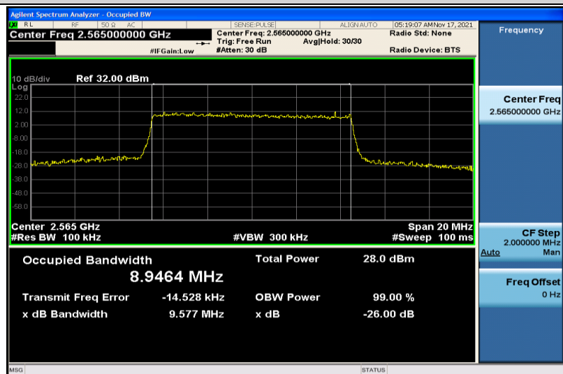
Band7-10MHz-16QAM-21400-50RB#0-8.9464
