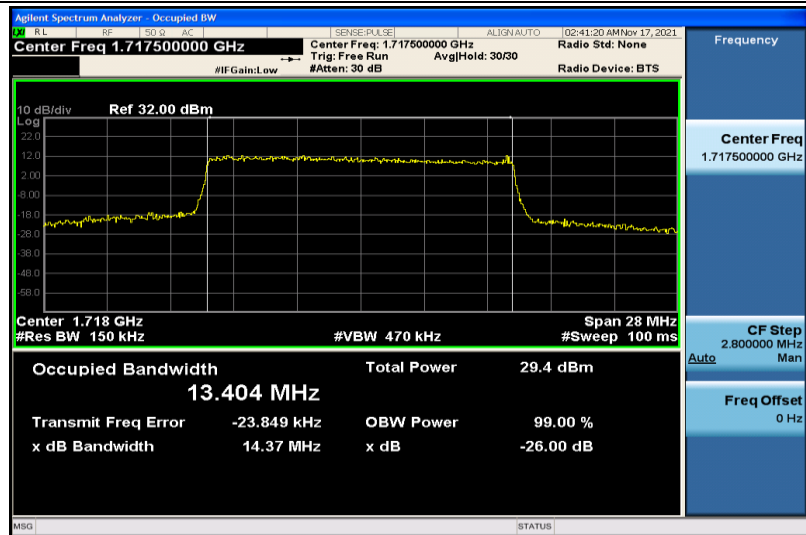
Band4-15MHz-16QAM-20025-75RB#0-13.404
