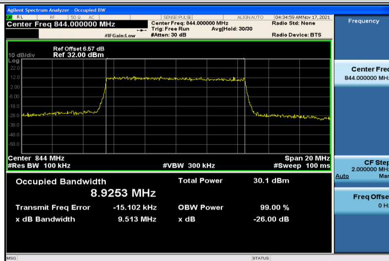
Band5-10MHz-16QAM-20600-50RB#0-8.9253
