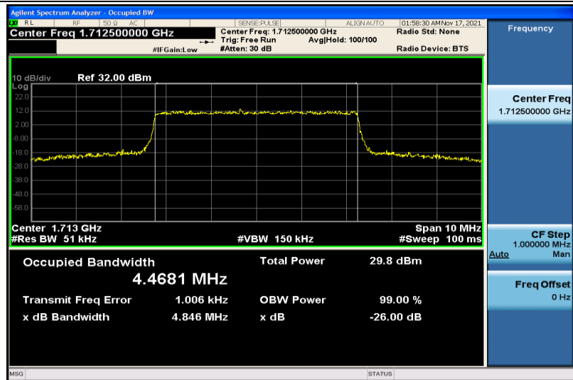
Band4-5MHz-QPSK-19975-25RB#0-4.4681
