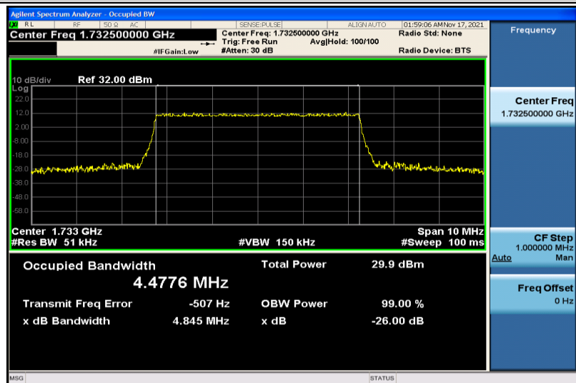
Band4-5MHz-QPSK-20175-25RB#0-4.4776
