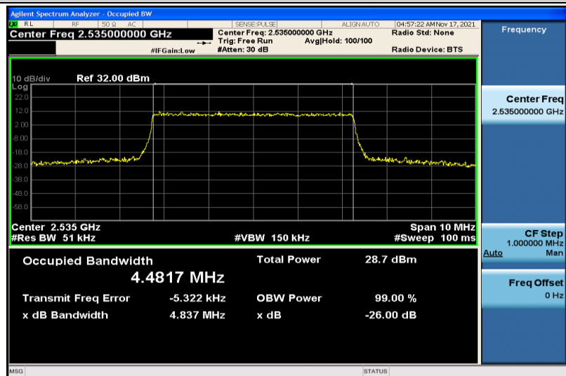
Band7-5MHz-QPSK-21100-25RB#0-4.4817
