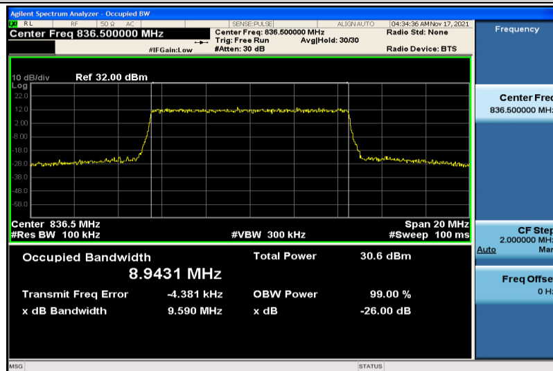
Band5-10MHz-16QAM-20525-50RB#0-8.9431
