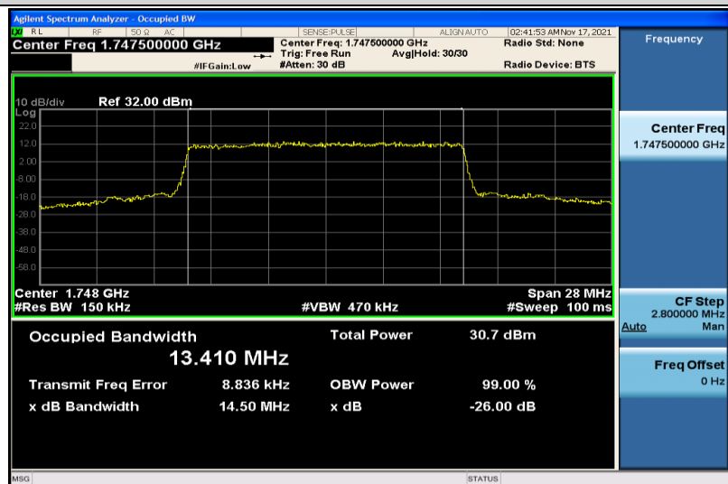
Band4-15MHz-QPSK-20325-75RB#0-13.410
