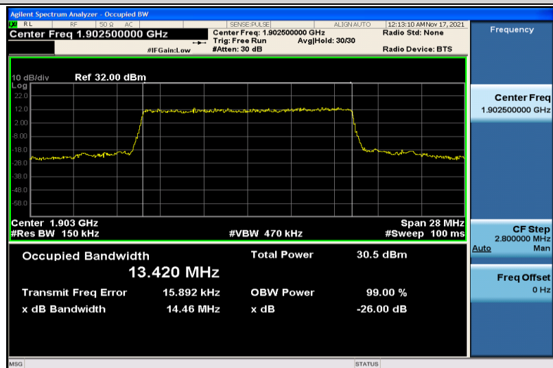
Band2-15MHz-QPSK-19125-75RB#0-13.420
