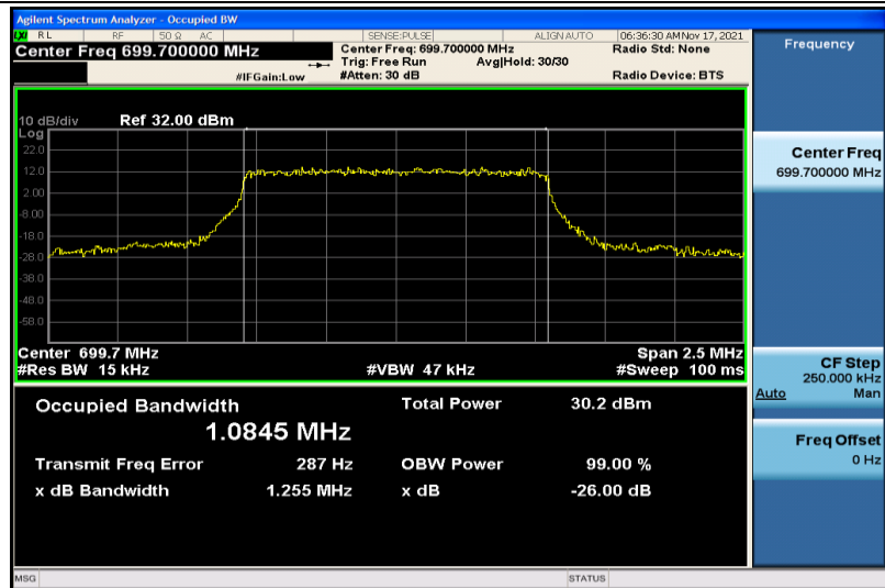
Band12-1.4MHz-QPSK-23017-6RB#0-1.0845
