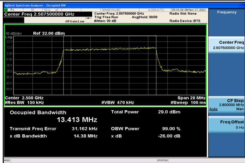
Band7-15MHz-QPSK-20825-75RB#0-13.413
