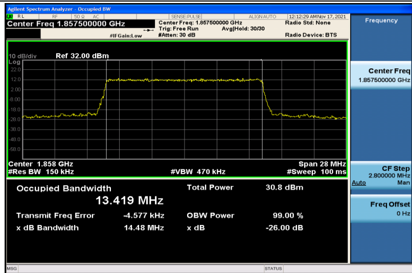
Band2-15MHz-QPSK-18675-75RB#0-13.419
