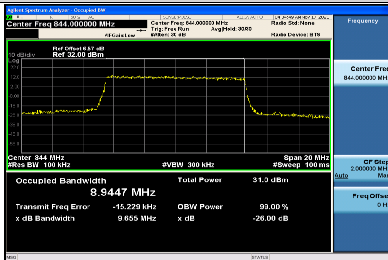
Band5-10MHz-QPSK-20600-50RB#0-8.9447
