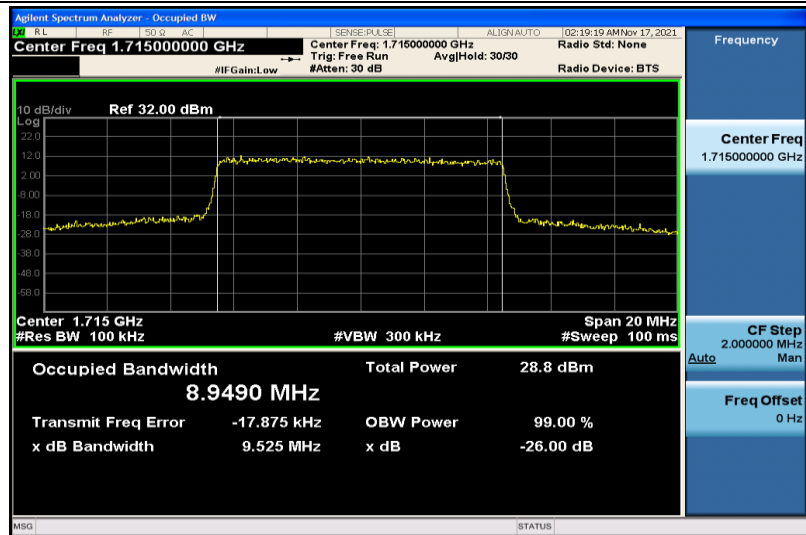
Band4-10MHz-16QAM-20000-50RB#0-8.9490
