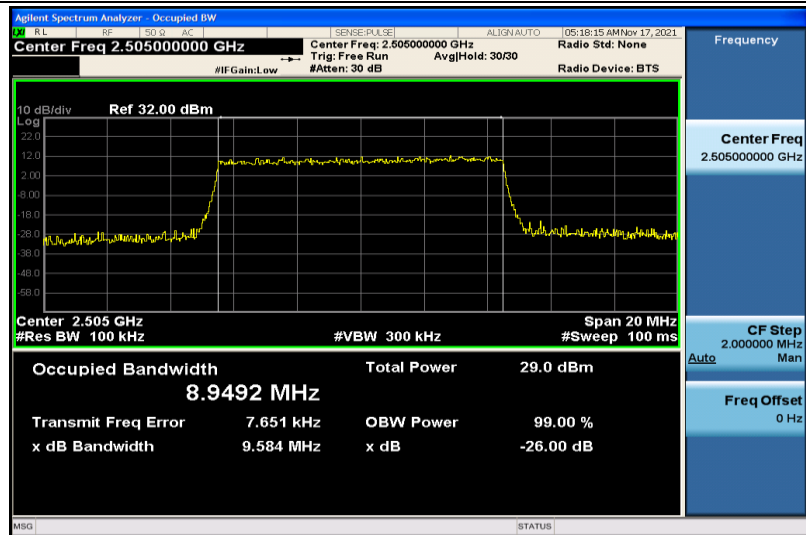
Band7-10MHz-QPSK-20800-50RB#0-8.9492
