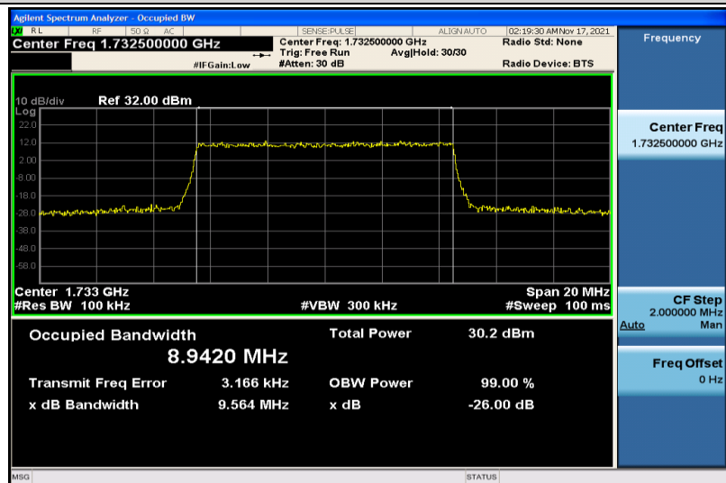
Band4-10MHz-QPSK-20175-50RB#0-8.9420
