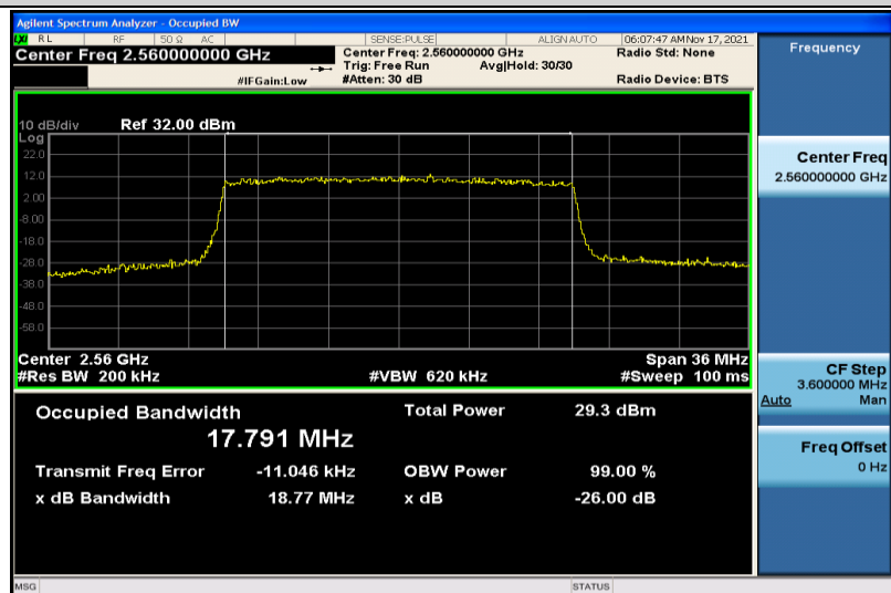
Band7-20MHz-QPSK-21350-100RB#0-17.791
