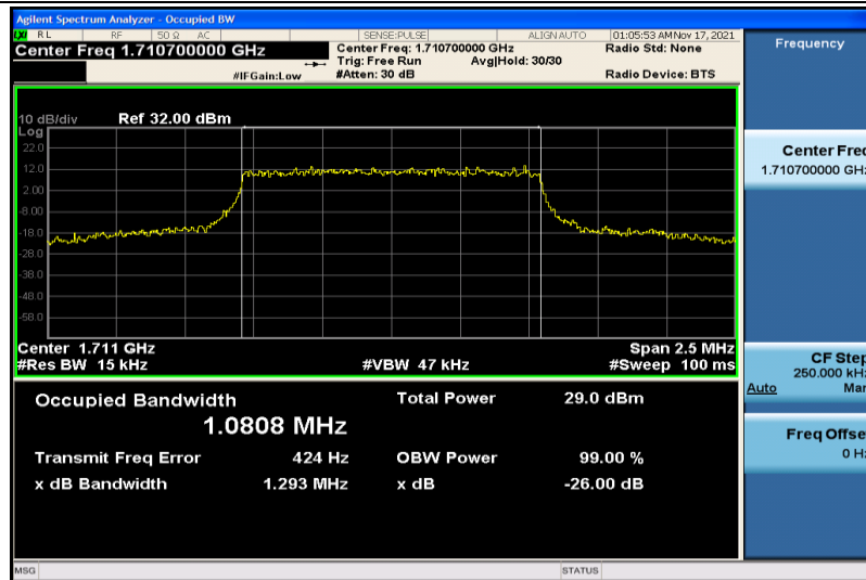
Band4-1.4MHz-QPSK-19957-6RB#0-1.0808
