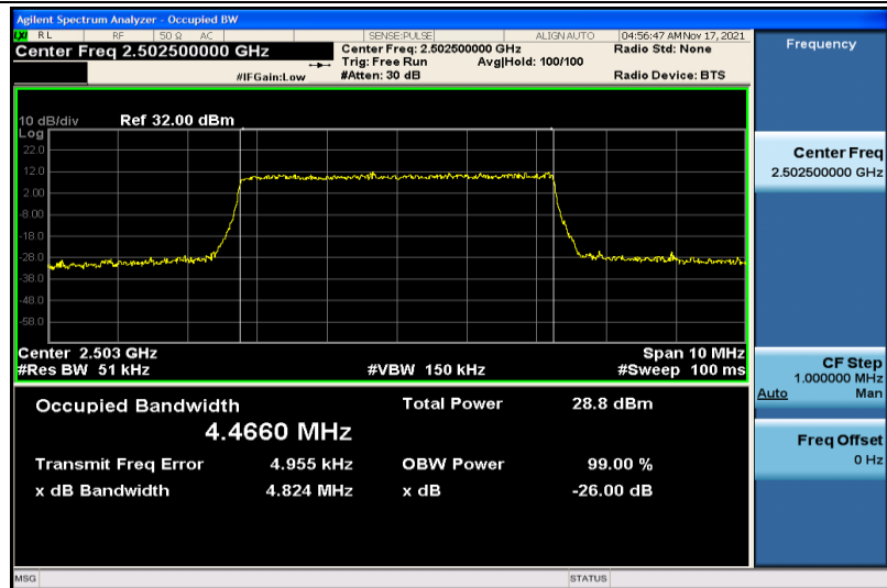
Band7-5MHz-QPSK-20775-25RB#0-4.4660
