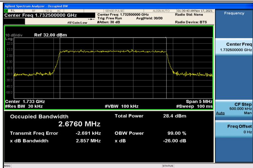
Band4-3MHz-16QAM-20175-15RB#0-2.6760
