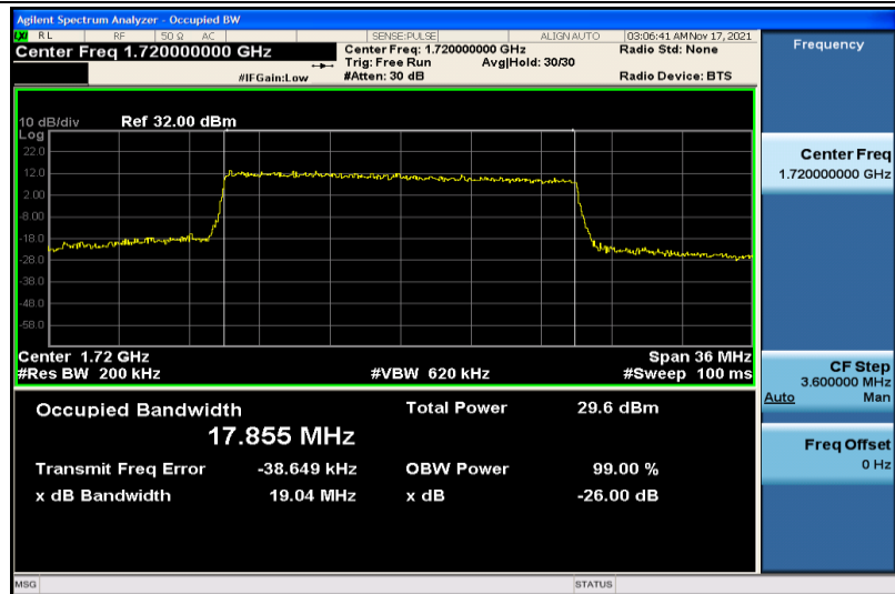
Band4-20MHz-16QAM-20050-100RB#0-17.855
