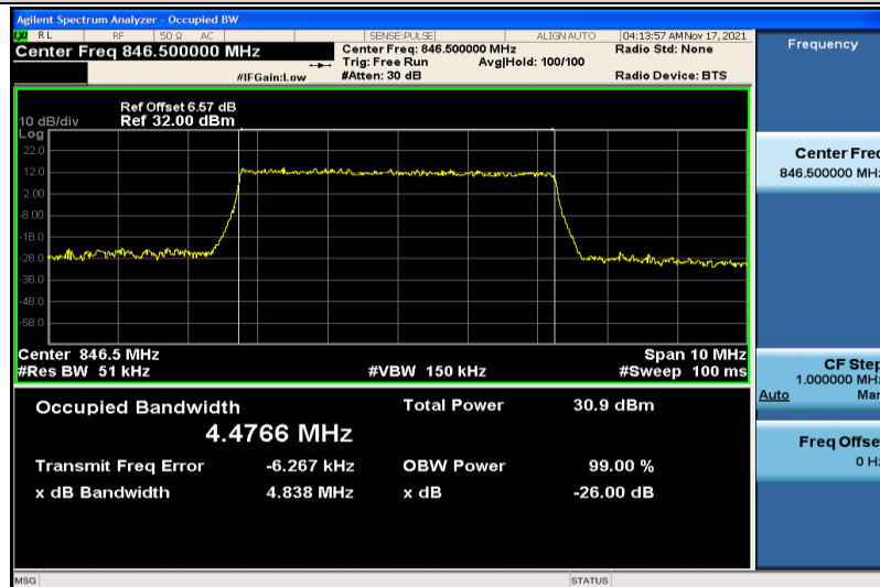
Band5-5MHz-QPSK-20625-25RB#0-4.4766
