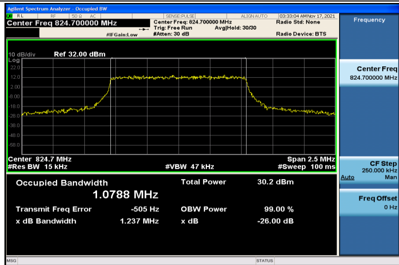
Band5-1.4MHz-QPSK-20407-6RB#0-1.0788
