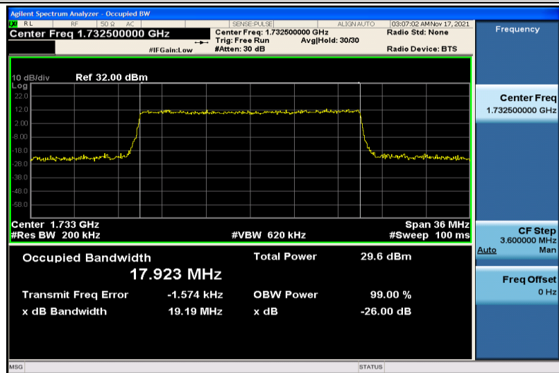
Band4-20MHz-16QAM-20175-100RB#0-17.923
