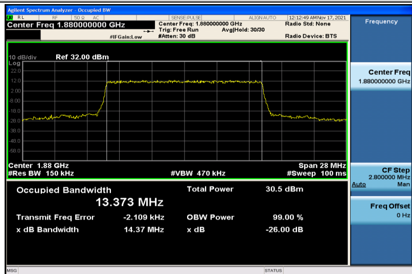
Band2-15MHz-QPSK-18900-75RB#0-13.373
