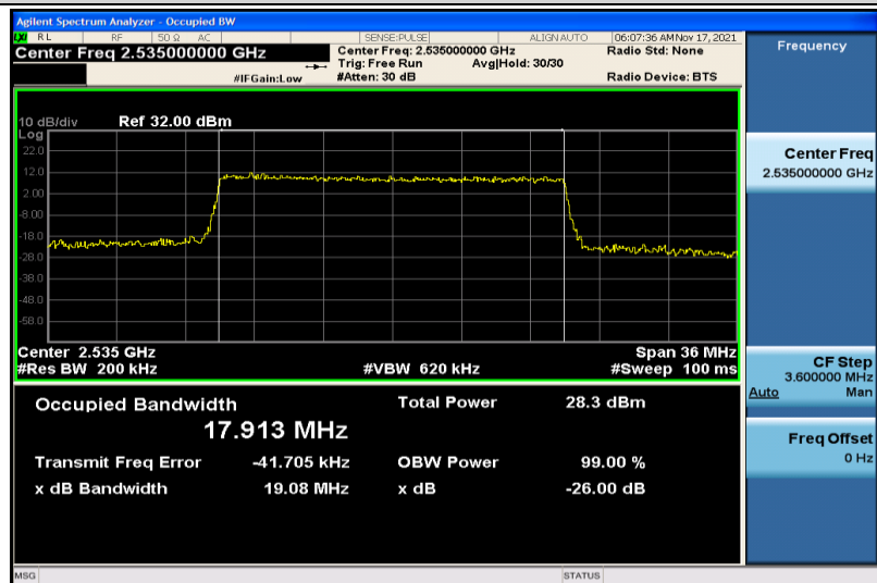
Band7-20MHz-16QAM-21100-100RB#0-17.913
