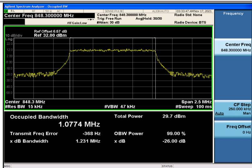
Band5-1.4MHz-QPSK-20643-6RB#0-1.0774
