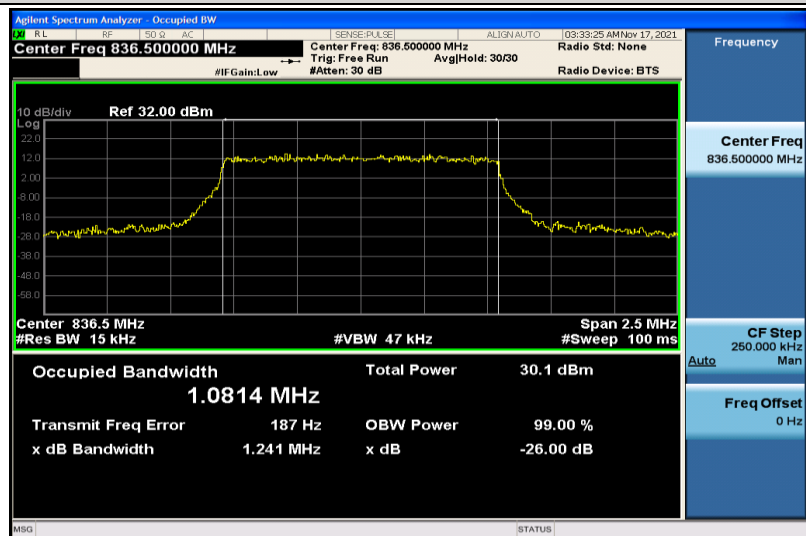
Band5-1.4MHz-QPSK-20525-6RB#0-1.0814
