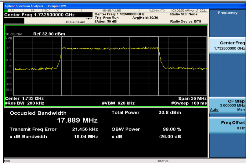
Band4-20MHz-QPSK-20175-100RB#0-17.889
