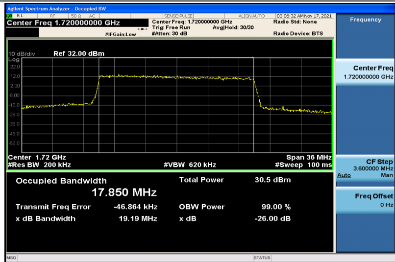
Band4-20MHz-QPSK-20050-100RB#0-17.850
