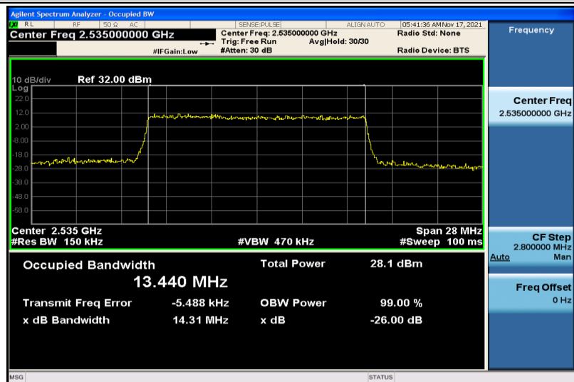
Band7-15MHz-16QAM-21100-75RB#0-13.440
