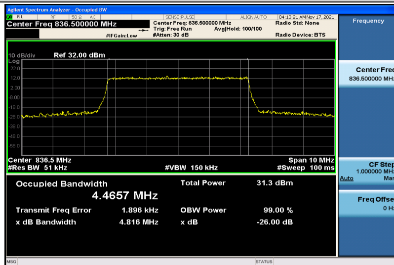
Band5-5MHz-QPSK-20525-25RB#0-4.4657
