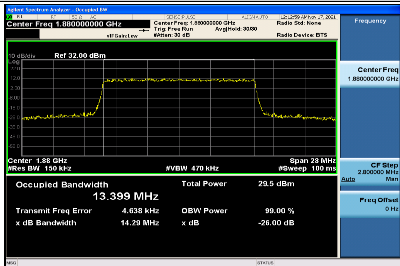
Band2-15MHz-16QAM-18900-75RB#0-13.399
