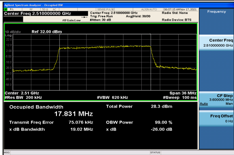
Band7-20MHz-16QAM-20850-100RB#0-17.831
