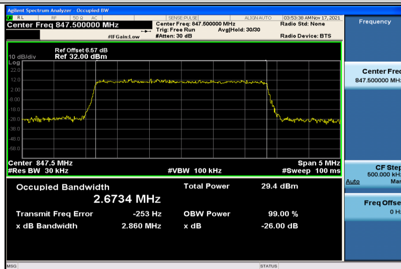
Band5-3MHz-16QAM-20635-15RB#0-2.6734
