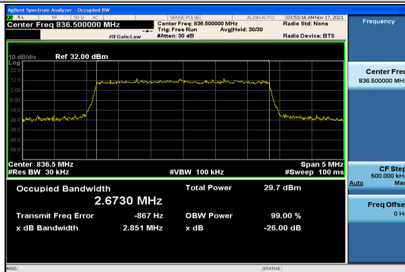
Band5-3MHz-16QAM-20525-15RB#0-2.6730
