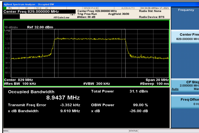
Band5-10MHz-QPSK-20450-50RB#0-8.9437
