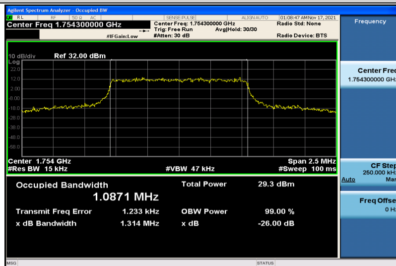
Band4-1.4MHz-QPSK-20393-6RB#0-1.0871
