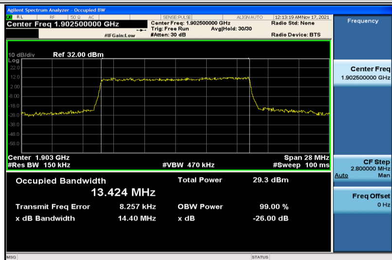
Band2-15MHz-16QAM-19125-75RB#0-13.424
