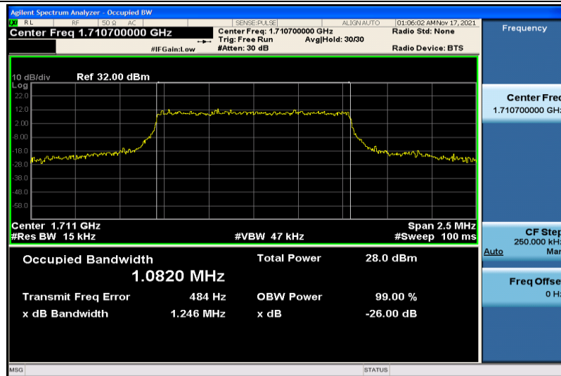
Band4-1.4MHz-16QAM-19957-6RB#0-1.0820
