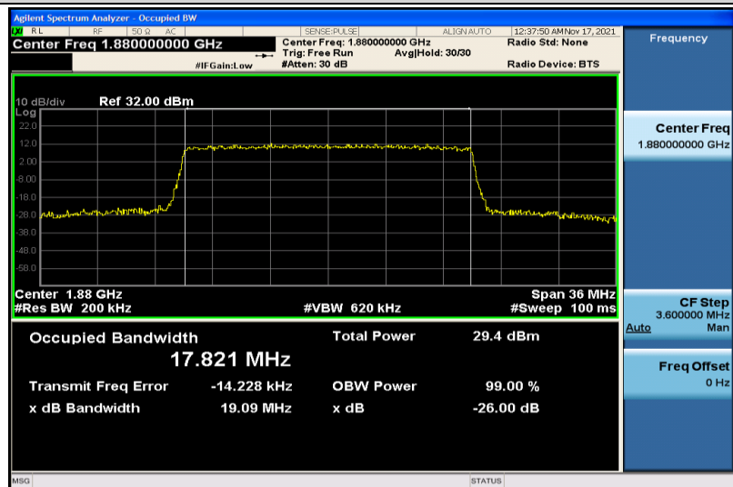
Band2-20MHz-16QAM-18900-100RB#0-17.821
