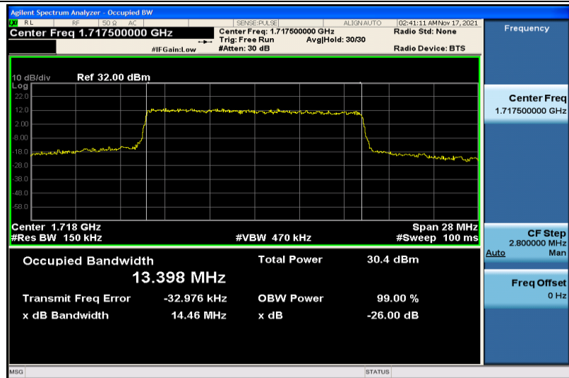
Band4-15MHz-QPSK-20025-75RB#0-13.398
