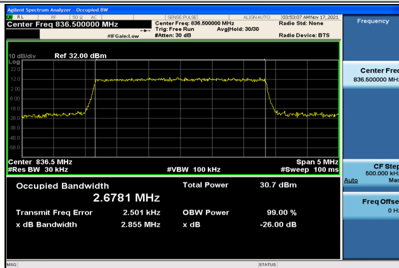
Band5-3MHz-QPSK-20525-15RB#0-2.6781
