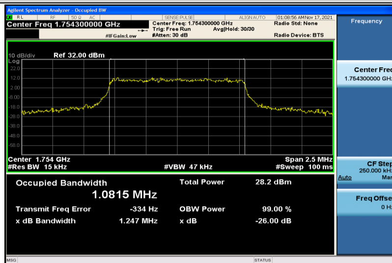
Band4-1.4MHz-16QAM-20393-6RB#0-1.0815
