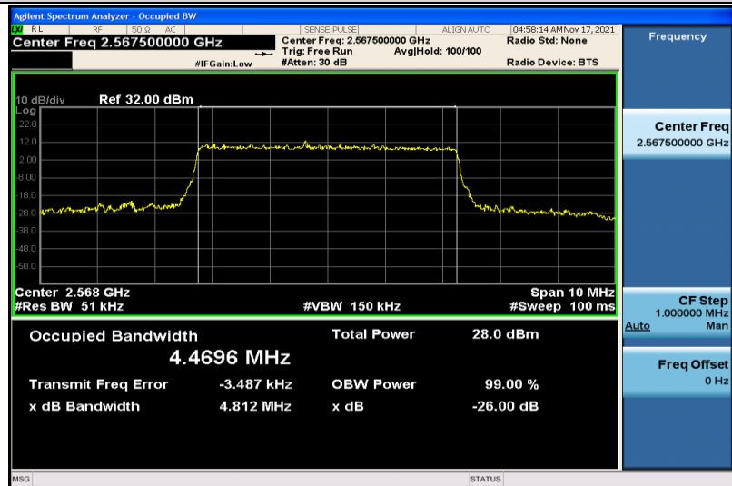
Band7-5MHz-16QAM-21425-25RB#0-4.4696
