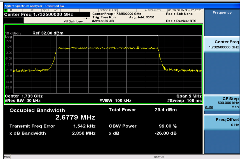
Band4-3MHz-QPSK-20175-15RB#0-2.6779
