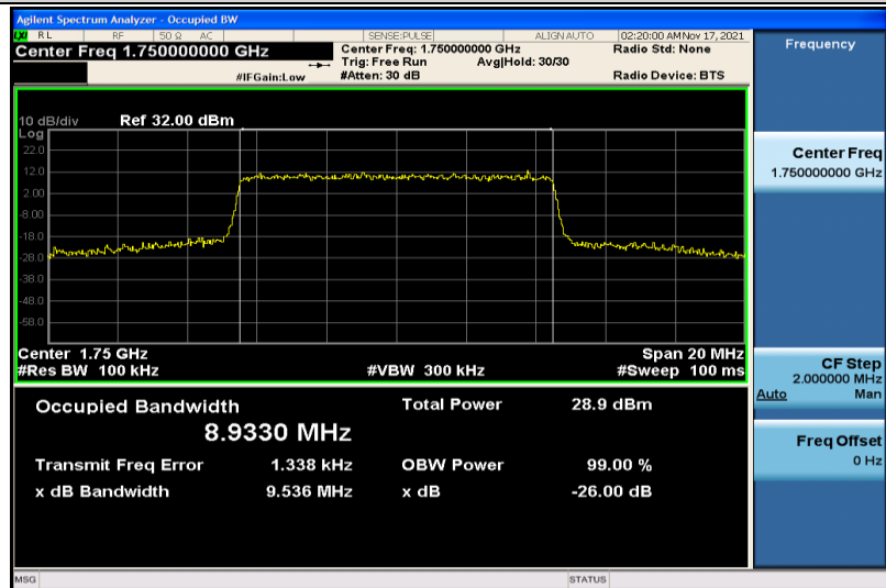
Band4-10MHz-16QAM-20350-50RB#0-8.9330
