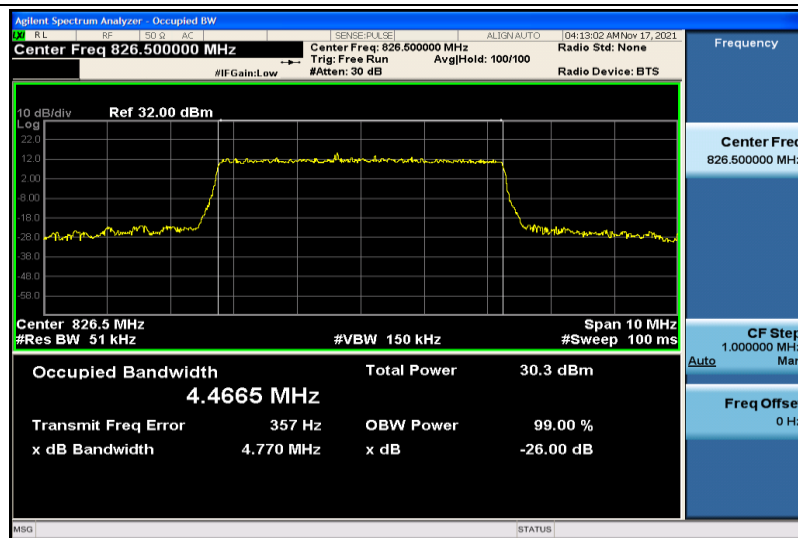
Band5-5MHz-16QAM-20425-25RB#0-4.4665
