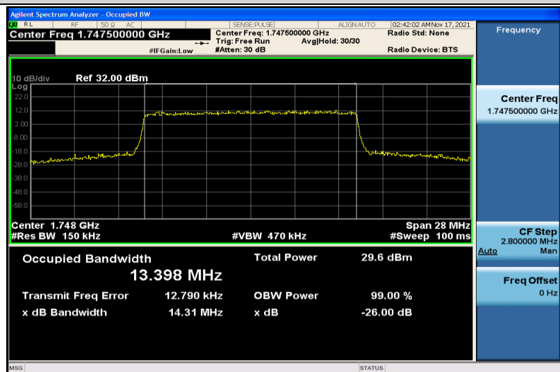
Band4-15MHz-16QAM-20325-75RB#0-13.398
