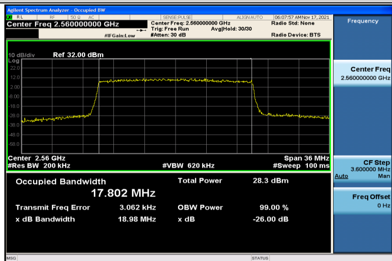
Band7-20MHz-16QAM-21350-100RB#0-17.802
