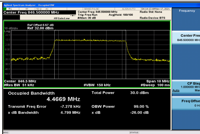
Band5-5MHz-16QAM-20625-25RB#0-4.4669
