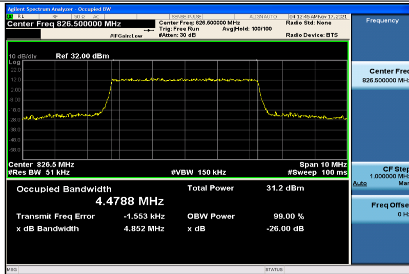
Band5-5MHz-QPSK-20425-25RB#0-4.4788
