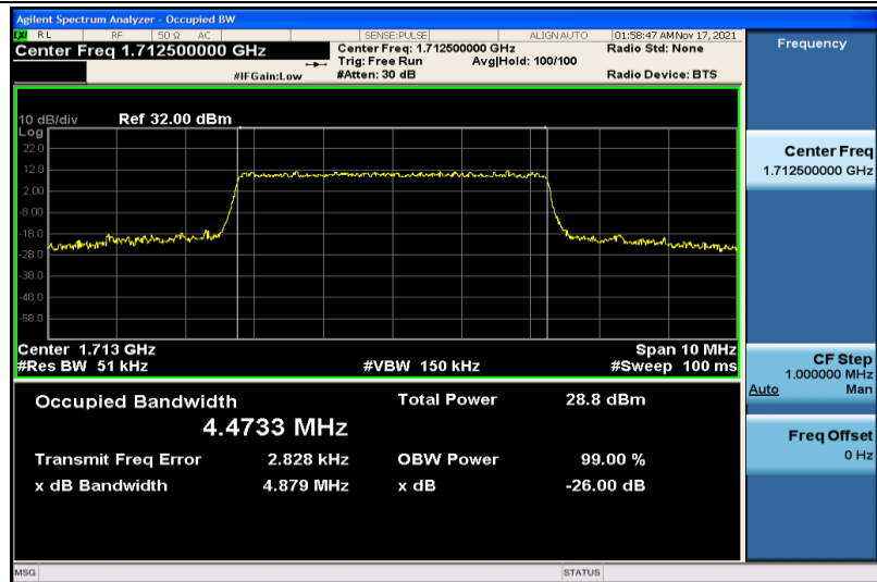
Band4-5MHz-16QAM-19975-25RB#0-4.4733
