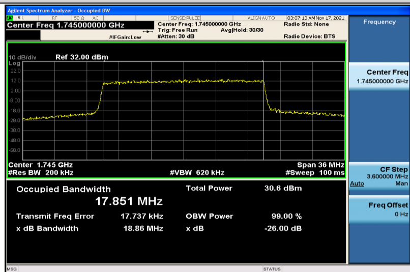
Band4-20MHz-QPSK-20300-100RB#0-17.851
