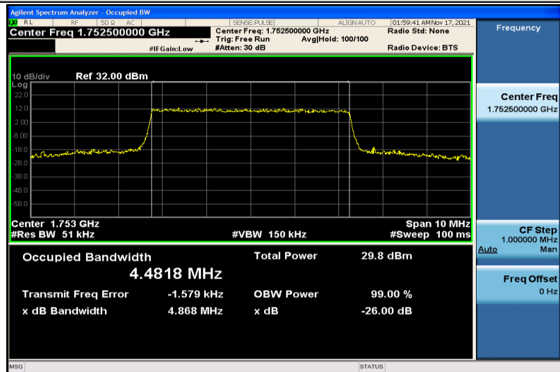
Band4-5MHz-QPSK-20375-25RB#0-4.4818
