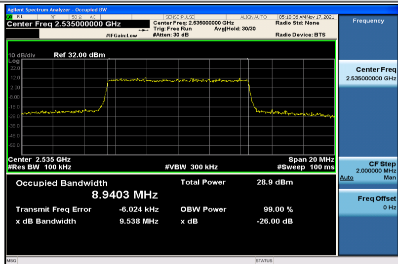
Band7-10MHz-QPSK-21100-50RB#0-8.9403
