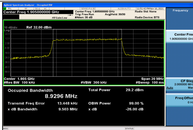
Band2-10MHz-16QAM-19150-50RB#0-8.9296
