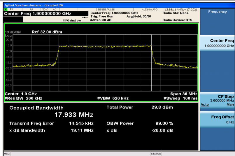
Band2-20MHz-16QAM-19100-100RB#0-17.933
