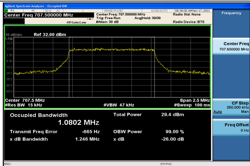
Band12-1.4MHz-16QAM-23095-6RB#0-1.0802
