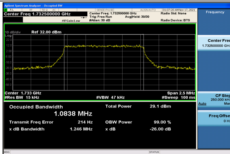
Band4-1.4MHz-QPSK-20175-6RB#0-1.0838
