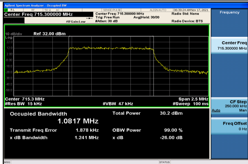
Band12-1.4MHz-QPSK-23173-6RB#0-1.0817
