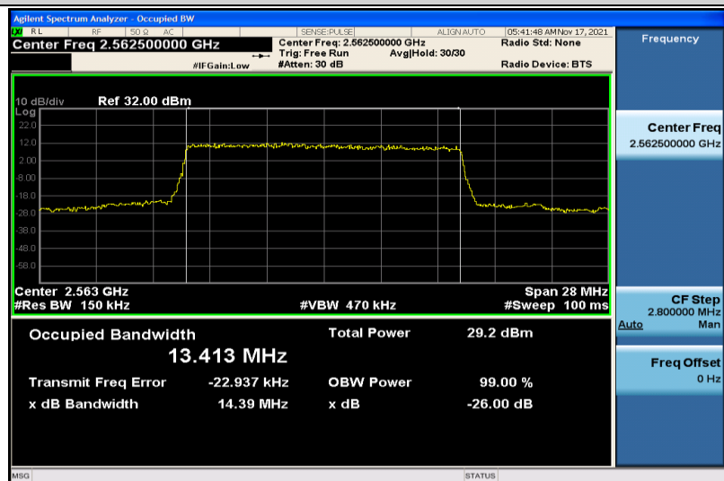
Band7-15MHz-QPSK-21375-75RB#0-13.413
