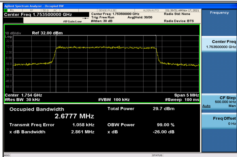
Band4-3MHz-QPSK-20385-15RB#0-2.6777
