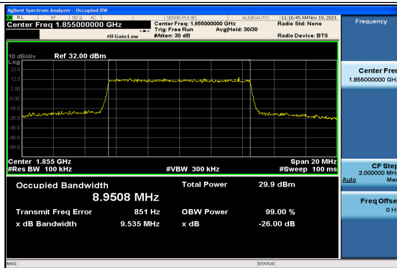
Band2-10MHz-16QAM-18650-50RB#0-8.9508
