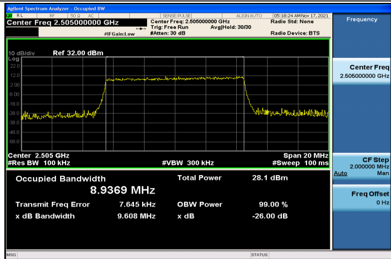
Band7-10MHz-16QAM-20800-50RB#0-8.9369
