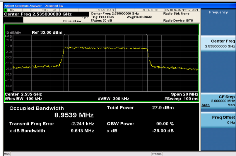
Band7-10MHz-16QAM-21100-50RB#0-8.9539
