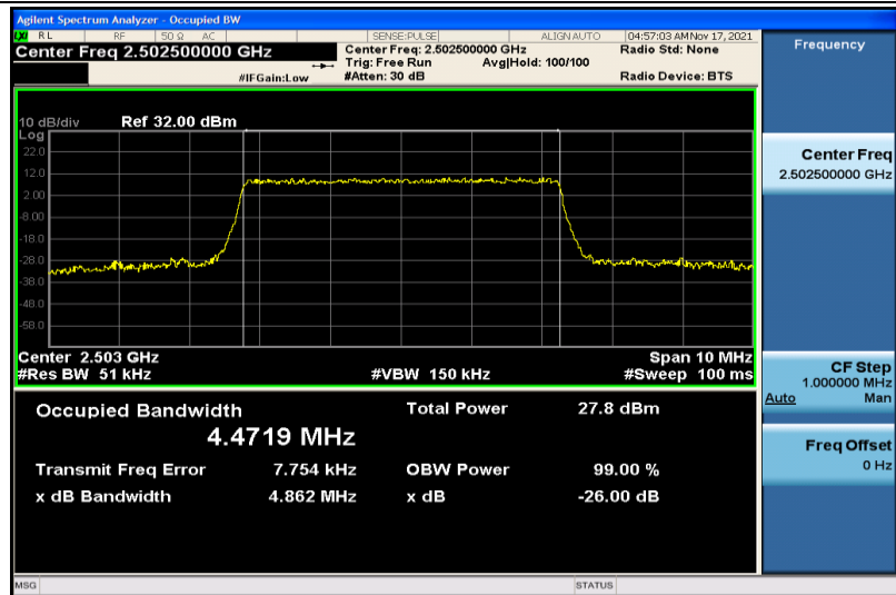
Band7-5MHz-16QAM-20775-25RB#0-4.4719
