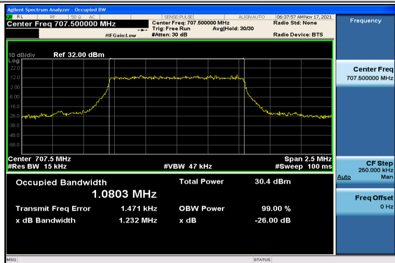
Band12-1.4MHz-QPSK-23095-6RB#0-1.0803
