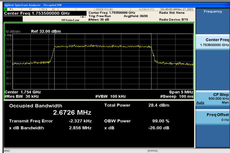
Band4-3MHz-16QAM-20385-15RB#0-2.6726
