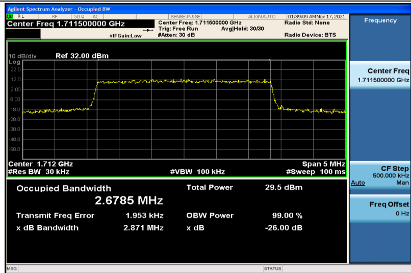
Band4-3MHz-QPSK-19965-15RB#0-2.6785
