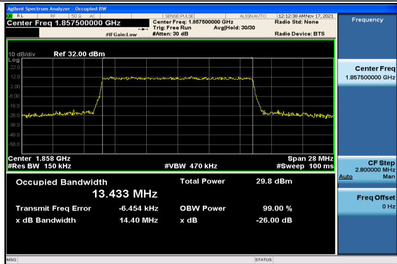
Band2-15MHz-16QAM-18675-75RB#0-13.433
