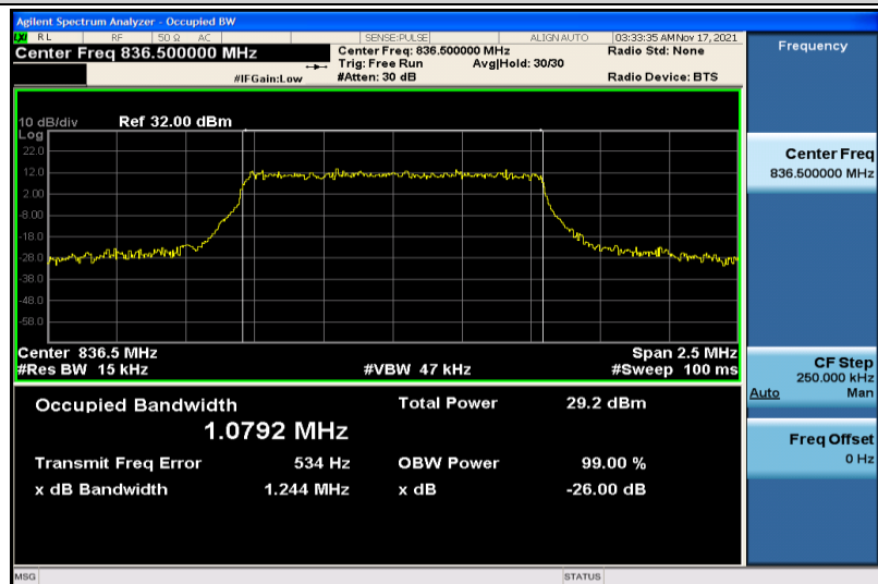
Band5-1.4MHz-16QAM-20525-6RB#0-1.0792
