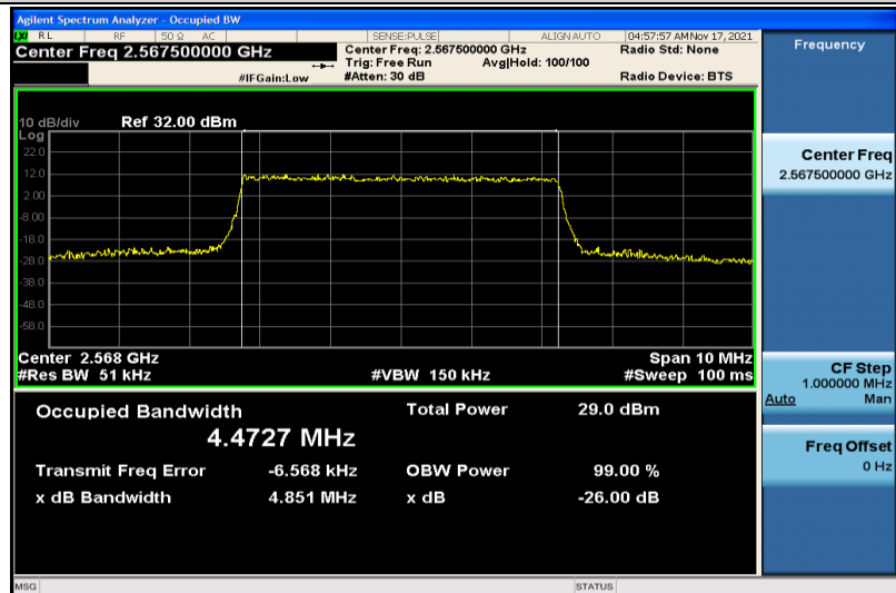
Band7-5MHz-QPSK-21425-25RB#0-4.4727
