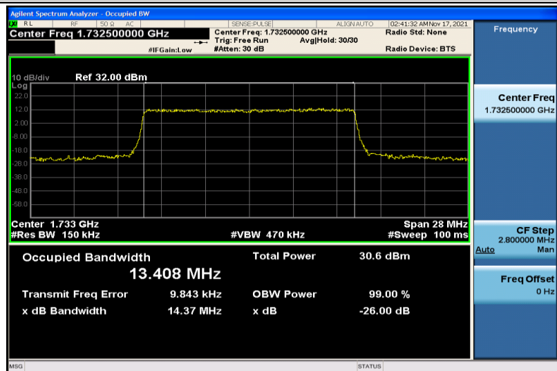
Band4-15MHz-QPSK-20175-75RB#0-13.408
