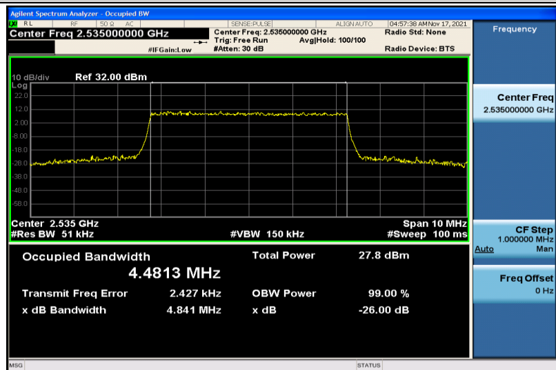
Band7-5MHz-16QAM-21100-25RB#0-4.4813
