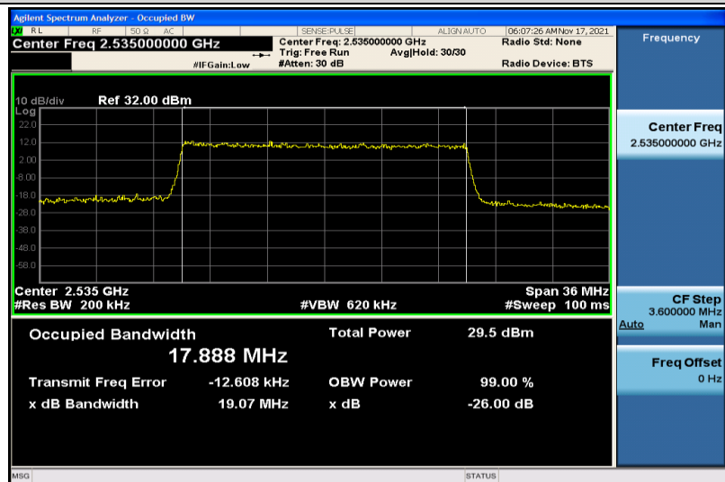
Band7-20MHz-QPSK-21100-100RB#0-17.888
