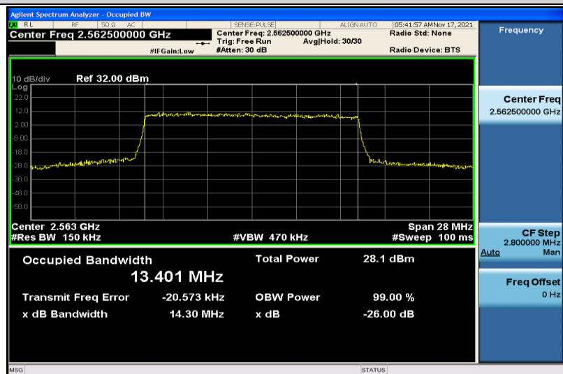
Band7-15MHz-16QAM-21375-75RB#0-13.401
