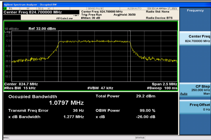
Band5-1.4MHz-16QAM-20407-6RB#0-1.0797
