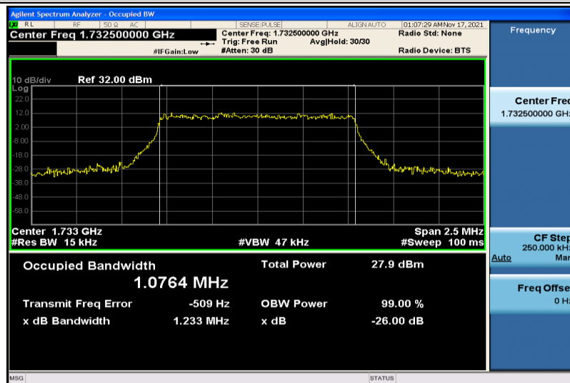
Band4-1.4MHz-16QAM-20175-6RB#0-1.0764
