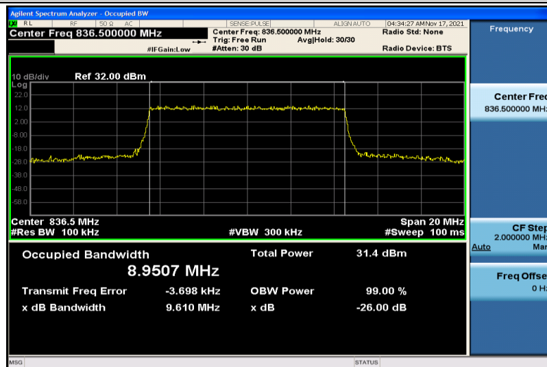
Band5-10MHz-QPSK-20525-50RB#0-8.9507
