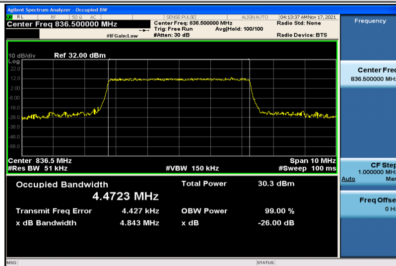
Band5-5MHz-16QAM-20525-25RB#0-4.4723
