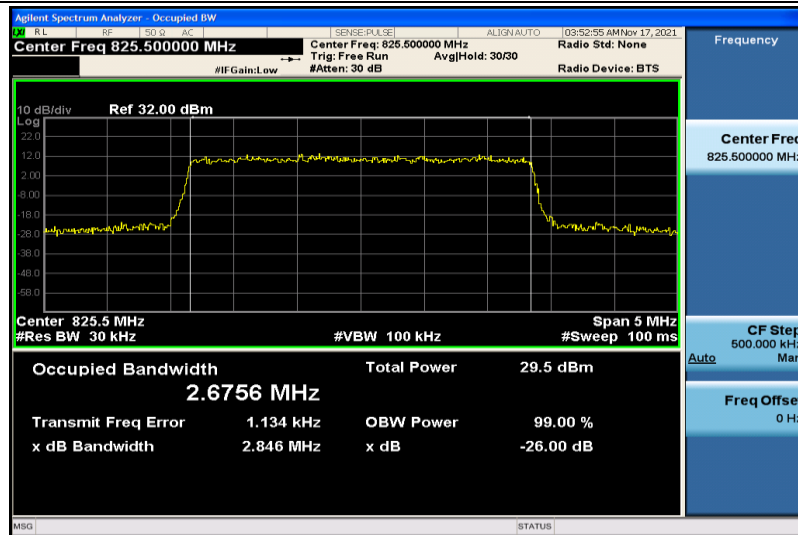
Band5-3MHz-16QAM-20415-15RB#0-2.6756
