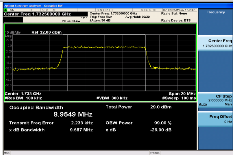
Band4-10MHz-16QAM-20175-50RB#0-8.9549
