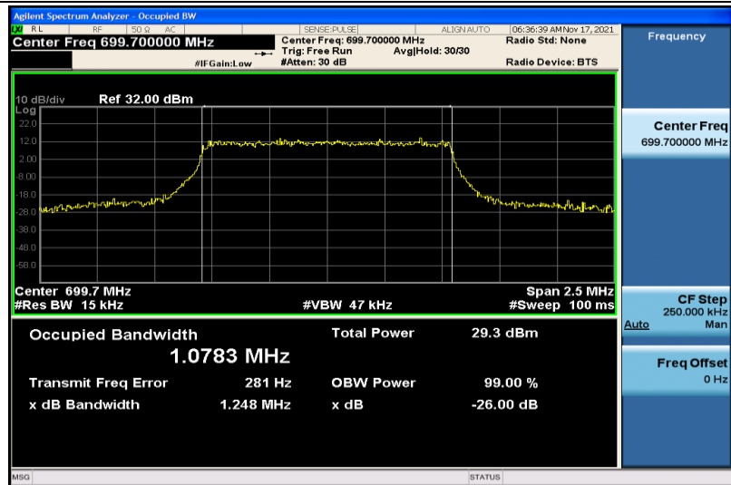
Band12-1.4MHz-16QAM-23017-6RB#0-1.0783
