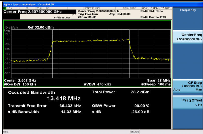
Band7-15MHz-16QAM-20825-75RB#0-13.418
