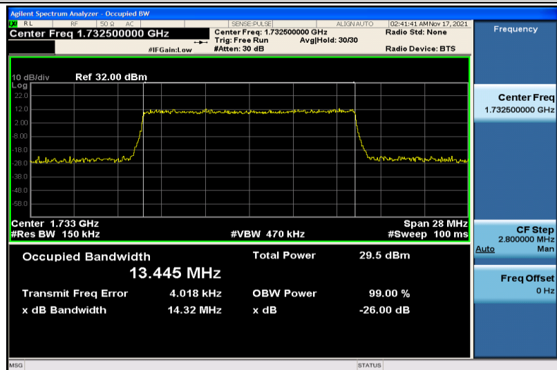
Band4-15MHz-16QAM-20175-75RB#0-13.445
