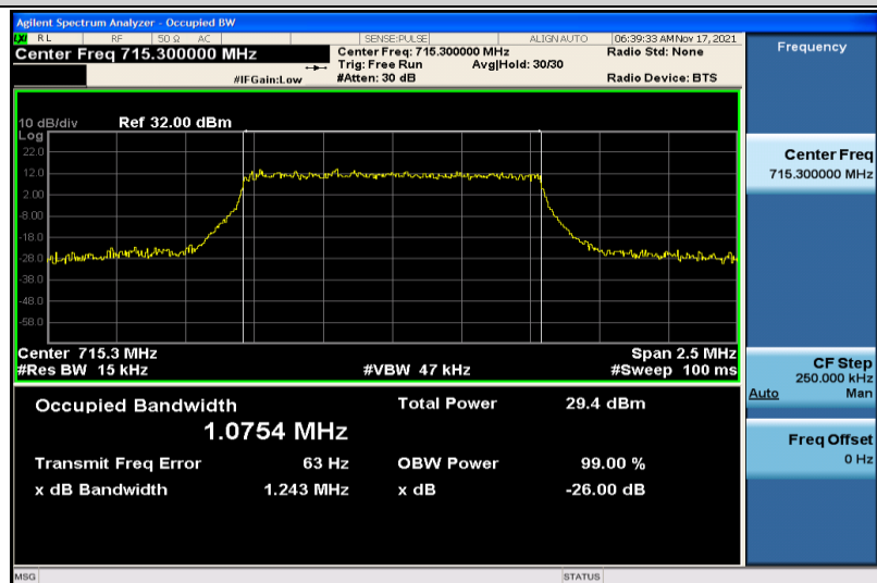
Band12-1.4MHz-16QAM-23173-6RB#0-1.0754
