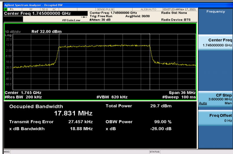
Band4-20MHz-16QAM-20300-100RB#0-17.831
