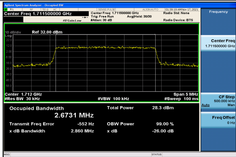
Band4-3MHz-16QAM-19965-15RB#0-2.6731
