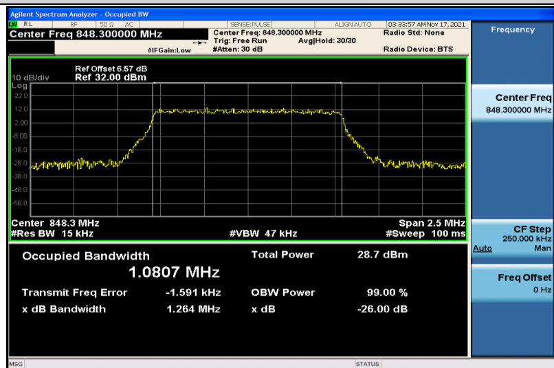
Band5-1.4MHz-16QAM-20643-6RB#0-1.0807
