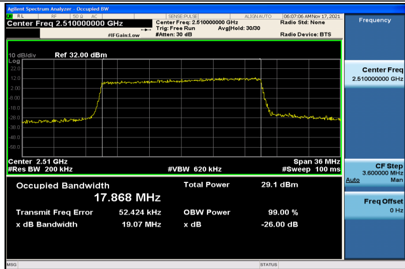
Band7-20MHz-QPSK-20850-100RB#0-17.868
