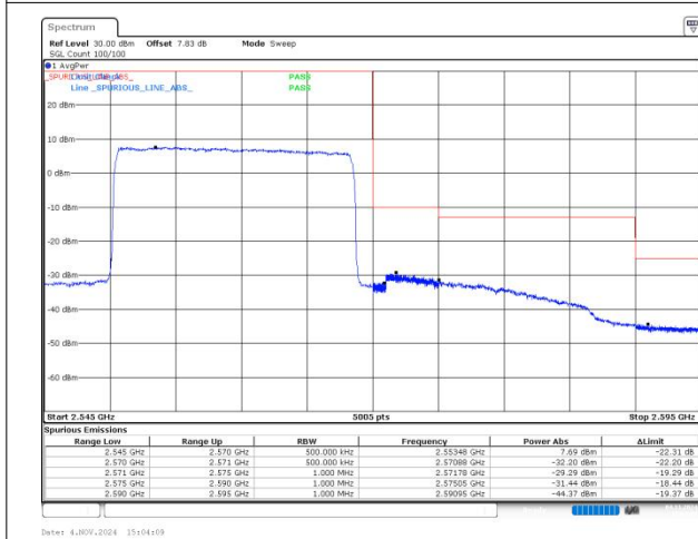
n7 SCS=15kHz DFT_QPSK BW=20MHz HighChannel=512000 RB=100@0
