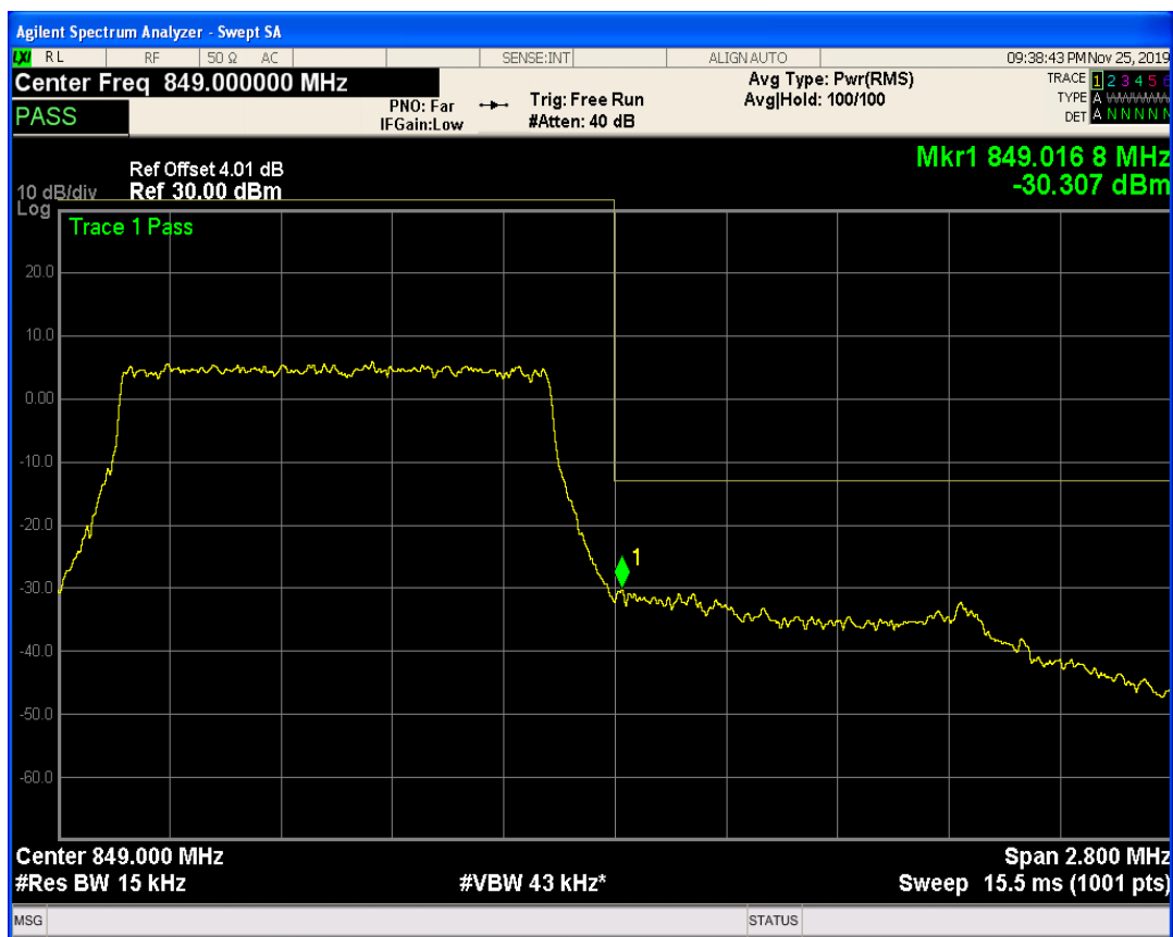
LTE Band5 QPSK BW=1.4MHz Channel=20643 RB Size=1 Position=#Max
