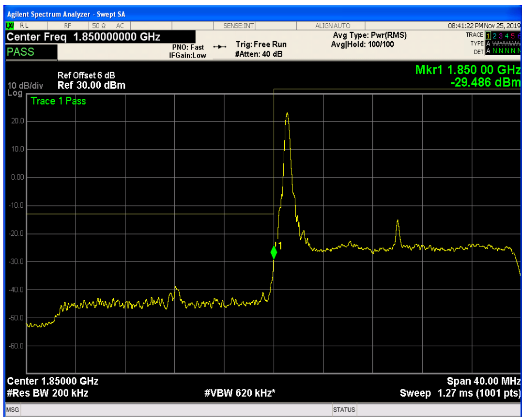
LTE Band2 QPSK BW=20MHz Channel=18700 RB Size=1 Position=#Max
