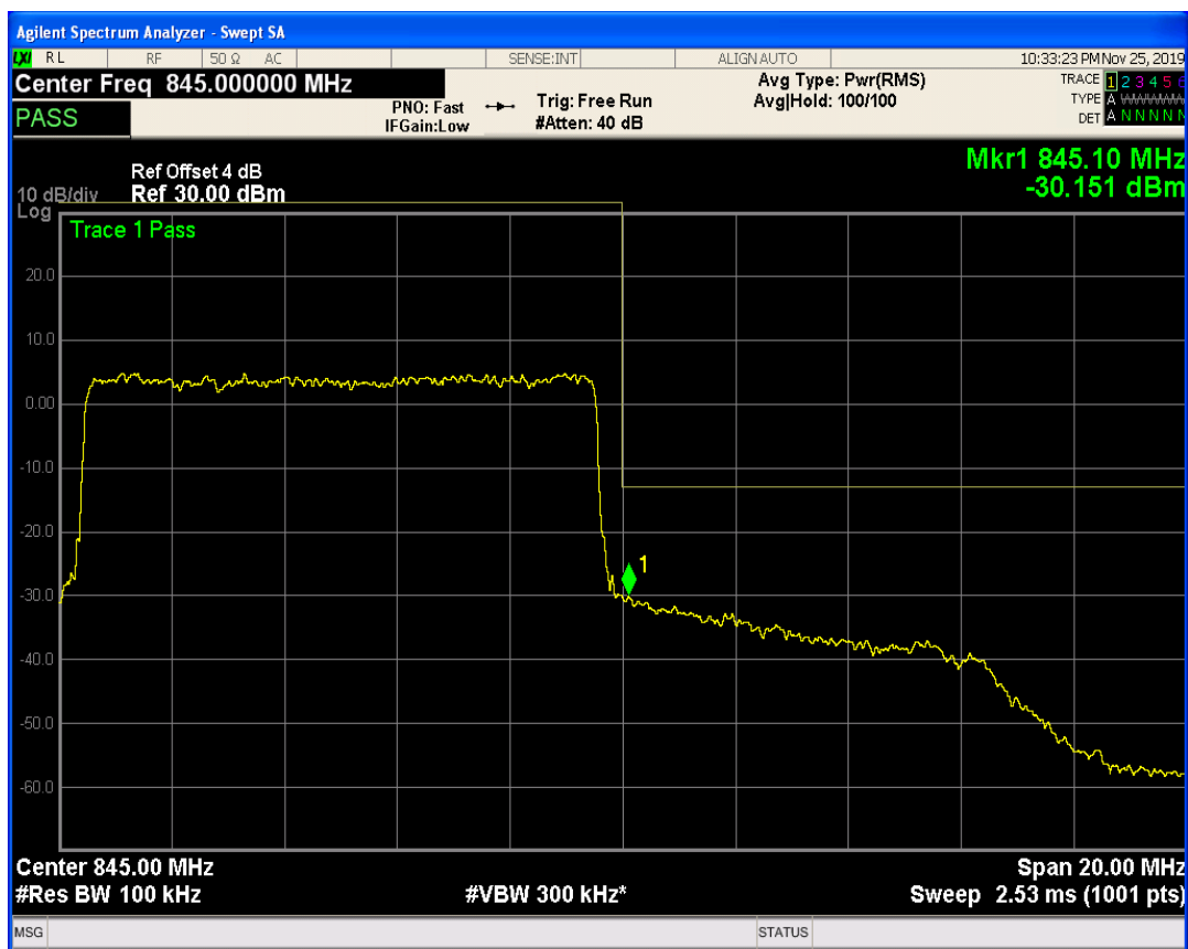
LTE Band19 QPSK BW=15MHz Channel=24075 RB Size=75 Position=#0
