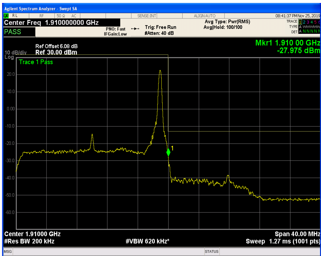
LTE Band2 QPSK BW=20MHz Channel=19100 RB Size=100 Position=#0
