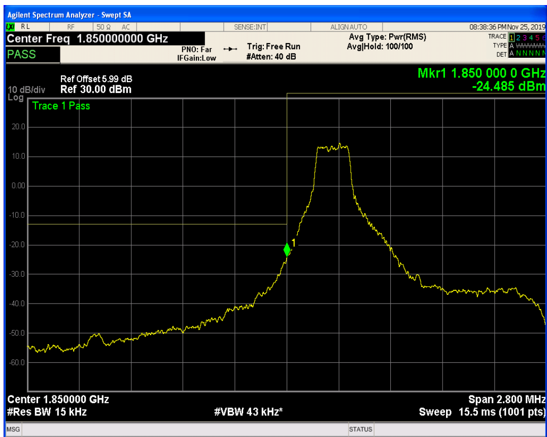
LTE Band2 QPSK BW=1.4MHz Channel=18607 RB Size=1 Position=#Max
