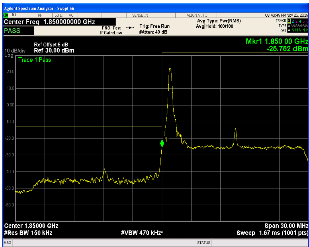
LTE Band2 QPSK BW=15MHz Channel=18675 RB Size=1 Position=#Max
