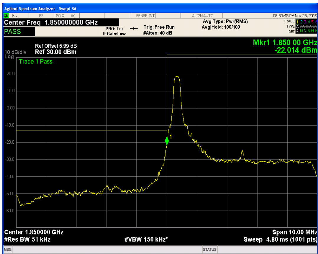
LTE Band2 QPSK BW=5MHz Channel=18625 RB Size=1 Position=#Max
