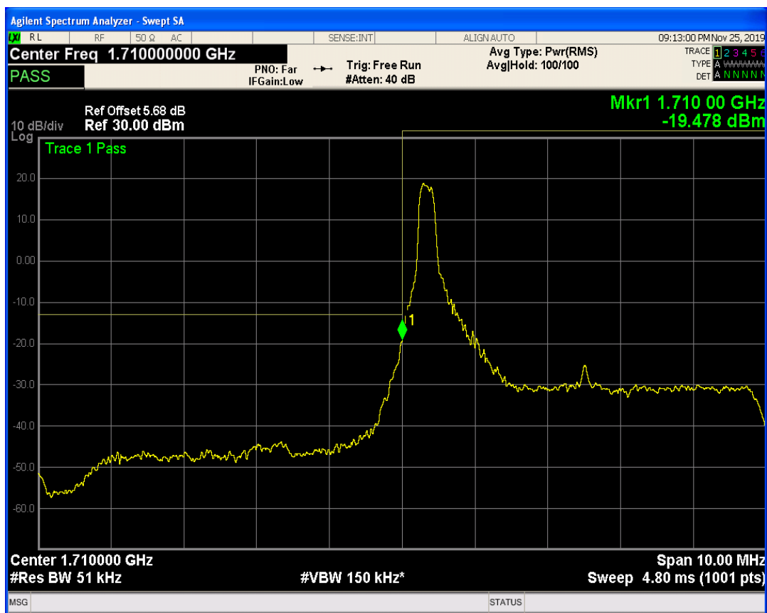
LTE Band4 QPSK BW=5MHz Channel=19975 RB Size=1 Position=#Max
