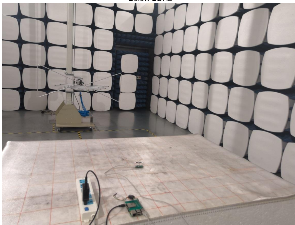
Radiated Spurious Emission(for External ANT B) Below 1GHz
