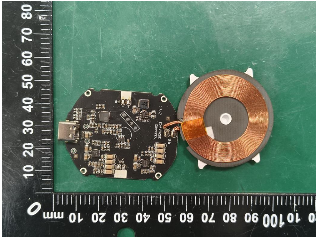
Figure 7 Top PCB view
