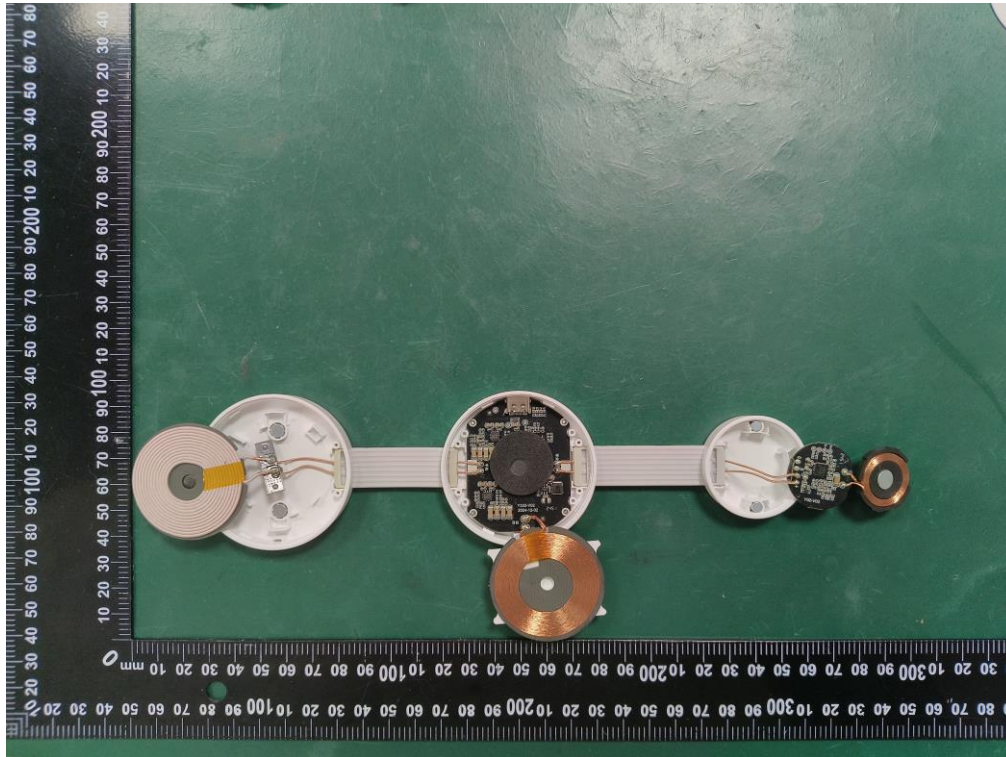
Figure 3 Internal view for model Y333
