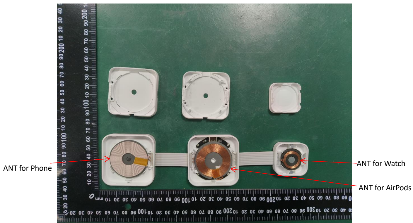
Figure 5 Internal view for model Y222
