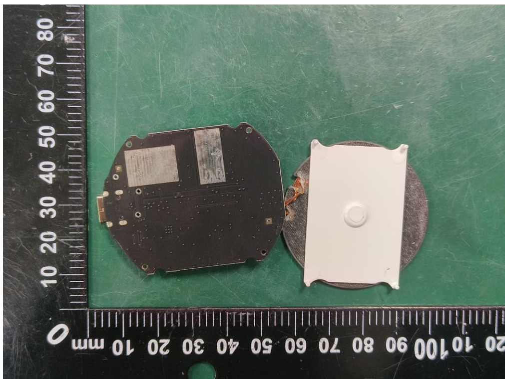
Figure 8 Bottom PCB view
