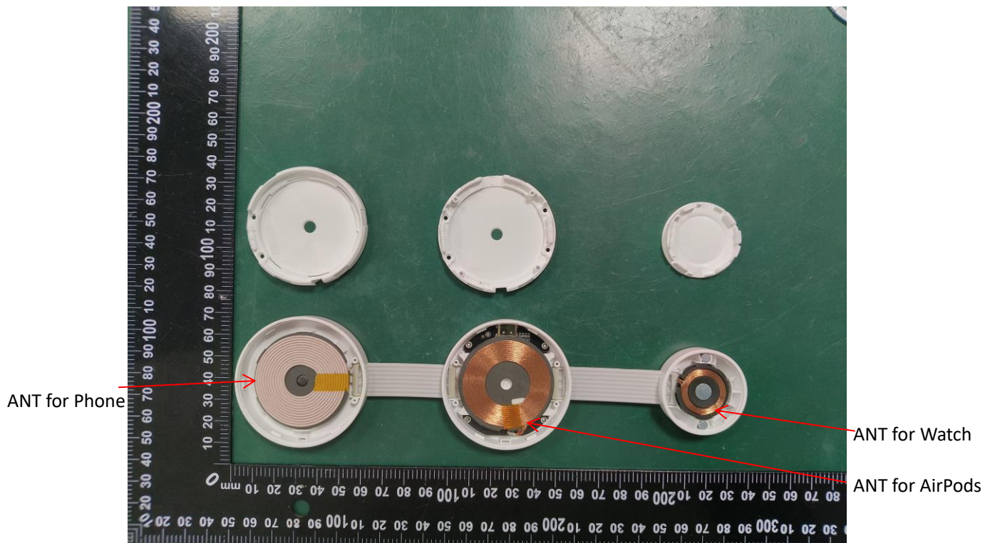
Figure 2 Internal view for model Y333
