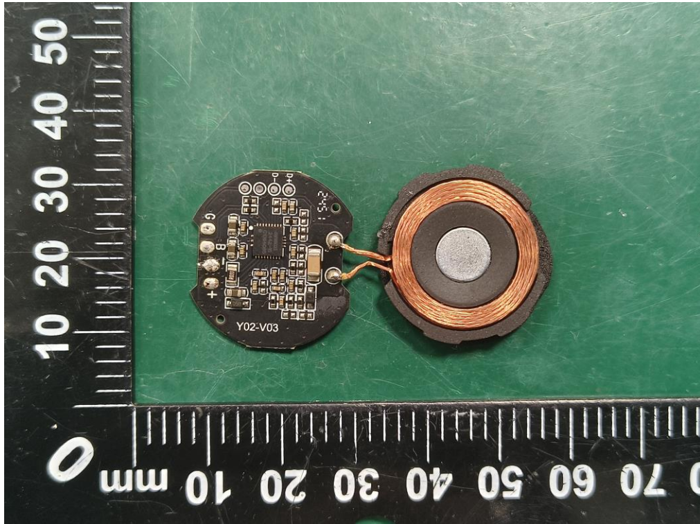
Figure 9 Top PCB view
