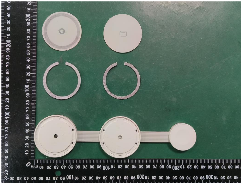
Figure 1 Internal view for model Y333
