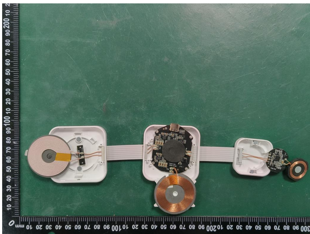
Figure 6 Internal view for model Y222
