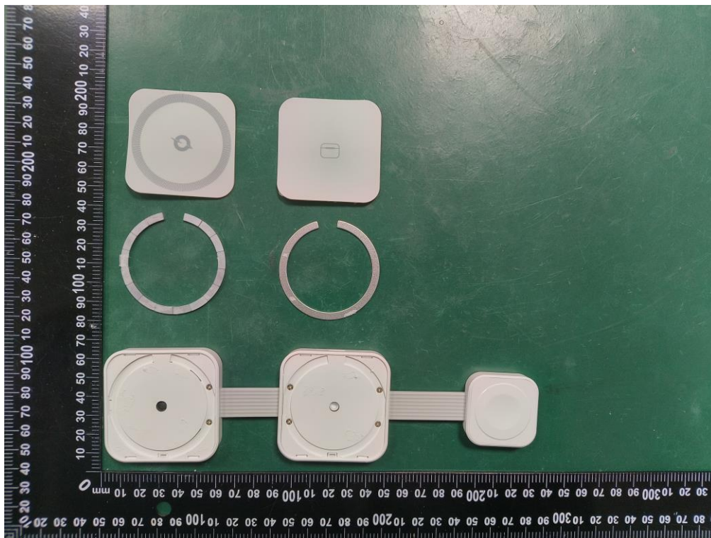
Figure 4 Internal view for model Y222
