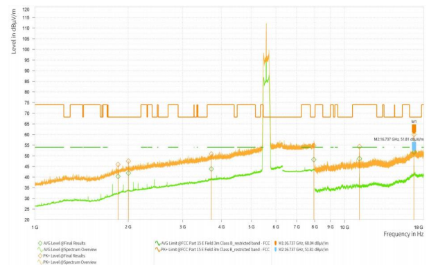
Wi-Fi 5G_11A_5580_High
