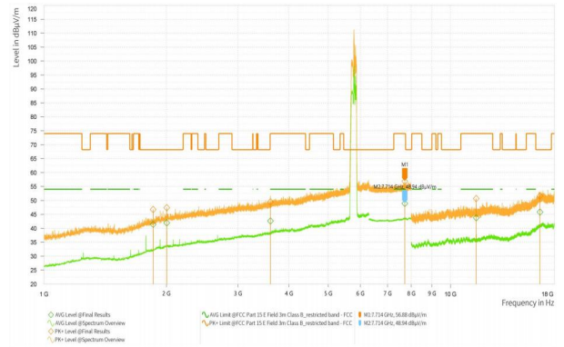
Wi-Fi 5G_11N40_5190_High
