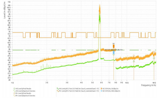
Wi-Fi 5G_11AC20_5180_High
