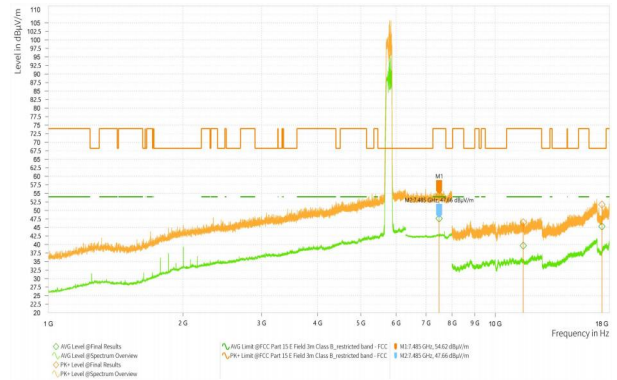
Wi-Fi 5G_11AC80_5775_High
