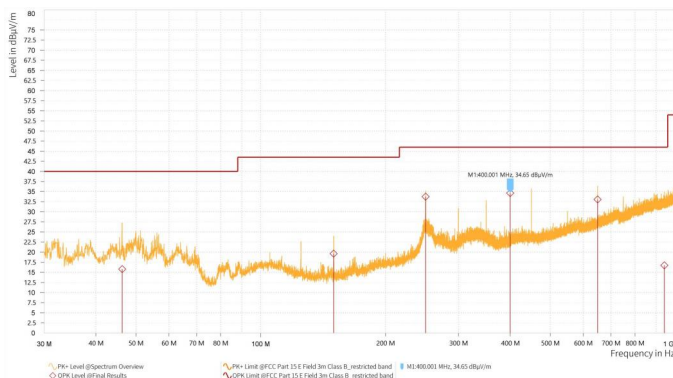
Wi-Fi 5G_11A_5260_Low
