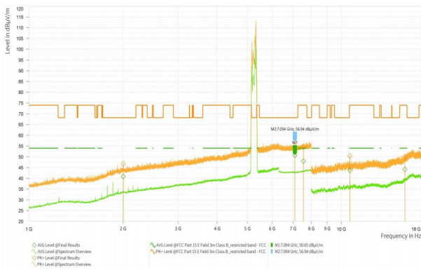
Wi-Fi 5G_11AC20_5580_High
