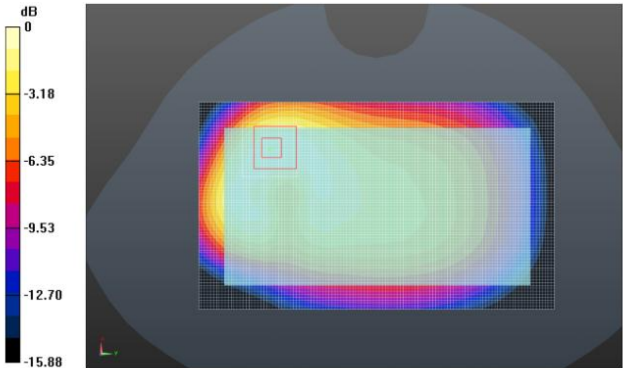
Rear Side (GSM850 GPRS 4TS Middle Channel)
