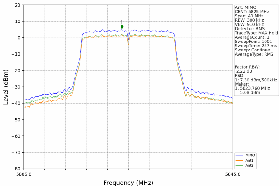
802.11ac(VHT20)_HCH_5825MHz_MIMO_NTNV
