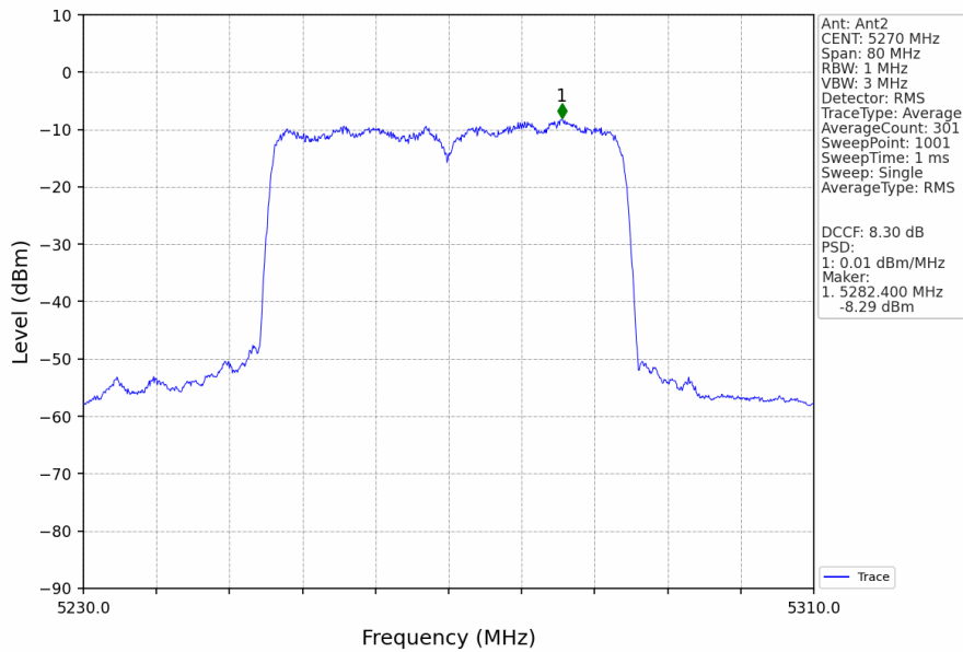
802.11ax(HEW40)_LCH_5270MHz_RU484_Left_MIMO_NTNV
