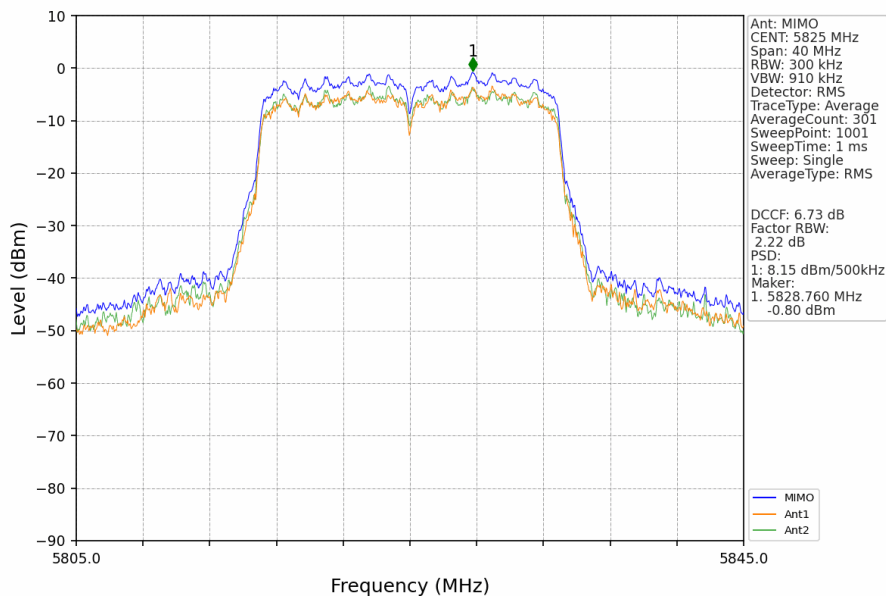
802.11ax(HEW20)_HCH_5825MHz_RU242_Left_MIMO_NTNV
