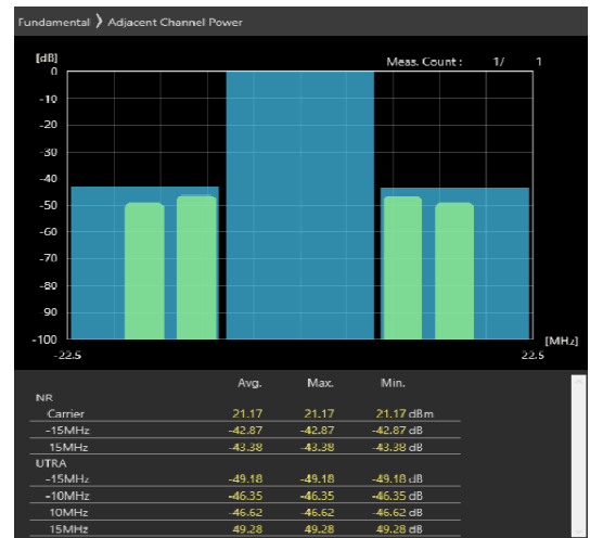
15MHz_30kHz_3692.5MHz-OFDM QPSK_RB36@0 -42.87,-43.38dB
