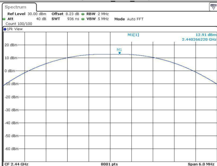
2.4G custom_Ant2_2440
