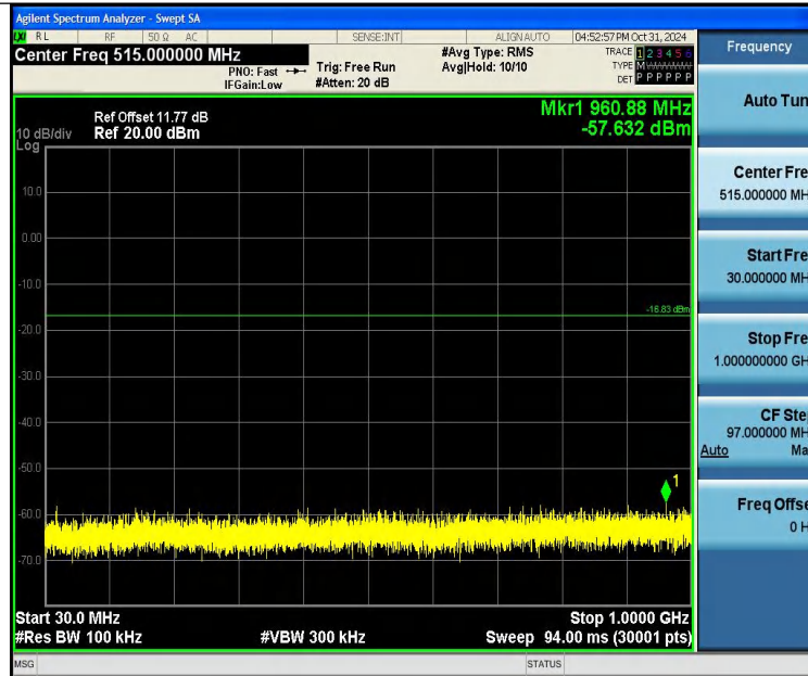
BLE_1M-Ant1-2440-30~1000-PASS
