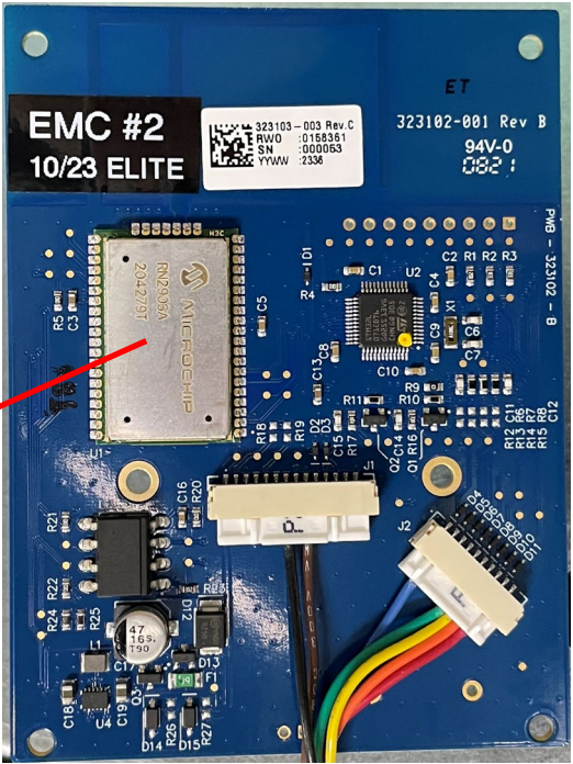
Endpoint PlumbSMART Board w/LoRa transceiver and antenna
