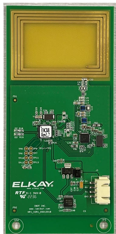
Filter NFC Board w/NFC transceiver and antenna
