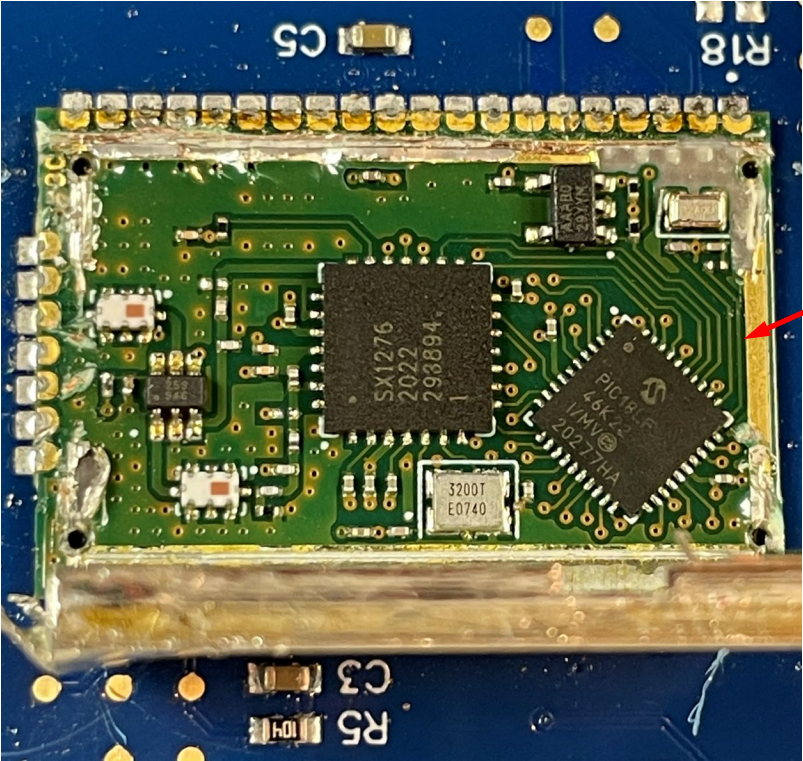
Endpoint PlumbSMART Board w/LoRa transceiver and antenna
