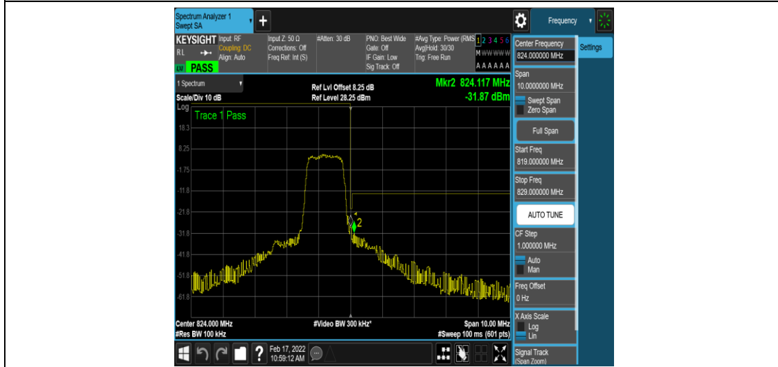
Band26-5MHz-16QAM-26765-6-0-High--29.02,-31.87-PASS
