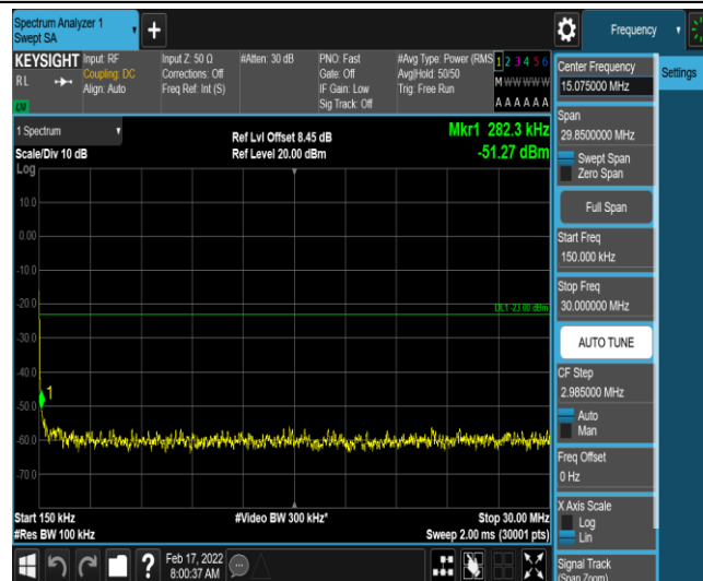
Band26-1.4MHz-16QAM-26697-1-0-Low-0.15-30--51.27-PASS
