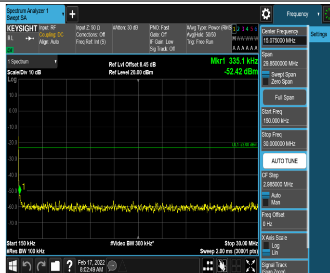
Band26-1.4MHz-QPSK-26740-1-0-Low-0.15-30--52.42-PASS
