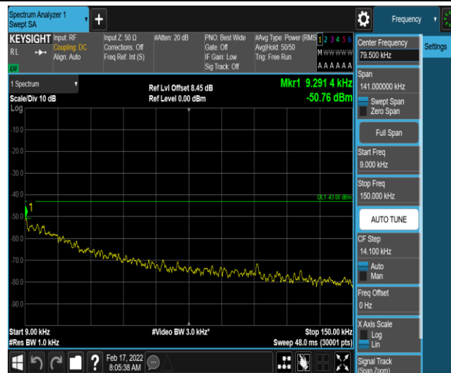
Band26-1.4MHz-QPSK-26783-1-0-High-0.009-0.15--50.77-PASS
