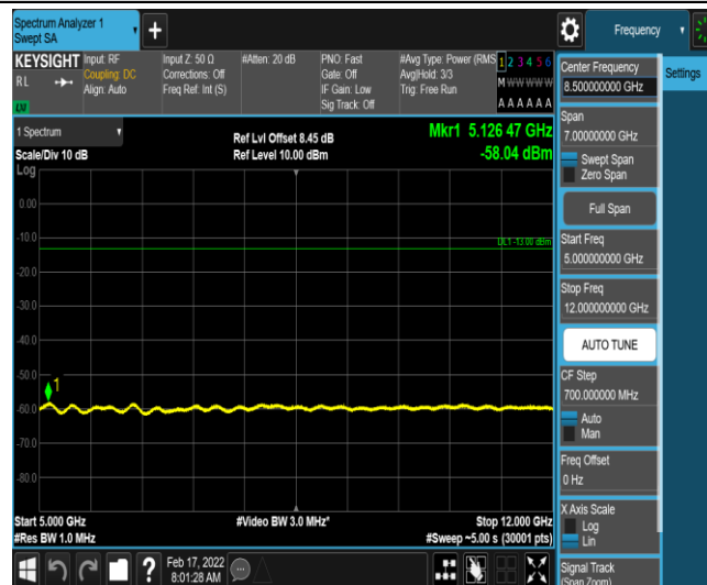
Band26-1.4MHz-16QAM-26697-1-0-Low-5000-12000--58.04-PASS
