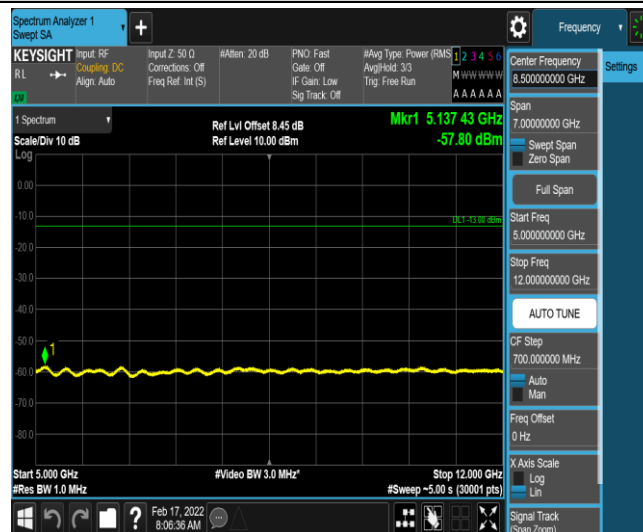
Band26-1.4MHz-QPSK-26783-1-0-High-5000-12000--57.8-PASS
