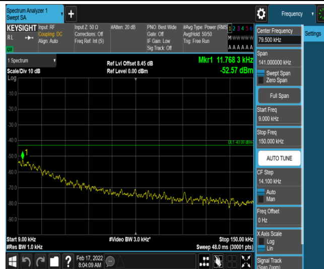
Band26-1.4MHz-16QAM-26740-1-0-Low-0.009-0.15--52.57-PASS
