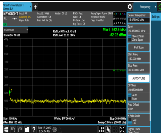
Band26-1.4MHz-16QAM-26740-1-0-Low-0.15-30--52.02-PASS
