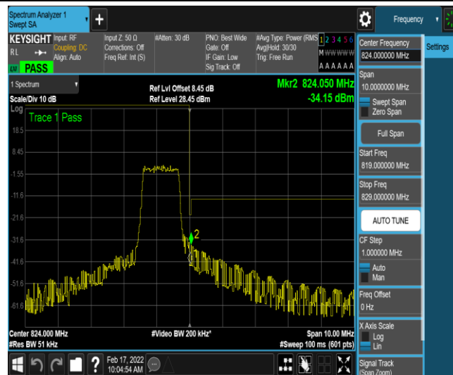
Band26-3MHz-16QAM-26775-6-0-High--42.84,-34.15-PASS
