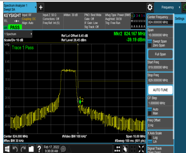
Band26-1.4MHz-16QAM-26783-6-0-High--37.30,-39.19-PASS
