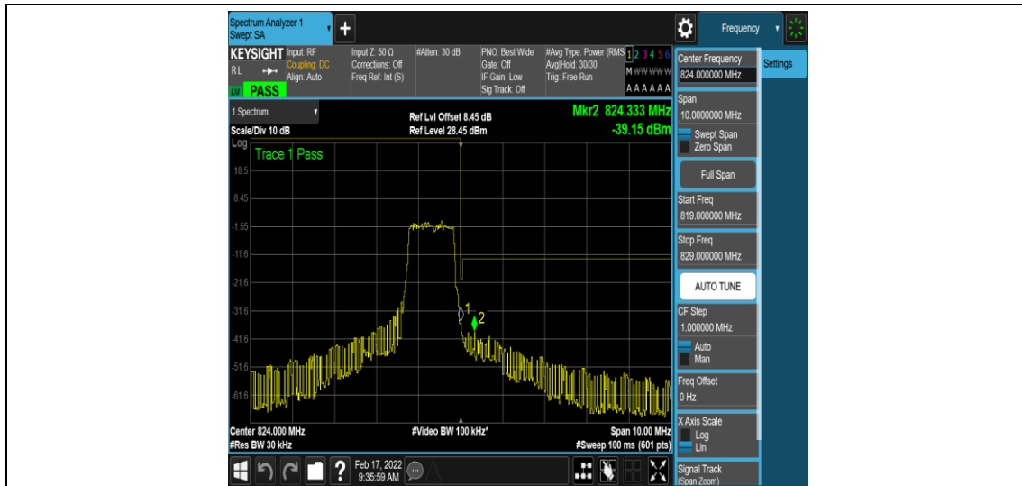
Band26-1.4MHz-QPSK-26783-6-0-High--35.90,-39.15-PASS
