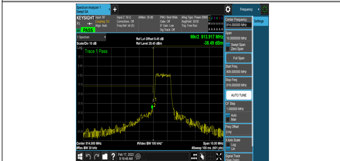
Band26-1.4MHz-16QAM-26697-6-0-Low--32.48,-38.49-PASS
