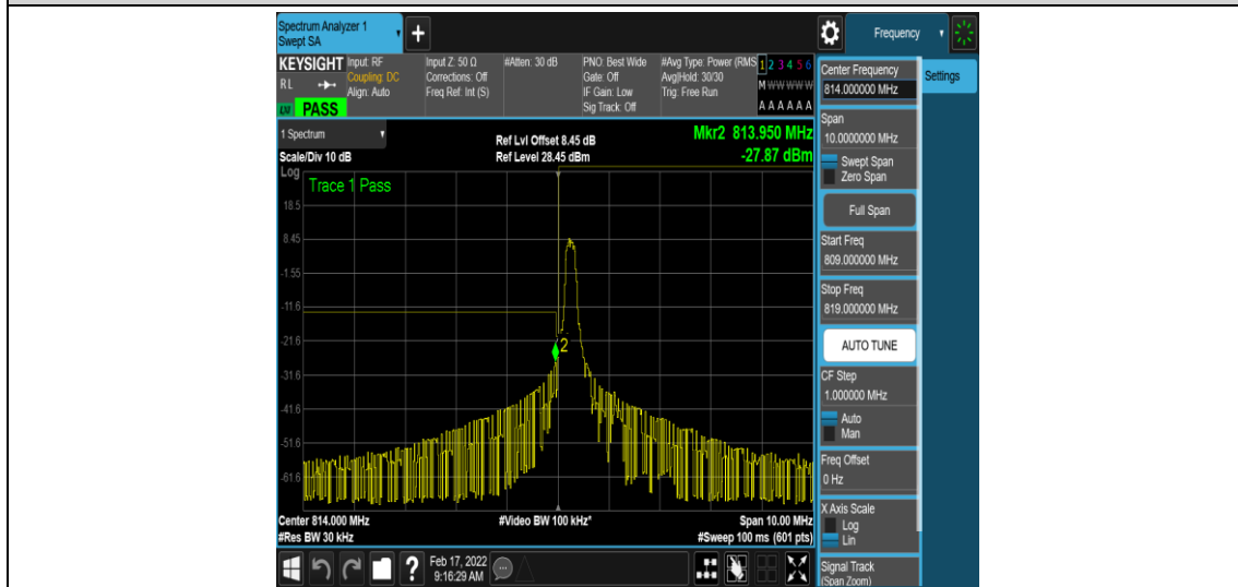
Band26-1.4MHz-16QAM-26697-1-0-Low--26.38,-27.87-PASS
