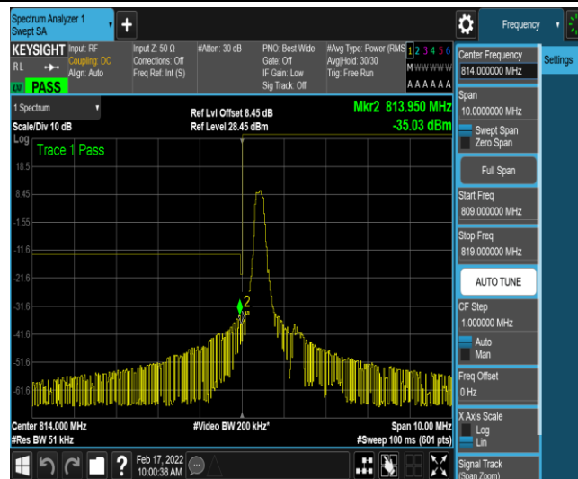
Band26-3MHz-16QAM-26705-1-0-Low--38.05,-35.03-PASS
