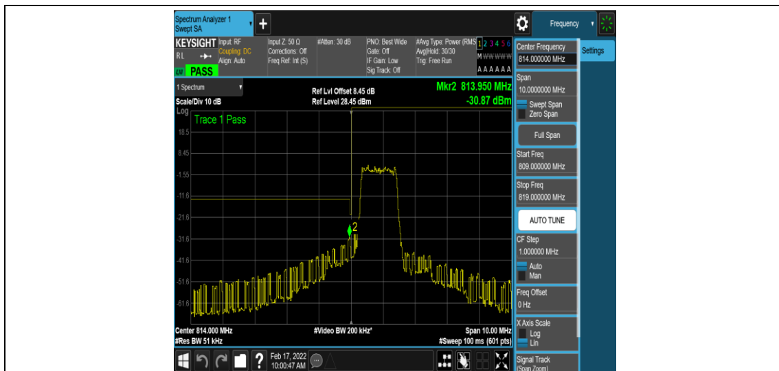
Band26-3MHz-QPSK-26705-6-0-Low--30.76,-30.87-PASS
