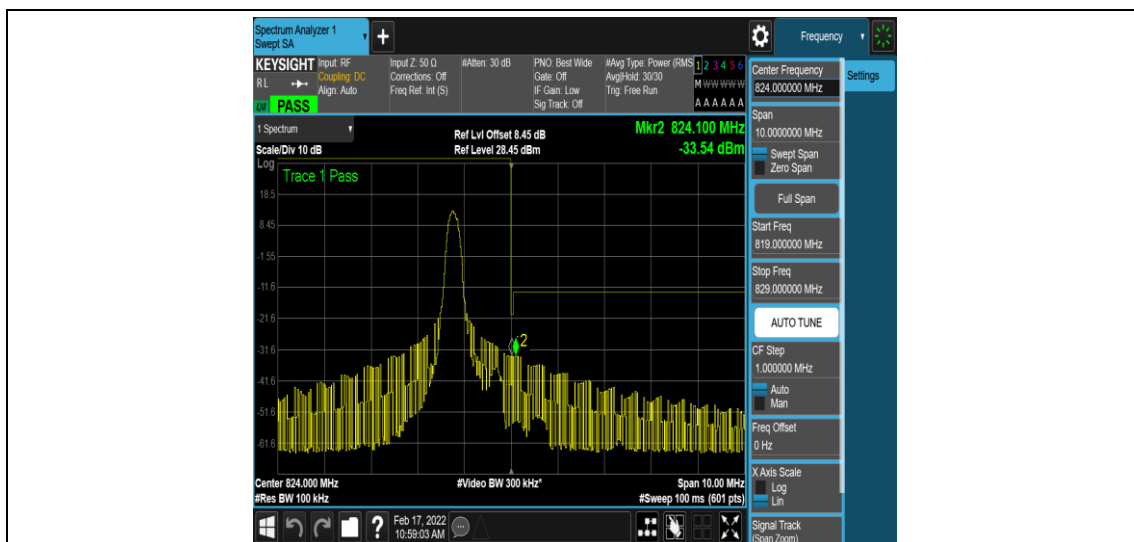
Band26-5MHz-QPSK-26765-1-0-High--33.74,-33.54-PASS
