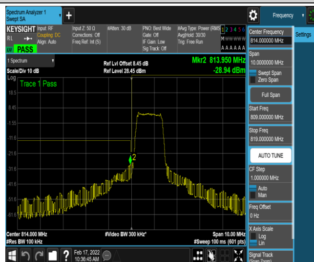
Band26-5MHz-QPSK-26715-6-0-Low--28.49,-28.94-PASS
