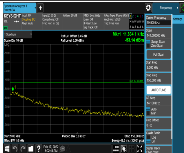
Band26-1.4MHz-QPSK-26740-1-0-Low-0.009-0.15--53.14-PASS
