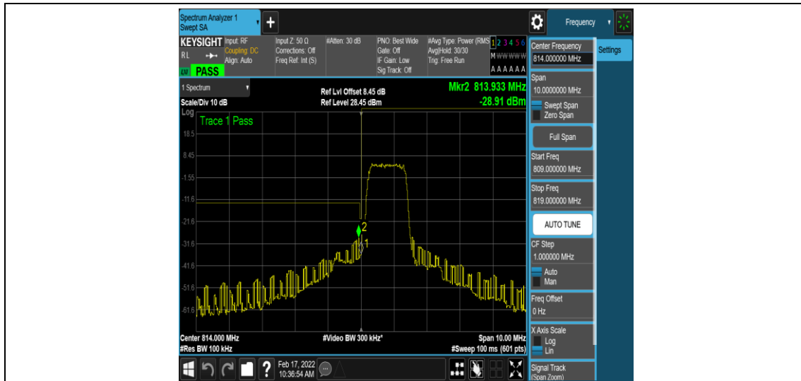
Band26-5MHz-16QAM-26715-6-0-Low--36.50,-28.91-PASS
