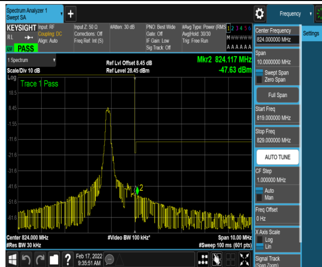
Band26-1.4MHz-16QAM-26783-1-0-High--47.26,-47.63-PASS
