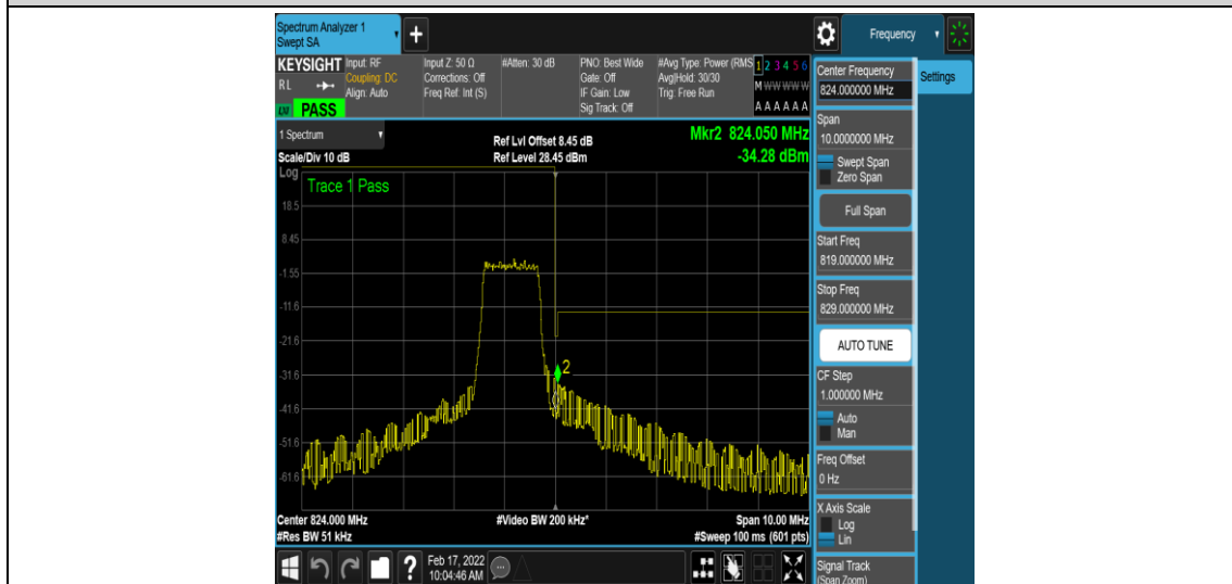
Band26-3MHz-QPSK-26775-6-0-High--42.03,-34.28-PASS
