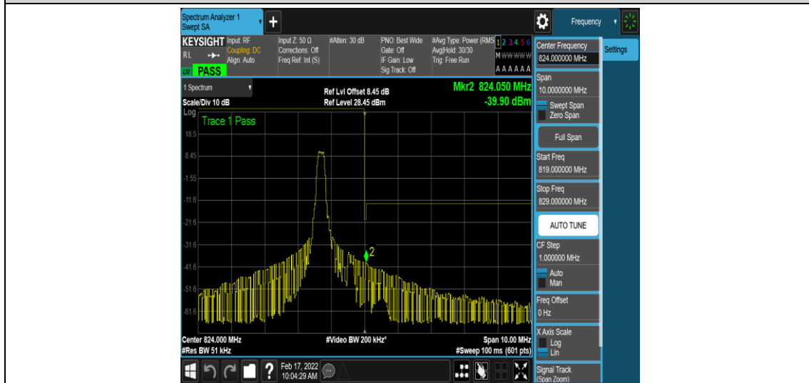
Band26-3MHz-QPSK-26775-1-0-High--39.91,-39.90-PASS
