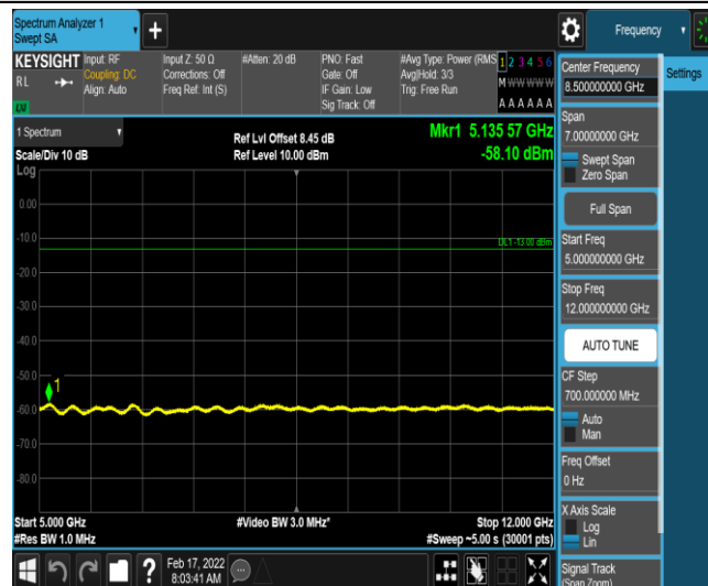
Band26-1.4MHz-QPSK-26740-1-0-Low-5000-12000--58.1-PASS
