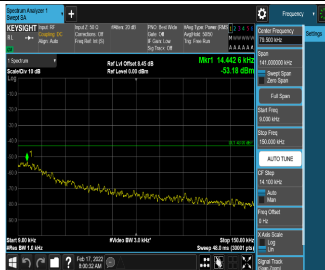
Band26-1.4MHz-16QAM-26697-1-0-Low-0.009-0.15--53.18-PASS
