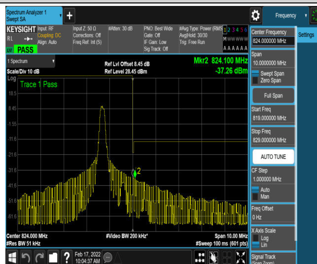
Band26-3MHz-16QAM-26775-1-0-High--36.51,-37.26-PASS
