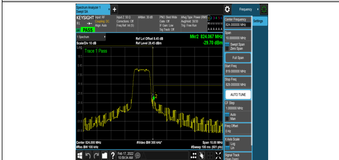
Band26-5MHz-16QAM-26765-6-0-High--27.55,-29.70-PASS
