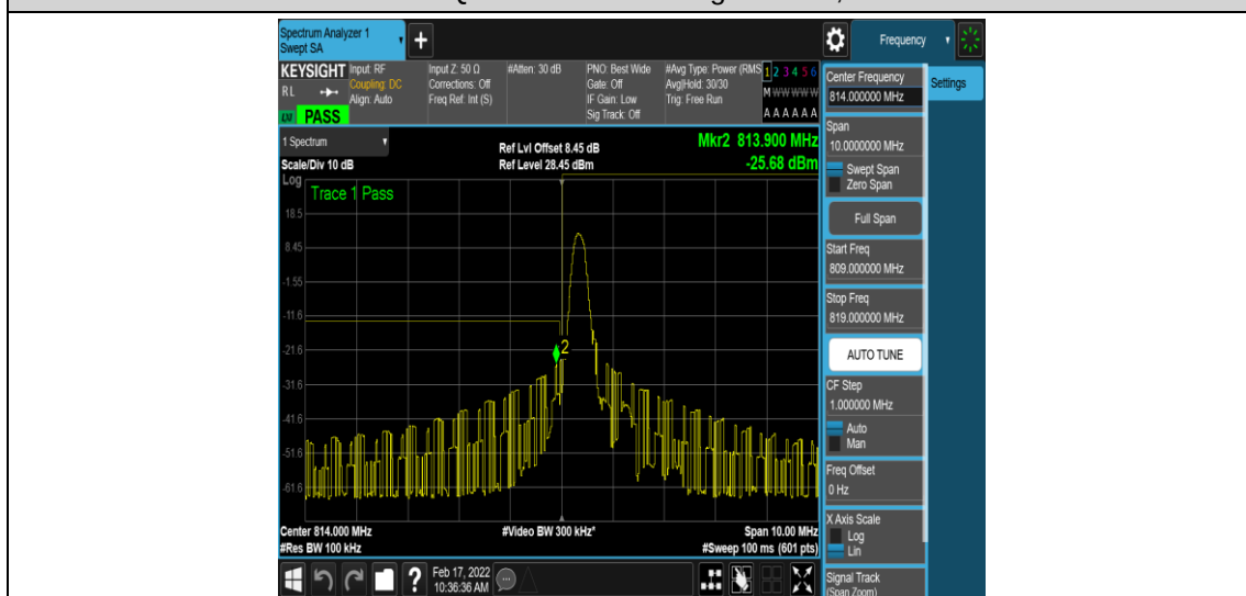
Band26-5MHz-16QAM-26715-1-0-Low--24.48,-25.68-PASS
