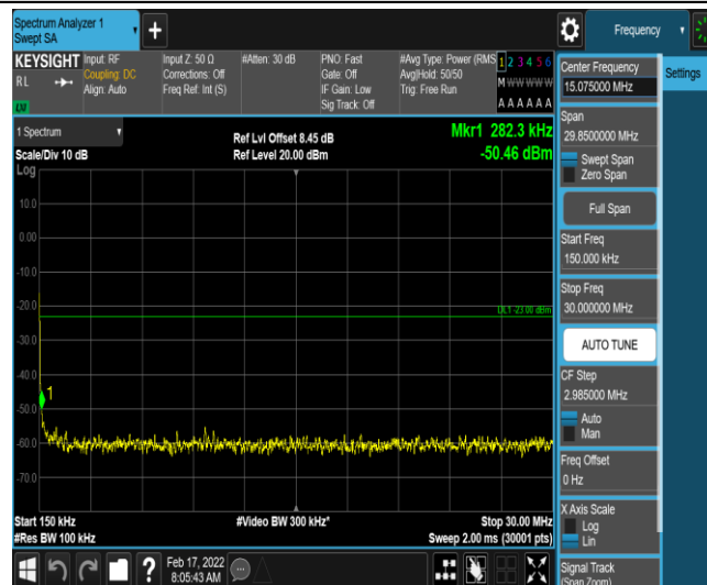
Band26-1.4MHz-QPSK-26783-1-0-High-0.15-30--50.46-PASS
