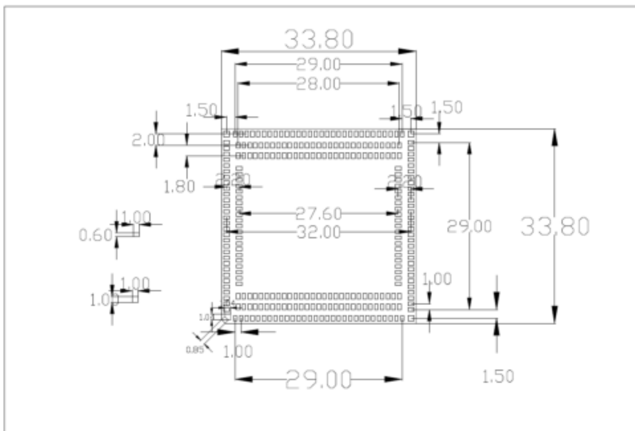
Figure 5-4 package dimensions
