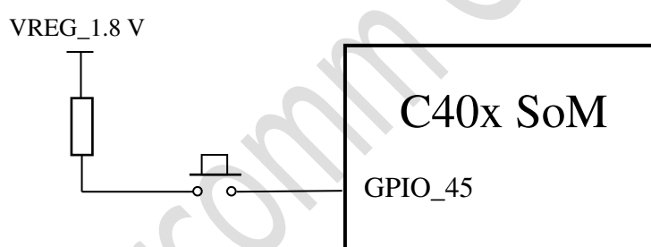
Figure 3-4Power on signal
