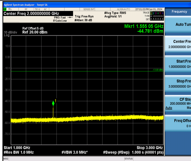
Band13_10MHz_QPSK_23230_1RB#0_1000~3000_1000~3000
