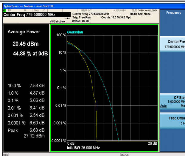
Band13-5MHz-16QAM-23205-1RB#0-PASS
