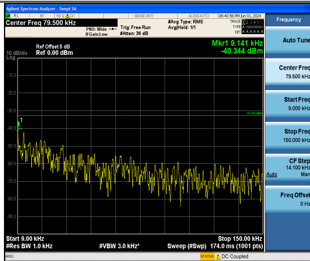
Band13_5MHz_16QAM_23255_1RB#0_0.009~0.15_0.009~0.15
