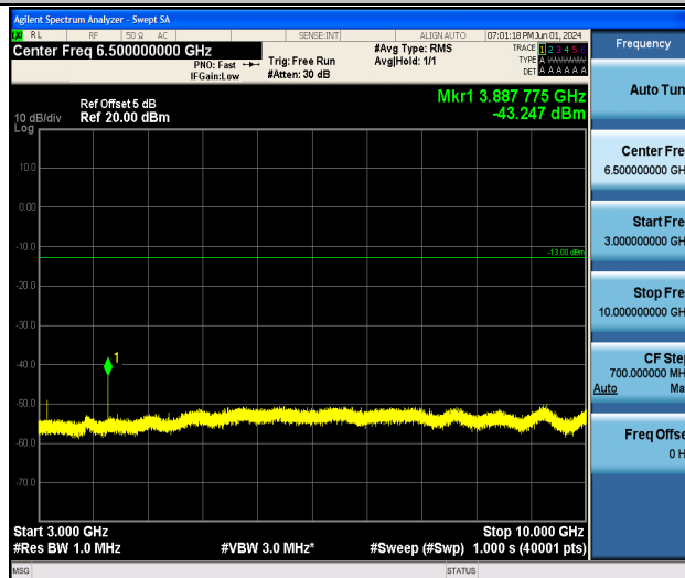
Band13_10MHz_QPSK_23230_1RB#0_3000~10000_3000~10000
