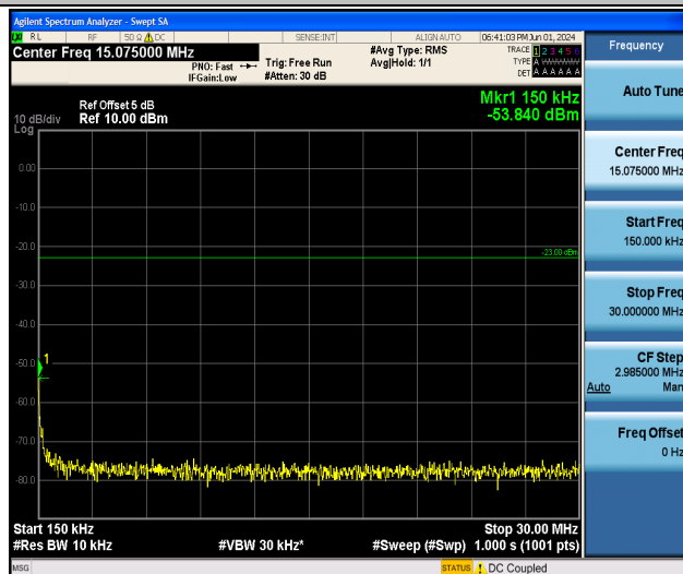
Band13_5MHz_16QAM_23255_1RB#0_0.15~30_0.15~30
