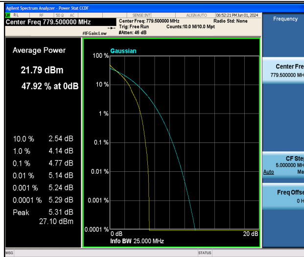
Band13-5MHz-QPSK-23205-1RB#0-PASS
