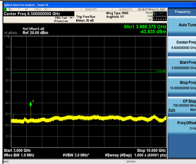
Band13_5MHz_16QAM_23205_1RB#0_3000~10000_3000~10000
