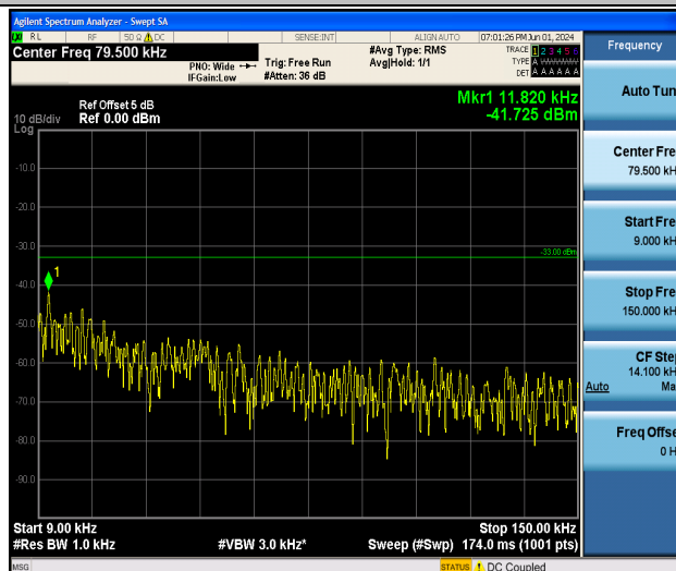
Band13_10MHz_16QAM_23230_1RB#0_0.009~0.15_0.009~0.15
