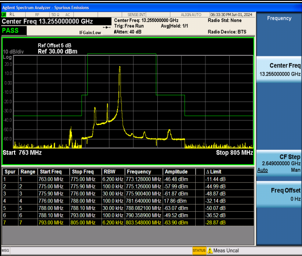
Band13_5MHz_QPSK_23205_1RB#24
