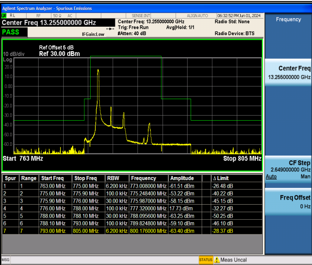
Band13_5MHz_QPSK_23205_1RB#0
