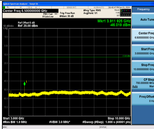
Band13_5MHz_QPSK_23255_1RB#0_3000~10000_3000~10000
