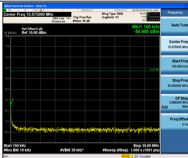
Band13_5MHz_QPSK_23230_1RB#0_0.15~30_0.15~30
