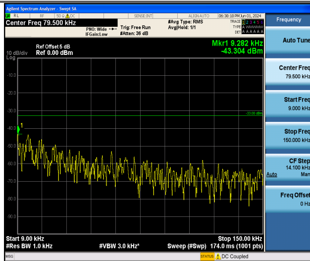
Band13_5MHz_QPSK_23230_1RB#0_0.009~0.15_0.009~0.15
