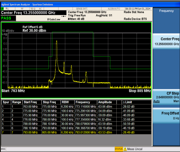
Band13_5MHz_16QAM_23205_1RB#0
