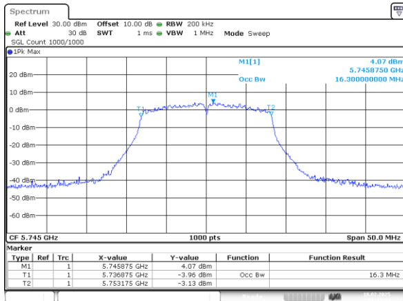
802.11a_5745MHz
