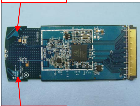
Printed antenna
