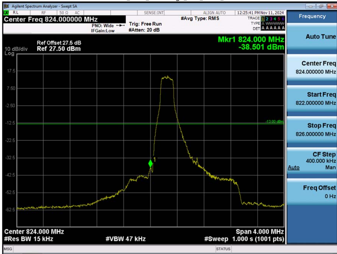
LTE B5_1.4M_Band Edge_Low_QPSK_1RB
