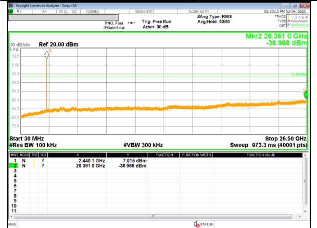
OUT-OF-BAND MIDDLE(17) CHANNEL
