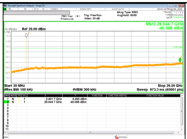
OUT-OF-BAND LOW(37) CHANNEL
