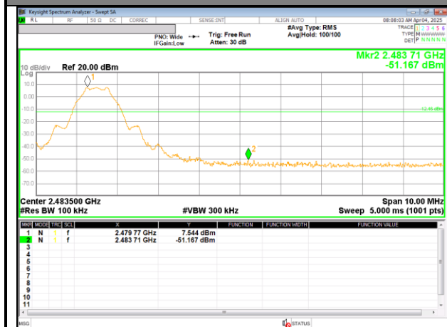
HIGH(39) CHANNEL BANDEDGE
