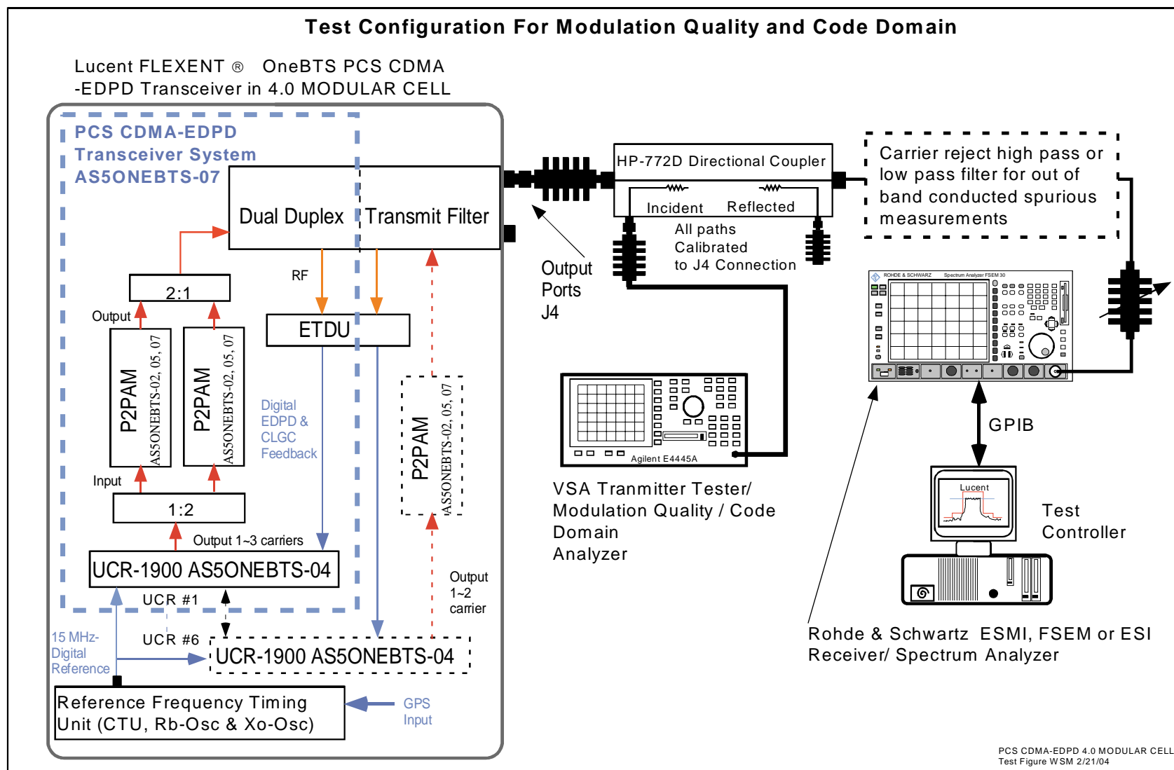
Figure 13 Modulation Quality Measurement
