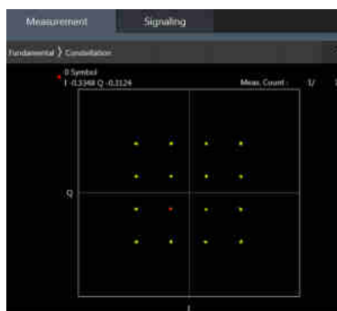
16QAM
