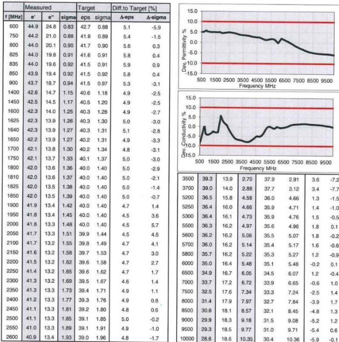
Figure D-2 600 – 10000 MHz Head Tissue Equivalent Matter
