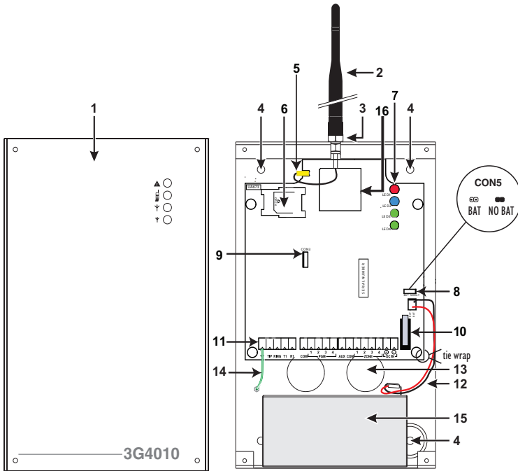
Figure 1 - Parts
