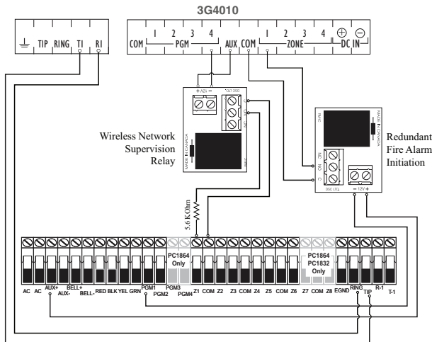
Figure 8 -Connection Details for Wireless Network Supervision Relay and Redundant Fire Alarm Trans- mission
