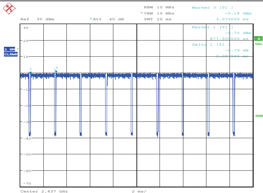
Test Graph_IEEE802.11g Duty Cycle:
