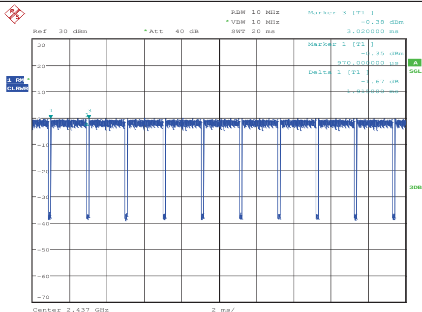
Test Graph_IEEE802.11 n (HT20) Duty Cycle:
