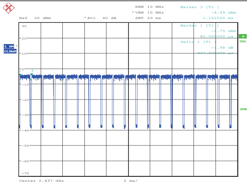
Test Graph_IEEE802.11 n (HT40) Duty Cycle:
