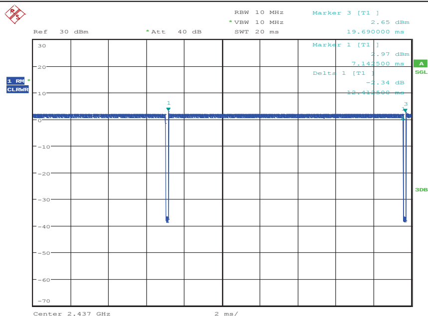
Test Graph_IEEE802.11b Duty Cycle:
