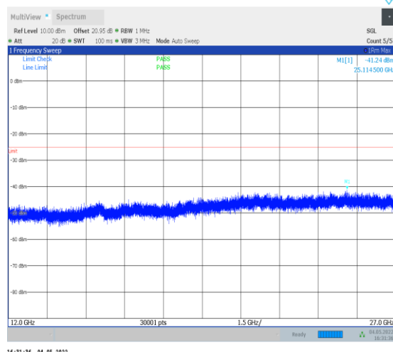
1-N41--30-100-L-1-DFT-PI2BPSK-Inner_1RB_Left-1 @1-12000-27000-Ant0--41.24--25-PASS
