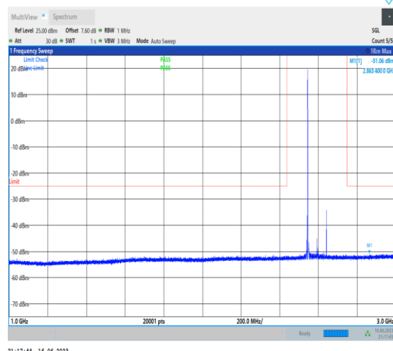
1-N41-PC1-30-100-M-1-DFT-QPSK-Edge_1RB_Left- 1@0-1000-3000-Ant0-2863.40--51.06--25-PASS
