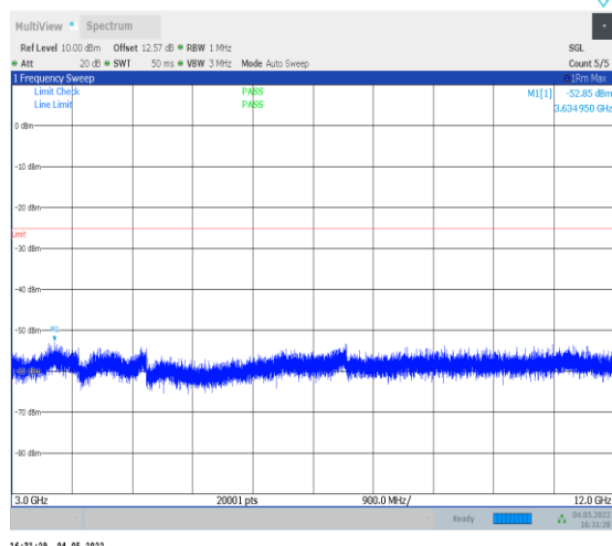
1-N41--30-100-L-1-DFT-PI2BPSK-Inner_1RB_Left-1 @1-3000-12000-Ant0--52.85--25-PASS
