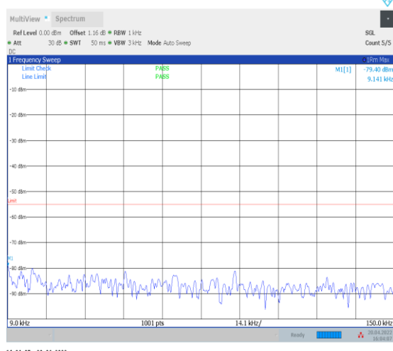
1-N41--30-100-M-1-DFT-PI2BPSK-Inner_1RB_Left-1 @1-0.009-0.15-Ant0--79.40--55-PASS
