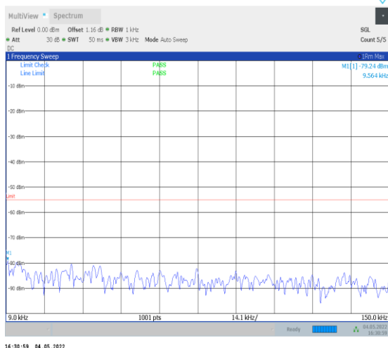
1-N41--30-100-L-1-DFT-PI2BPSK-Inner_1RB_Left-1 @1-0.009-0.15-Ant0--79.24--55-PASS
