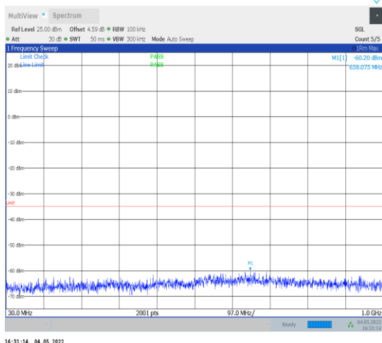
1-N41--30-100-L-1-DFT-PI2BPSK-Inner_1RB_Left-1 @1-30-1000-Ant0--60.20--35-PASS
