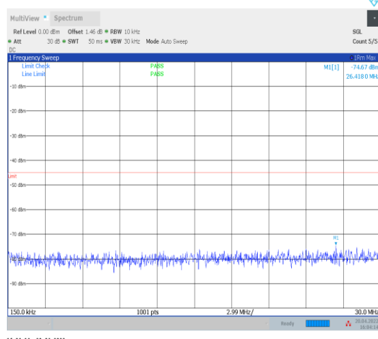
1-N41--30-100-M-1-DFT-PI2BPSK-Inner_1RB_Left-1 @1-0.15-30-Ant0--74.67--45-PASS
