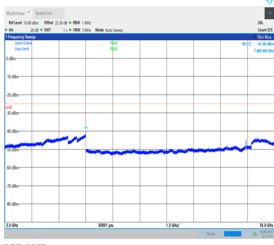
1-N41-PC1-30-100-M-1-DFT-QPSK-Edge_1RB_Left -1@0-3000-18000-Ant0-7495.50--41.44--25-PASS
