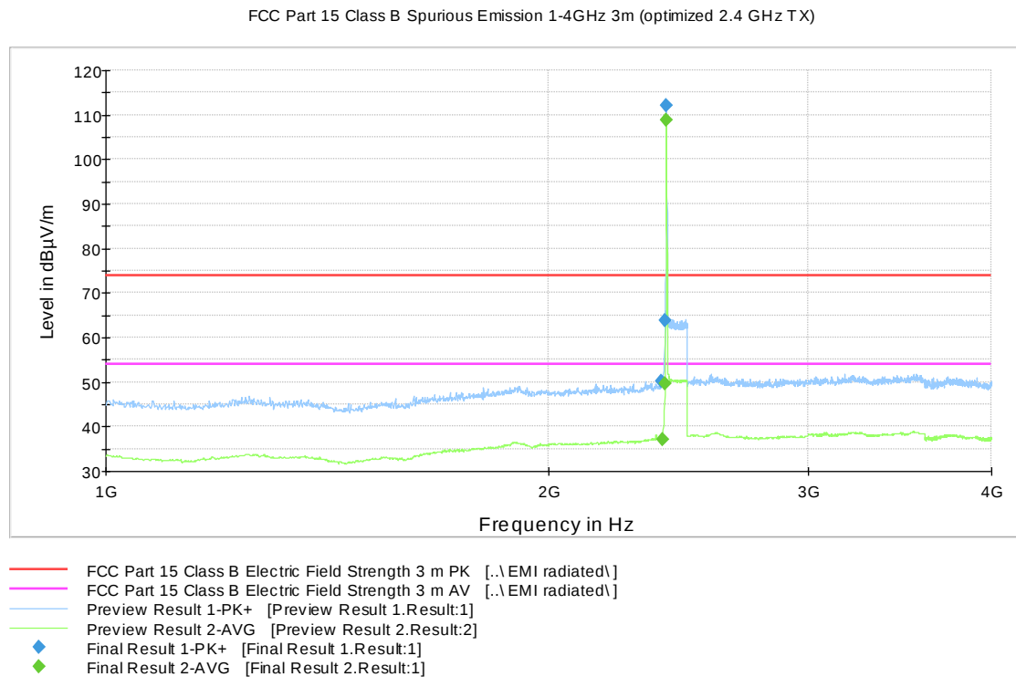
Figure 2: Channel 11 low 1 GHz – 4 GHz
