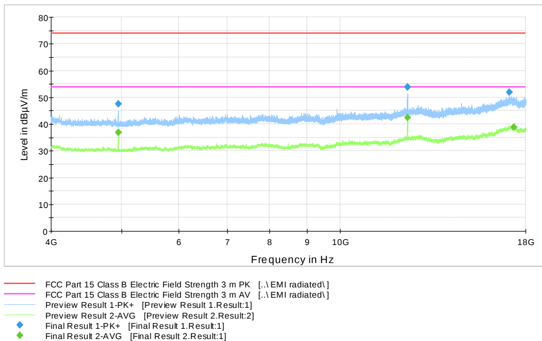
Figure 12: Channel 25 high 4 GHz – 18 GHz
