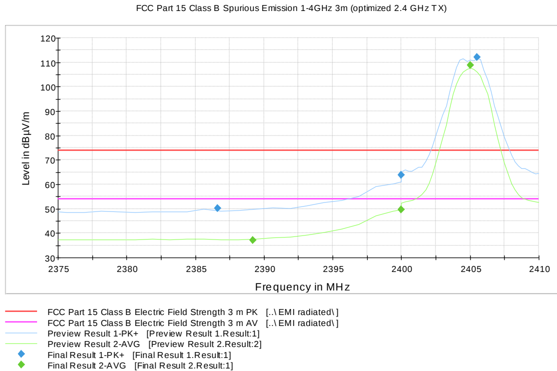
Figure 14: Radiated Band Edge measurement graph, Channel 11 low
