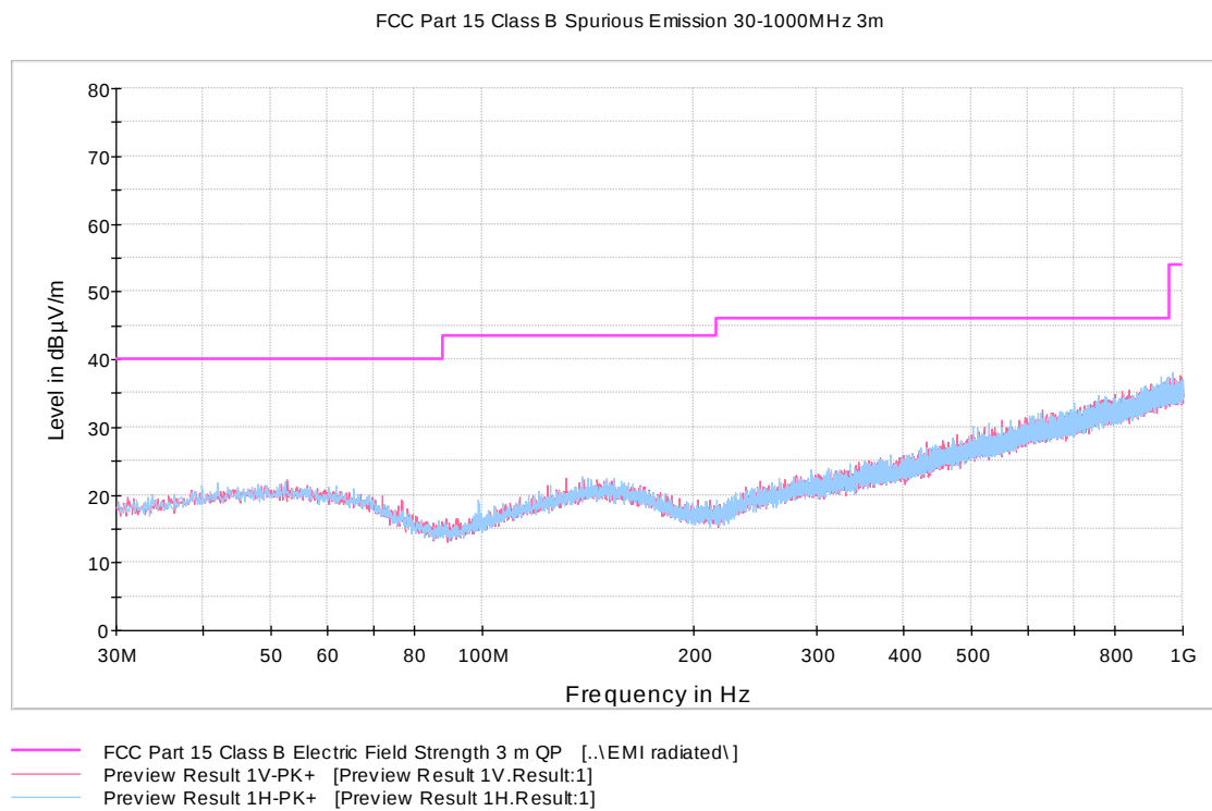
Figure 10: Channel 25 high 30 MHz – 1000 MHz
