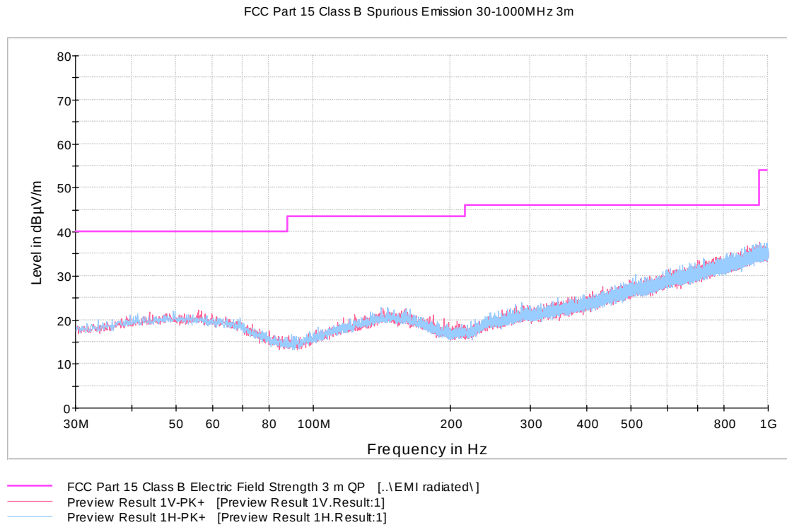
Figure 1: Channel 11 low 30 MHz – 1000 MHz
