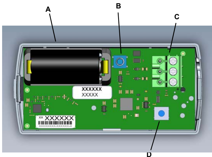
Figure 1 EN1550EP Components
