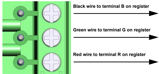
Figure 2 Connect the transmitter to the Neptune E-CODER register
