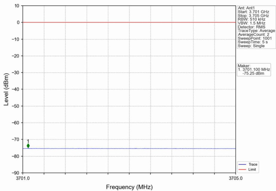
n48_30kHz_SISO_NTNV_40MHz_CP-OFDM QPSK_3624.99MHz_Edge_1RB_Left
