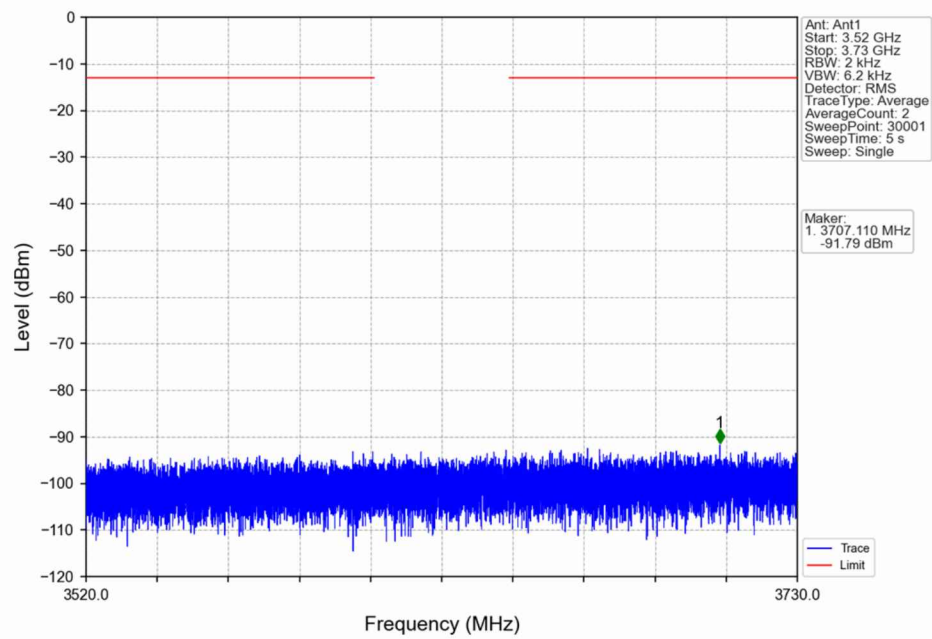
n48_30kHz_SISO_NTNV_40MHz_CP-OFDM QPSK_3624.99MHz_Edge_1RB_Left
