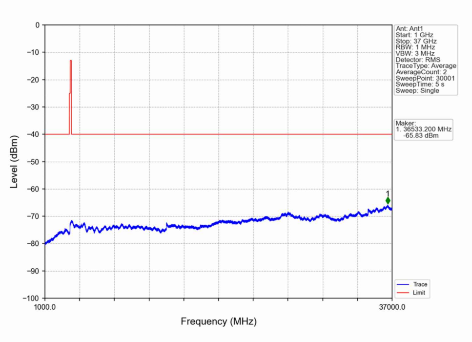
n48_30kHz_SISO_NTNV_40MHz_CP-OFDM QPSK_3679.98MHz_Outer_Full
