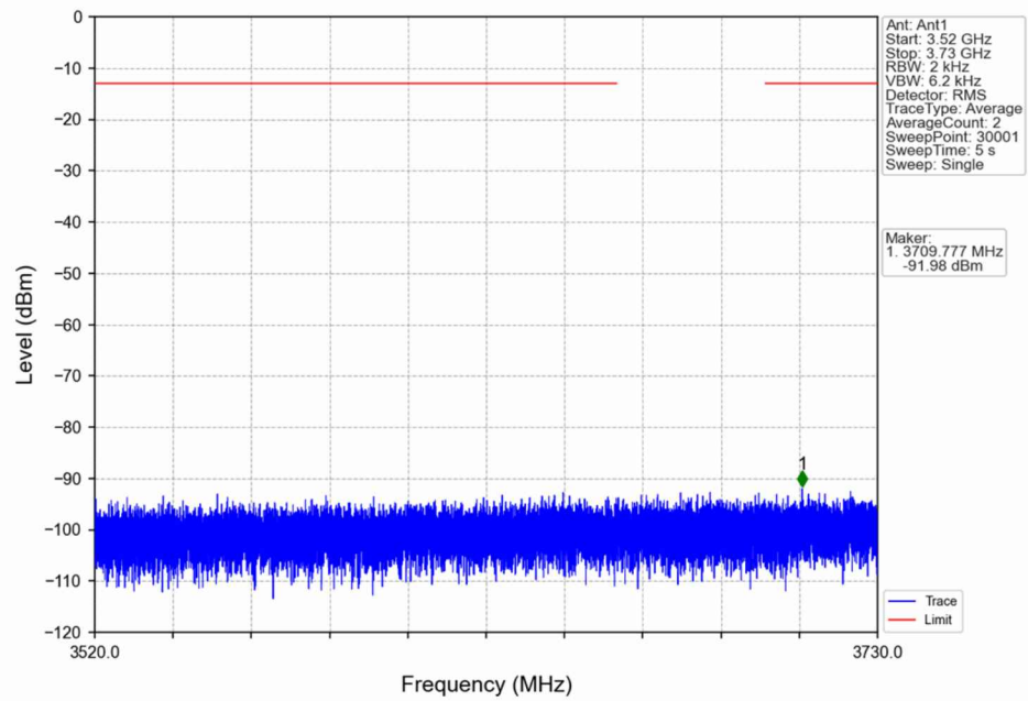
n48_30kHz_SISO_NTNV_40MHz_CP-OFDM QPSK_3679.98MHz_Inner_1RB_Right
