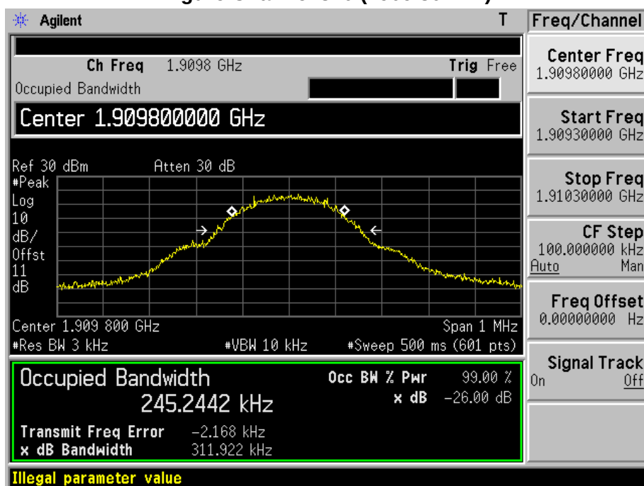
Figure Channel 810 (1909.80MHz)
