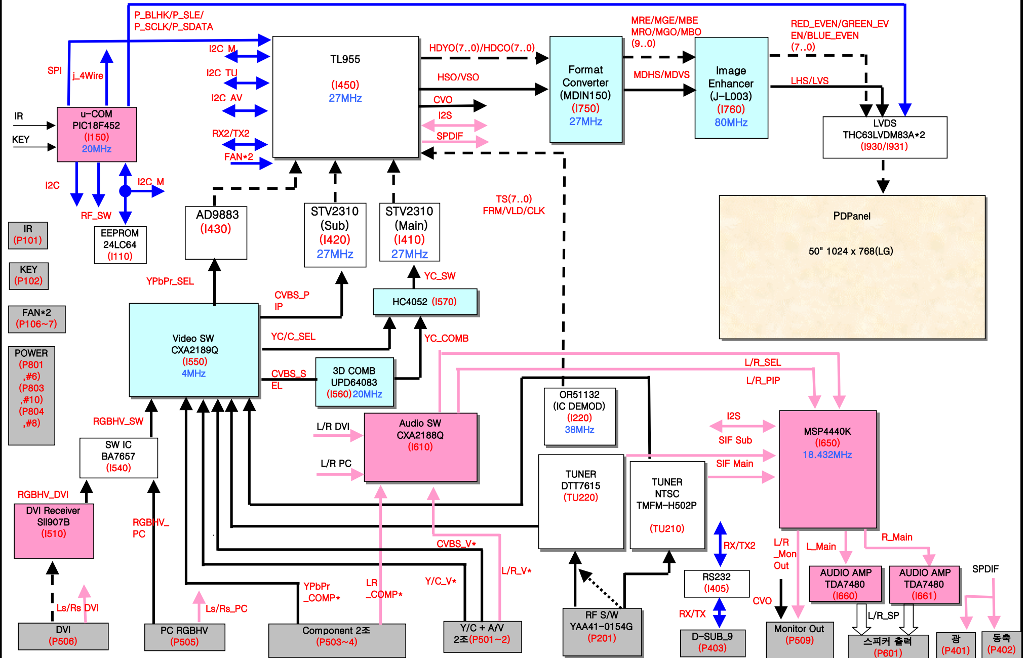
DPA-5034LDS BlockDiagram
