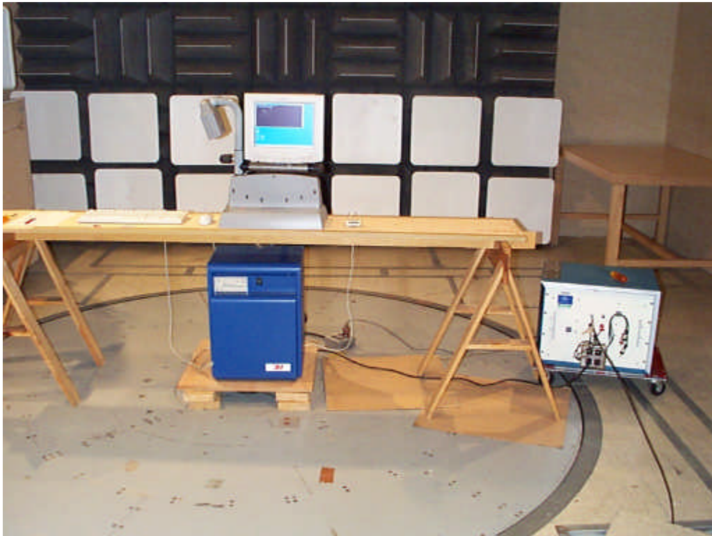
Conducted Emissions
