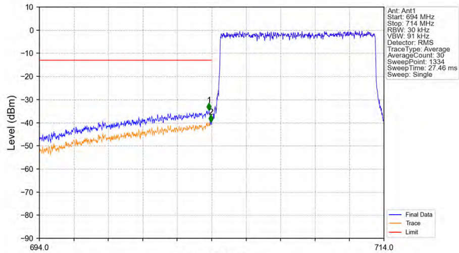
Band17_10MHz_16QAM_LCH_709MHz_RB_50_0_NTNV
