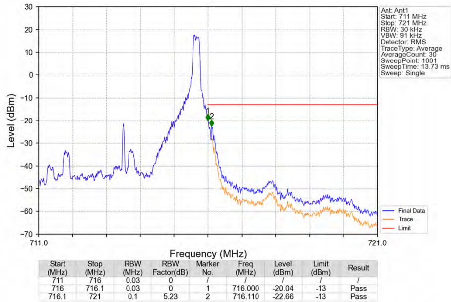
Band17_5MHz_QPSK_HCH_713.5MHz_RB_1_24_NTNV
