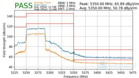
Plot 7-617. SDM (Pk & Avg, RU484, Index 65, Ch.54, MCS11)
