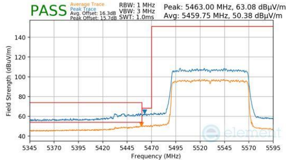
Plot 7-636. CDD (Pk & Avg, RU996, Index 67, Ch.106, MCS11)
