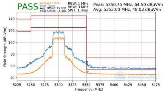
Plot 7-601. SDM (Pk & Avg, RU242, Index 61, Ch.60, MCS11)
