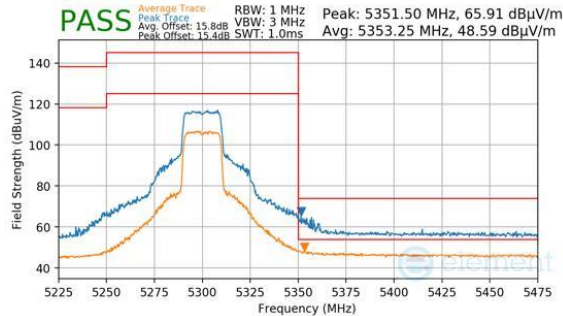
Plot 7-543. Antenna WF2 (Pk & Avg, RU242, Index 61, Ch.60, MCS11)
