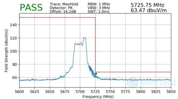
Plot 7-596. SDM (Pk, RU52, Index 40, Ch.140, MCS11)
