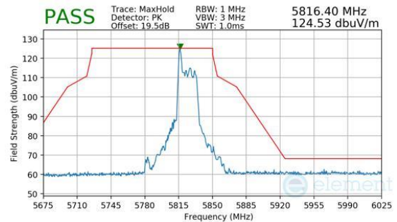
Plot 7-598. CDD (Pk, RU26, Index 0, Ch.165, MCS11)
