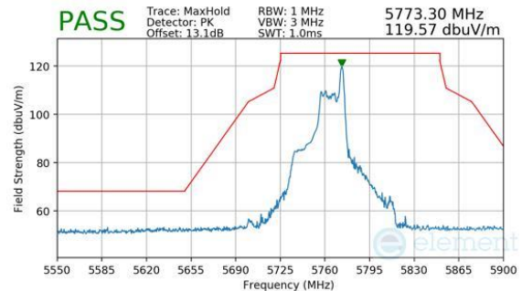
Plot 7-613. CDD (Pk, RU26, Index 17, Ch.151, MCS11)
