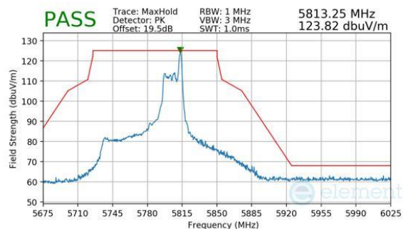
Plot 7-633. CDD (Pk, RU26, Index 36, Ch.155, MCS11)
