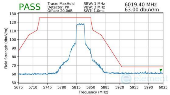
Plot 7-608. CDD (Pk, RU242, Index 61, Ch.165, MCS11)
