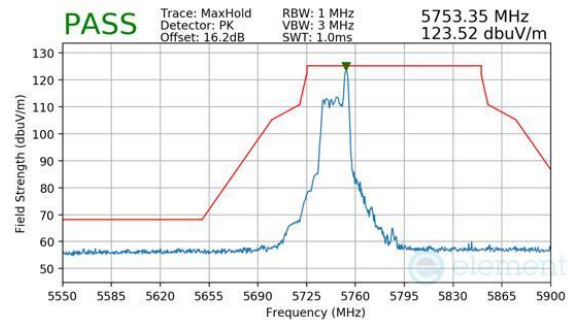
Plot 7-539. Antenna WF2 (Pk, RU26, Index 8, Ch.149, MCS11)
