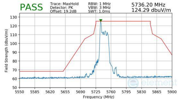
Plot 7-597. CDD (Pk, RU26, Index 0, Ch.149, MCS11)
