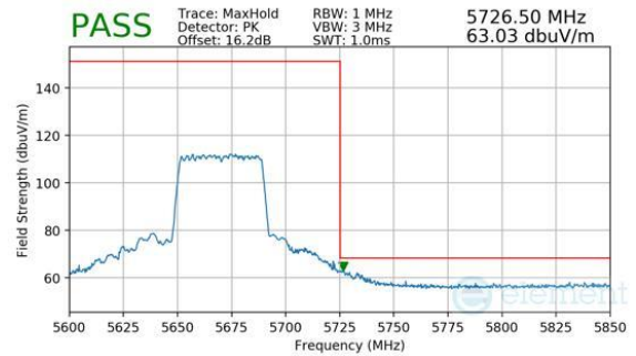
Plot 7-624. CDD (Pk, RU484, Index 65, Ch.134, MCS11)
