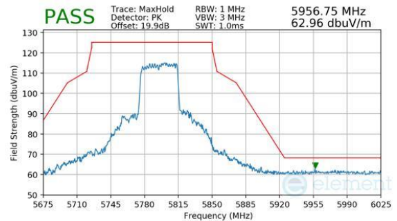
Plot 7-626. CDD (Pk, RU484, Index 65, Ch.159, MCS11)
