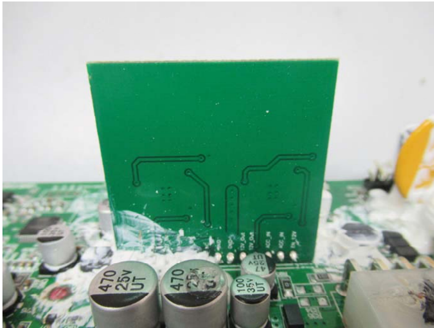
EUT – PCB-4 Chip View-2
